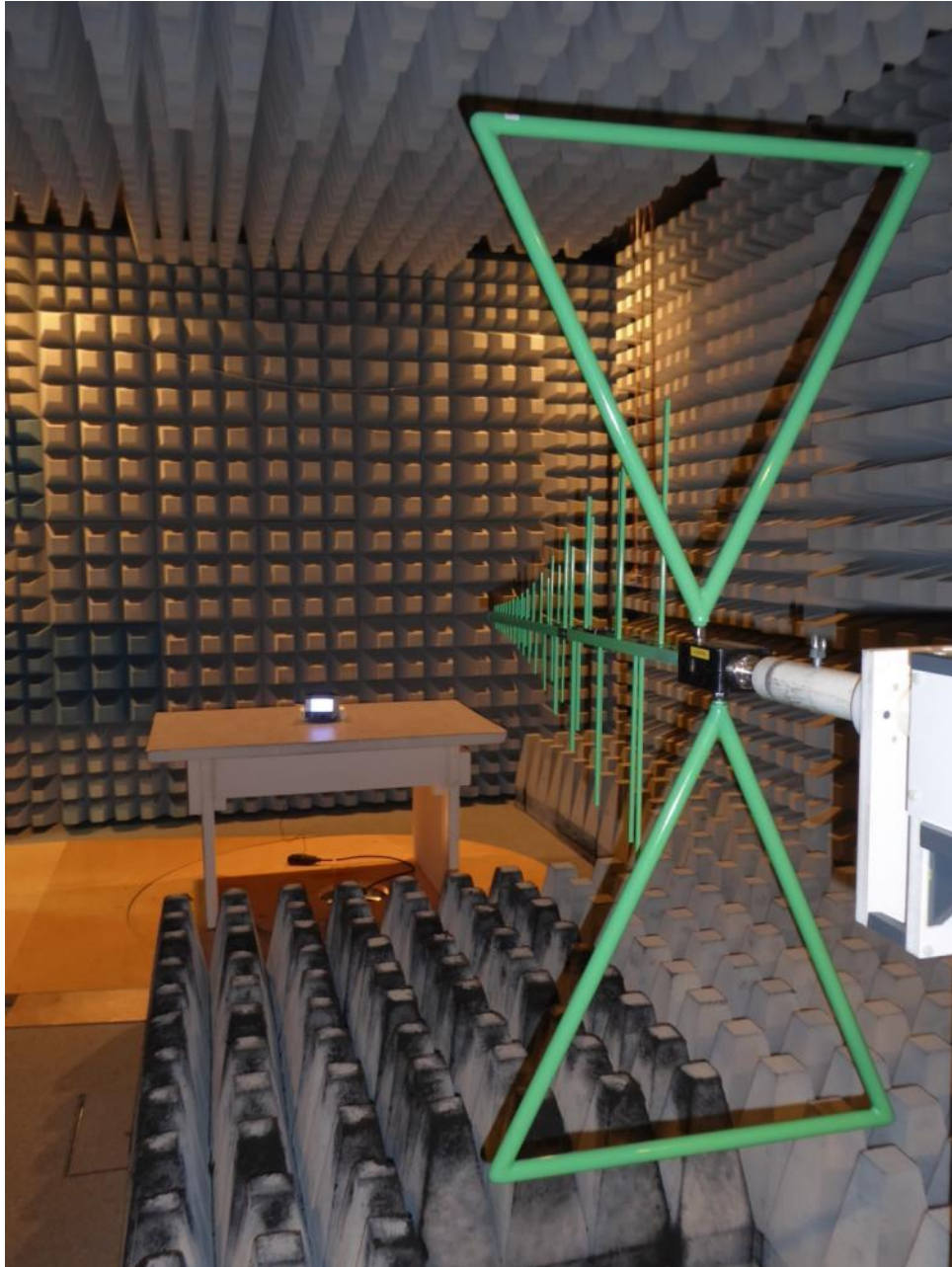
170756_F2.JPG: Test setup fully anechoic chamber
