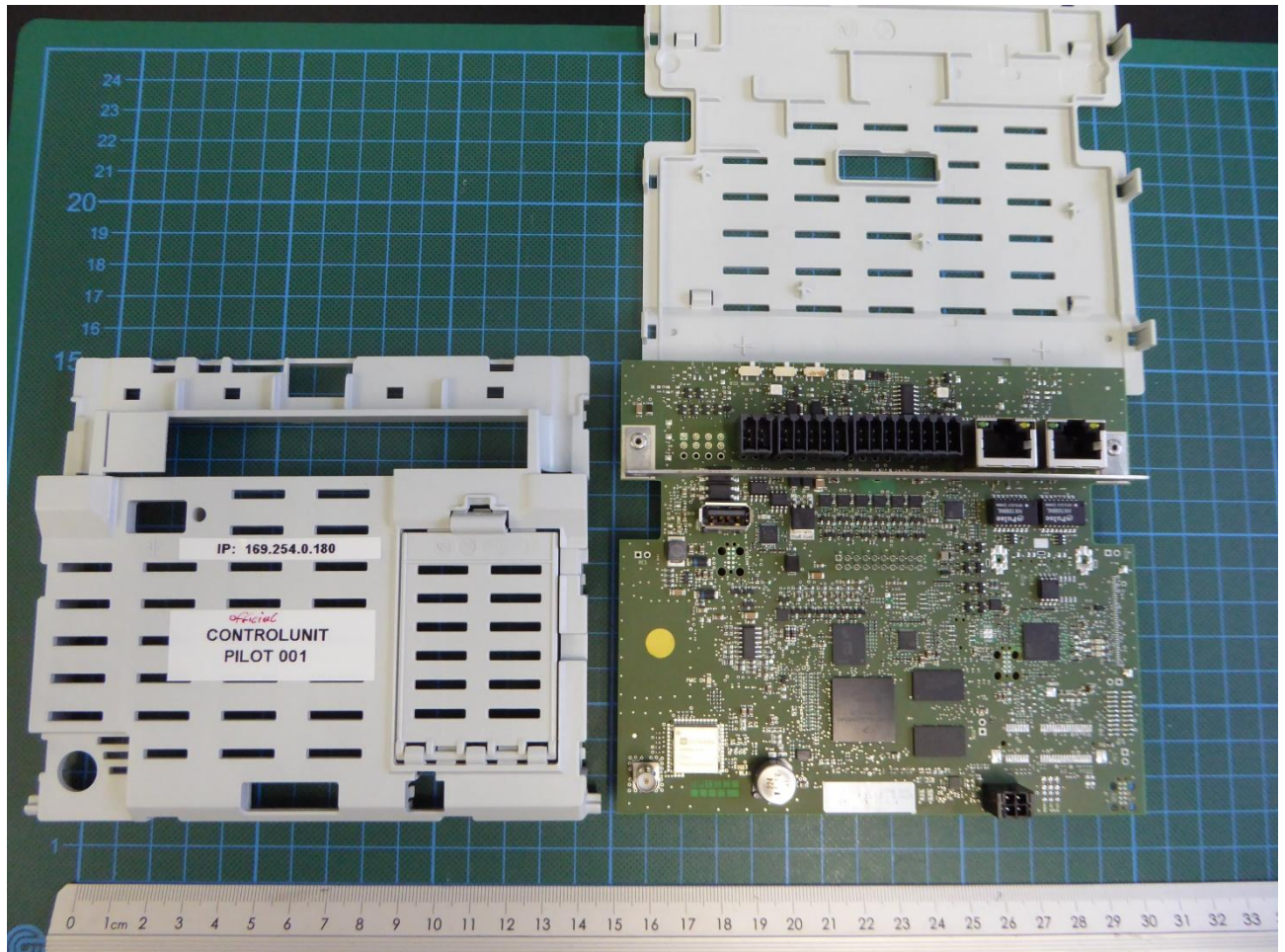
EUT opened front view
