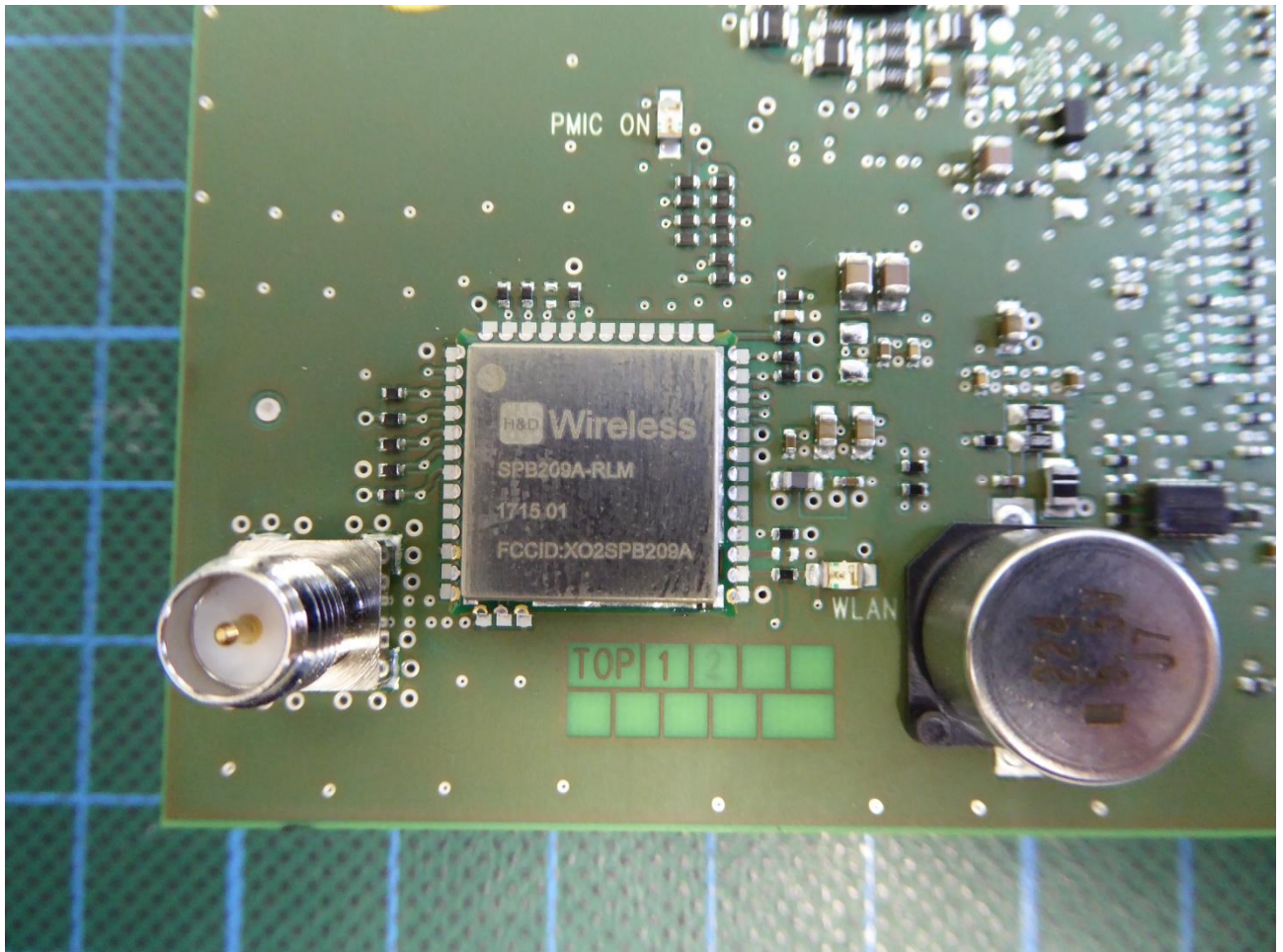
EUT radio module Detail view
