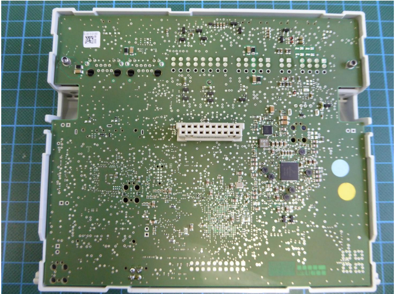
EUT PCB rear view
