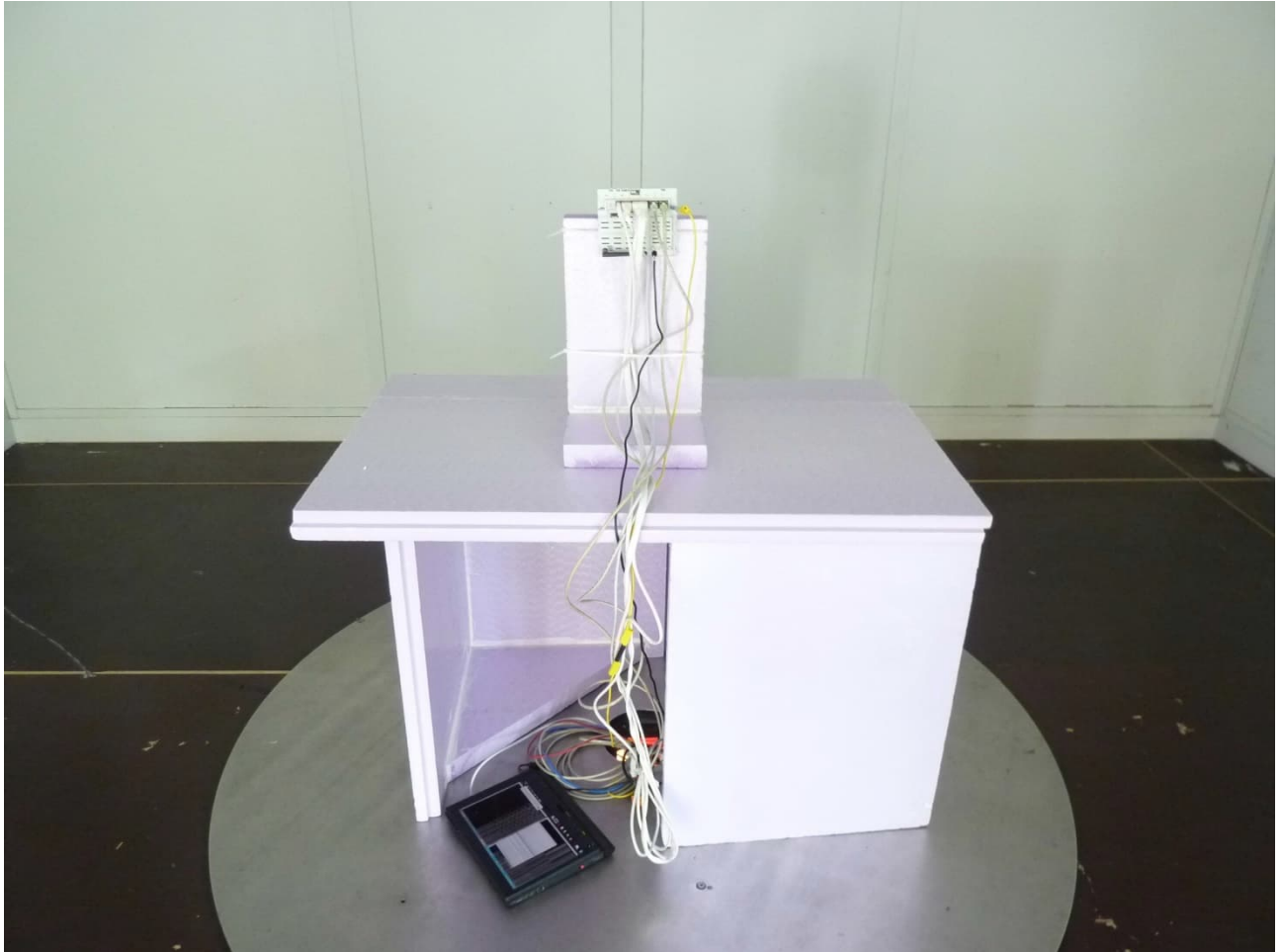
Test setup OATS Final measurement 30 MHz – 1 GHz
