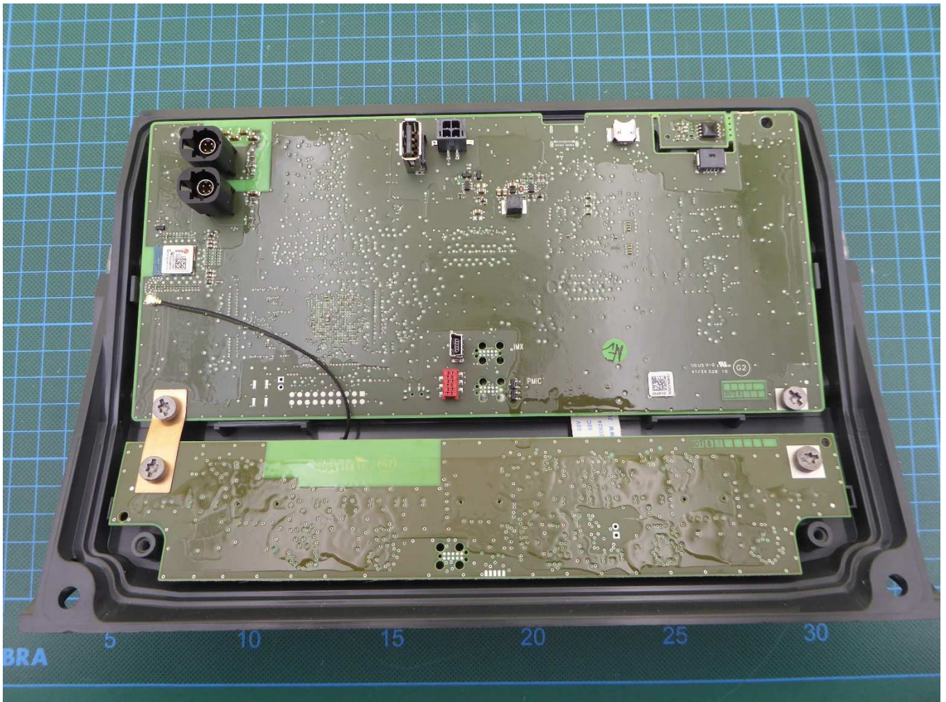
EUT Opened
