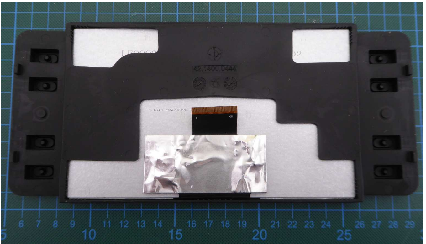
Display – top view
