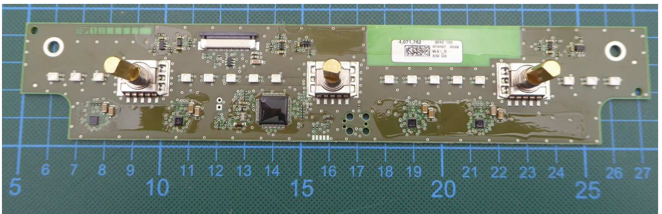
MMI PCB – bottom view
