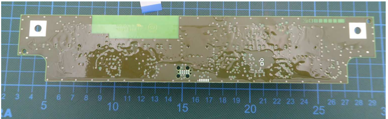
MMI PCB – top view
