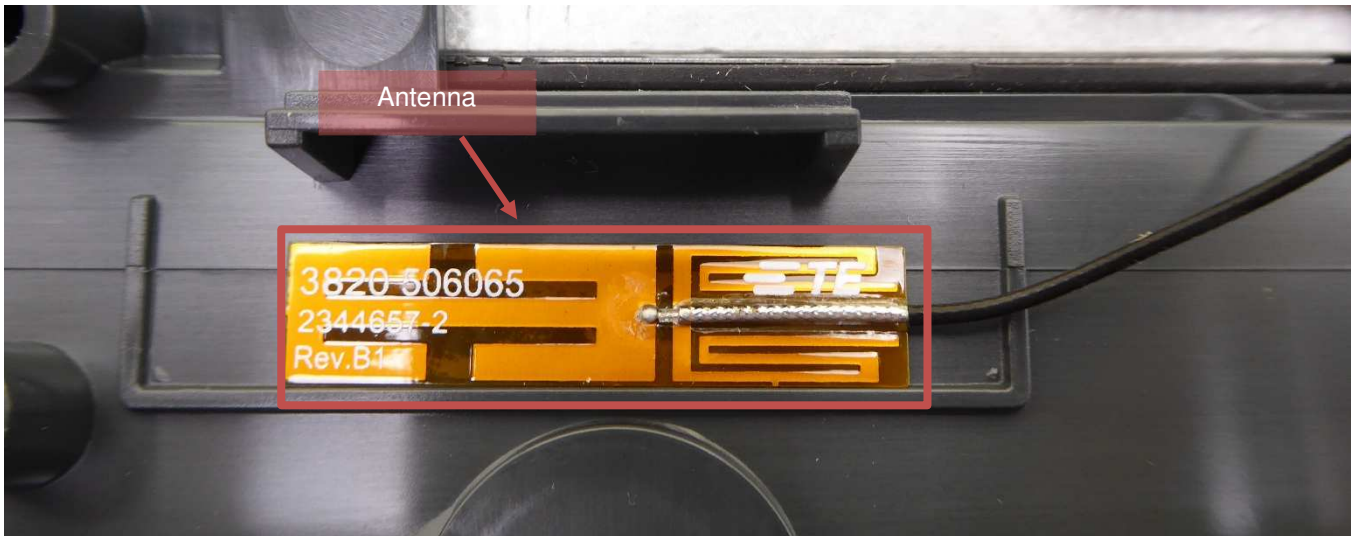
Antenna – detail view
