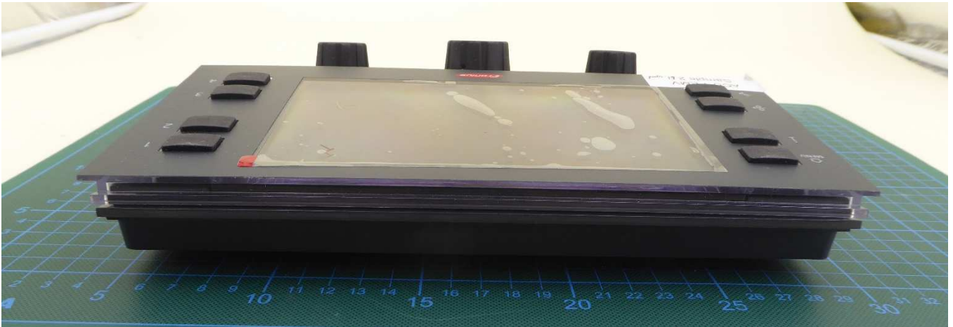
EUT Side view 4
