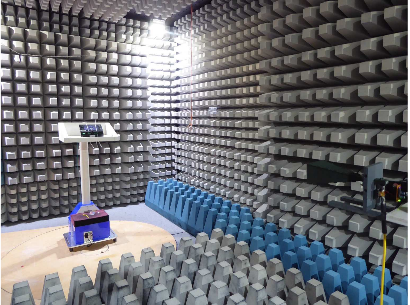
Test setup fully anechoic chamber TX 12.75 GHz - 18 GHz
