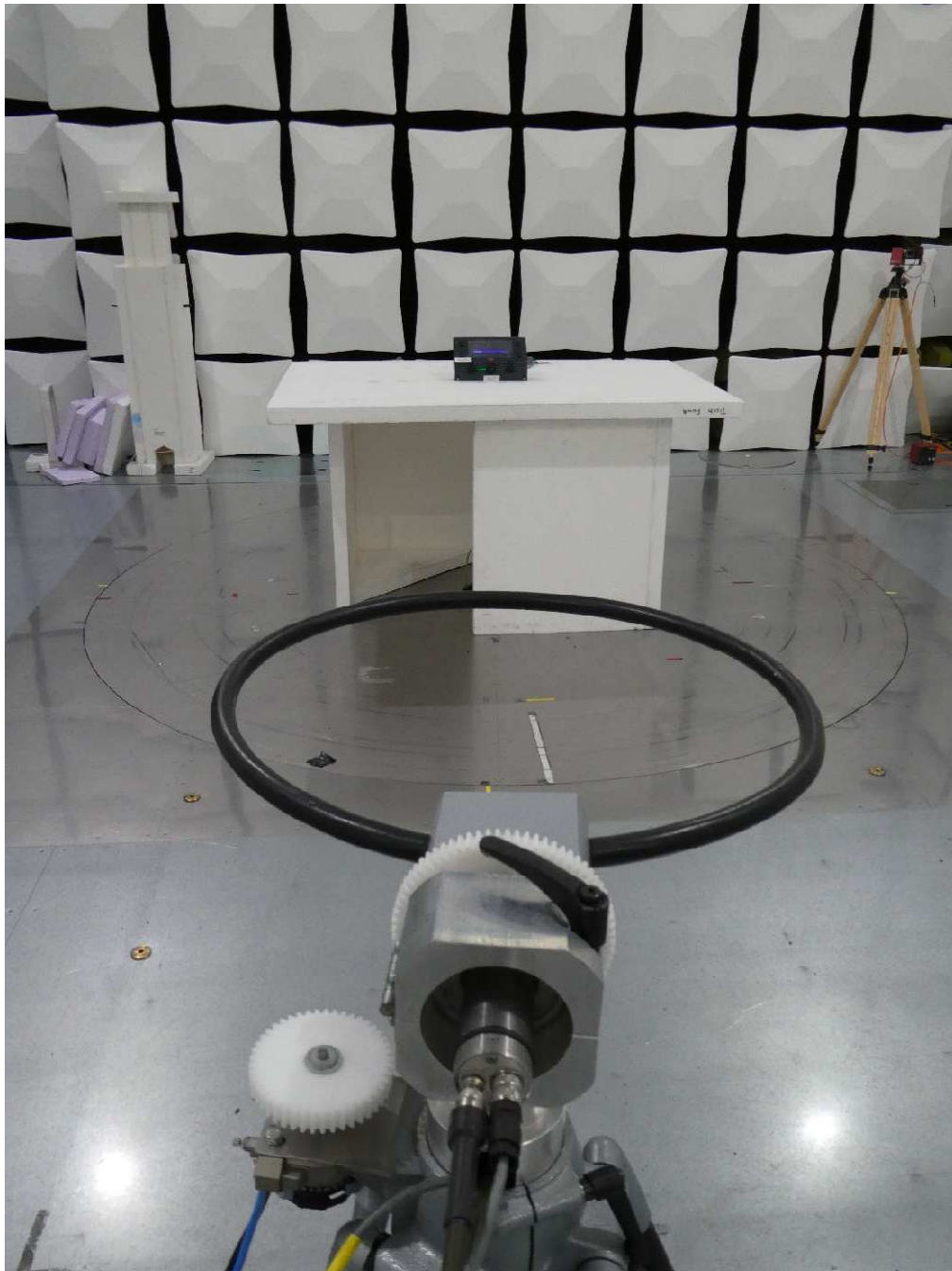
Test setup semi anechoic chamber TX 9 kHz – 30 MHz – 3
