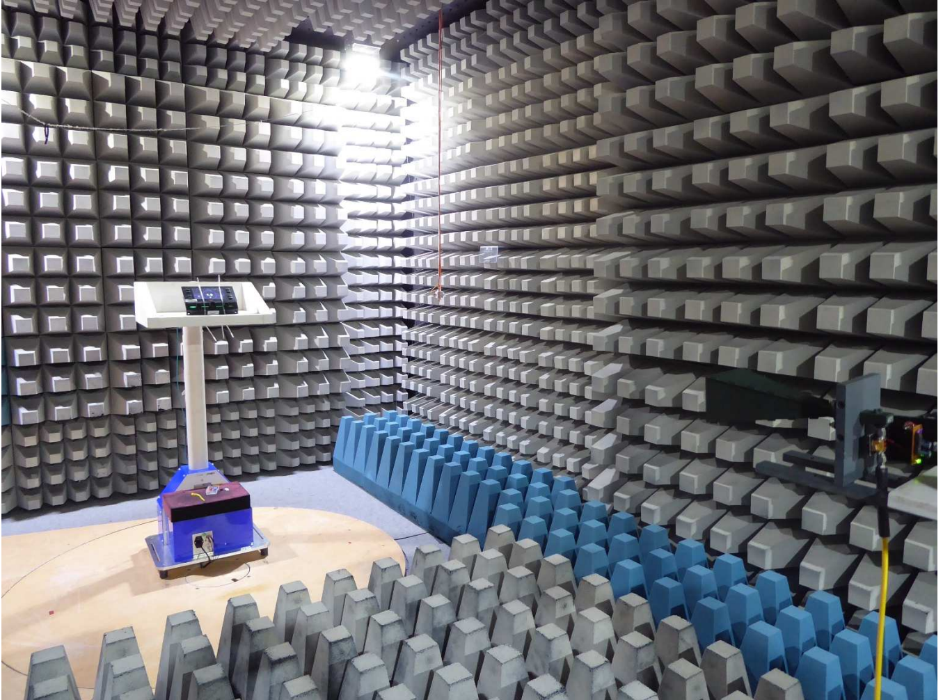
Test setup fully anechoic chamber TX 12 GHz - 18 GHz
