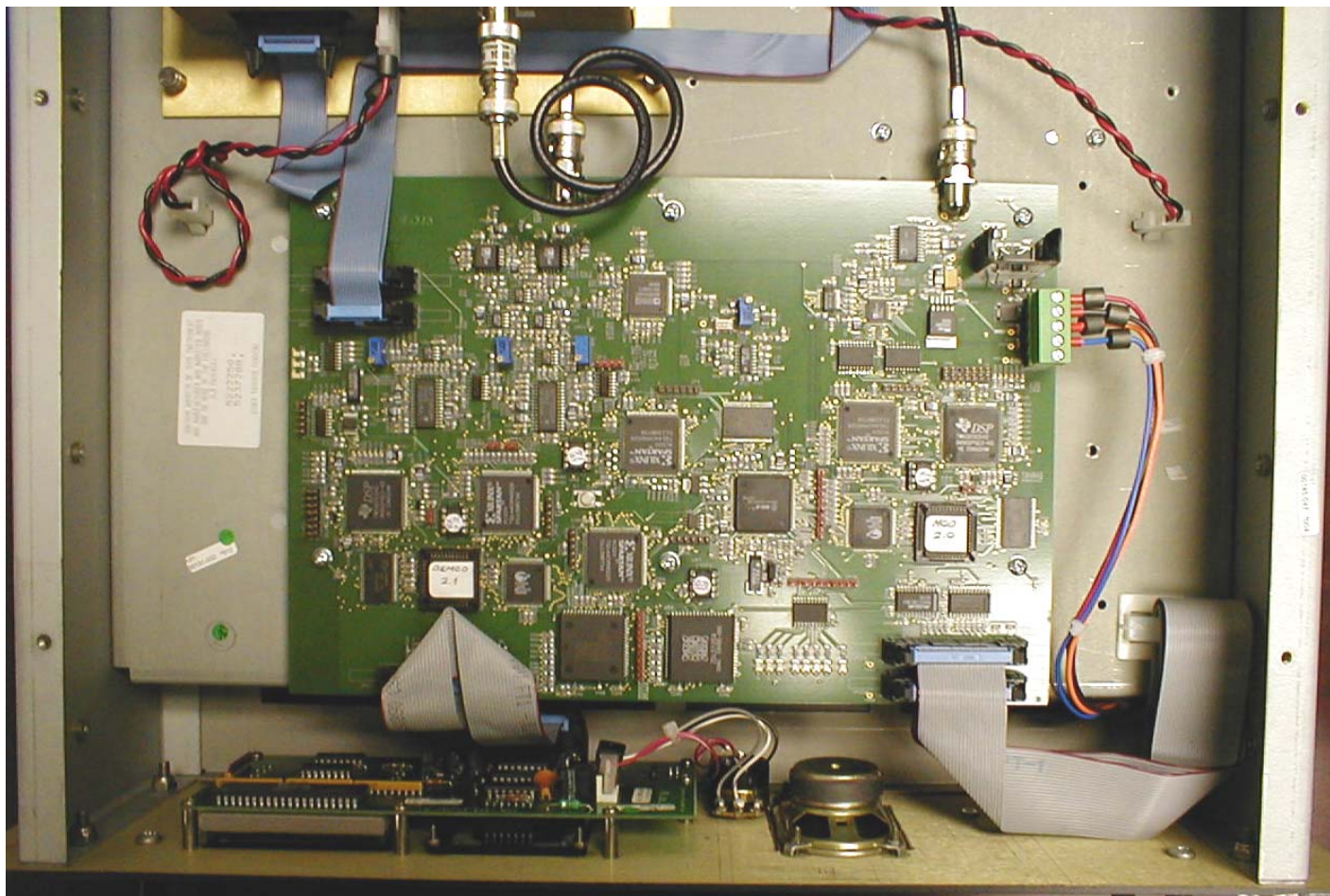
Figure 5.4 Internal Top View - CX2-1100R (Receiver/Control) Controller Board Detail
