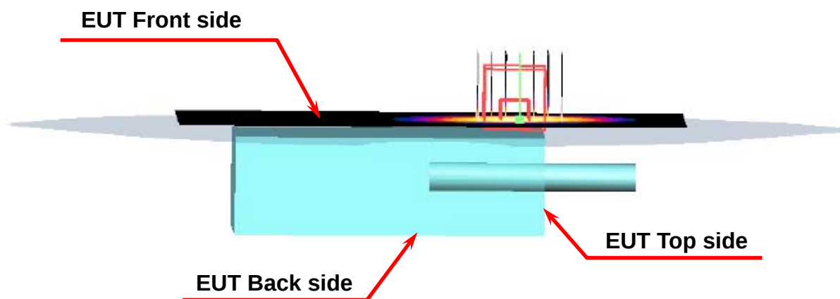
Figure 2. Brain SAR Test Setup (Flat Section)
