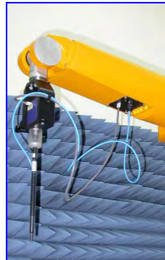
Figure 3. Probe setup on robot
