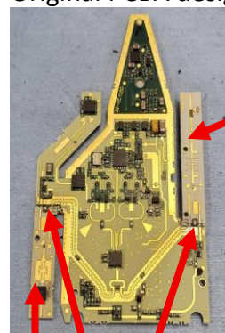
Original PCBA design
