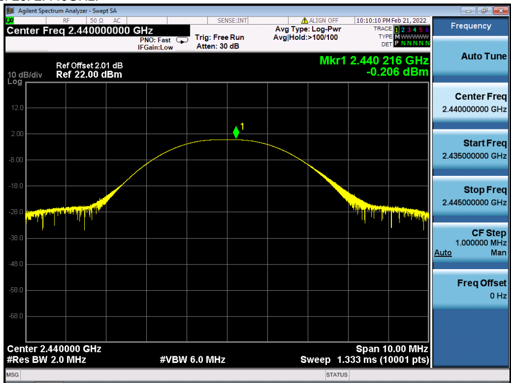
Channel 20: 2.440GHz:
