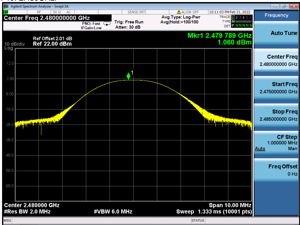
Channel 40: 2.480GHz:
