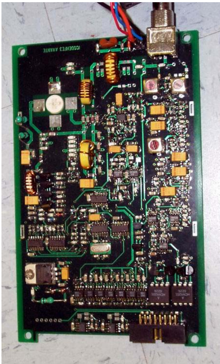
Component Side/PCB1
