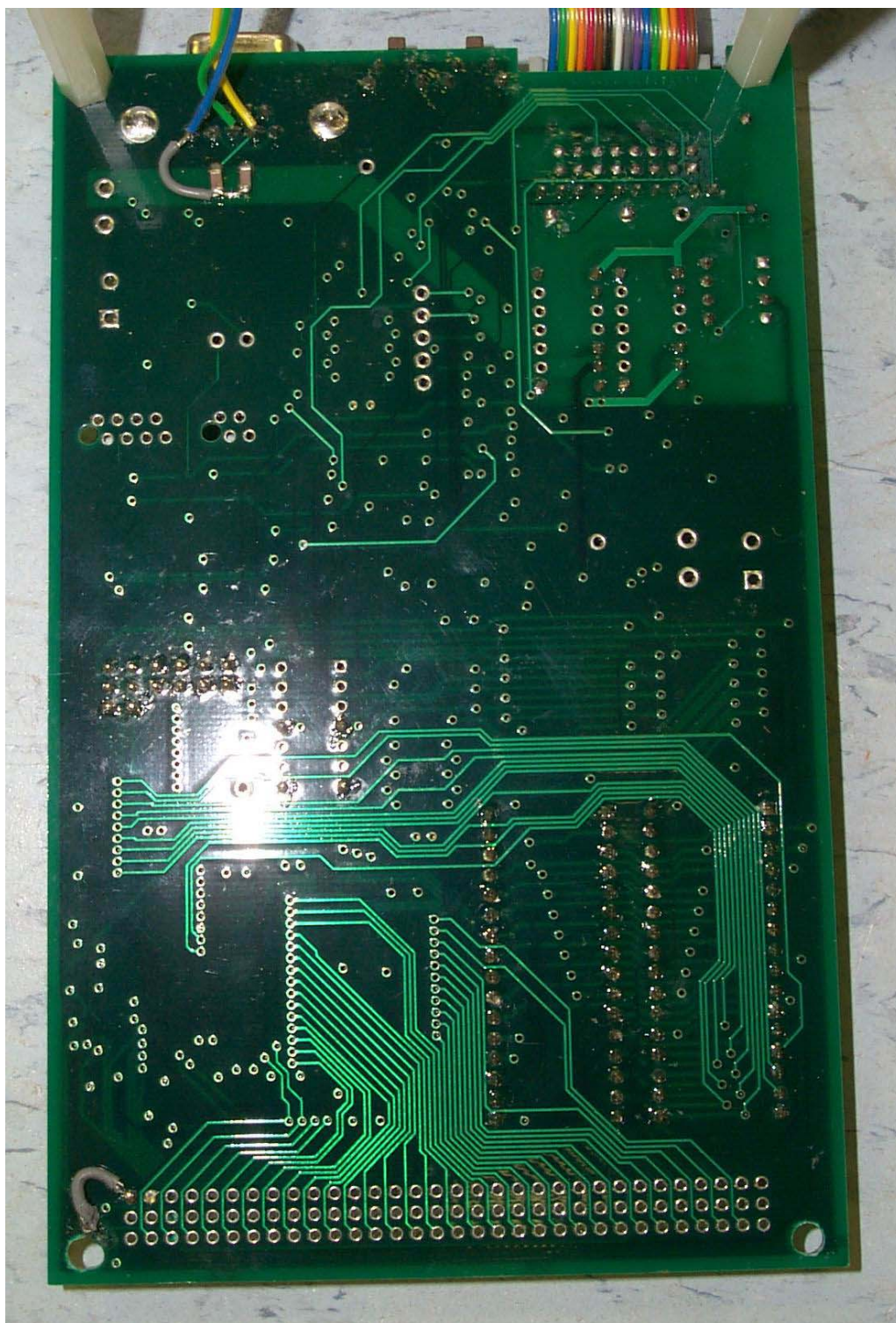
Foil Side/PCB2
