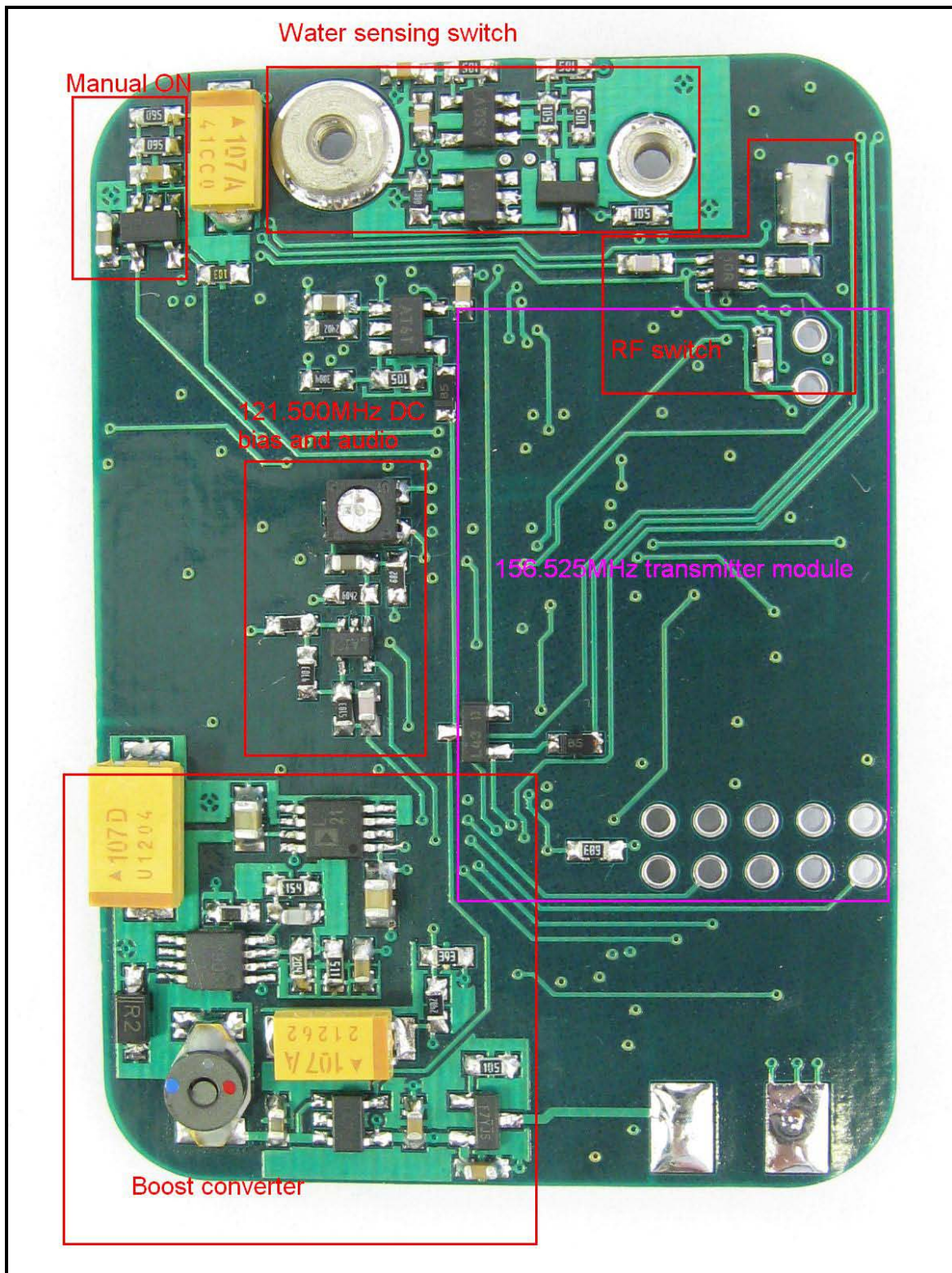
Photograph 7: Main PCB - Bottom
