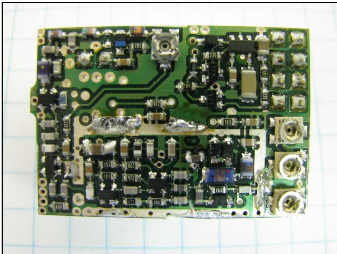
Photograph 11: DSC Transmitter – Bottom (with smaller shield removed)
