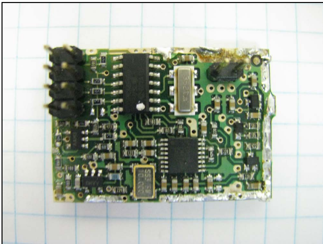
Photograph 9: DSC Transmitter with Shield Removed - Top
