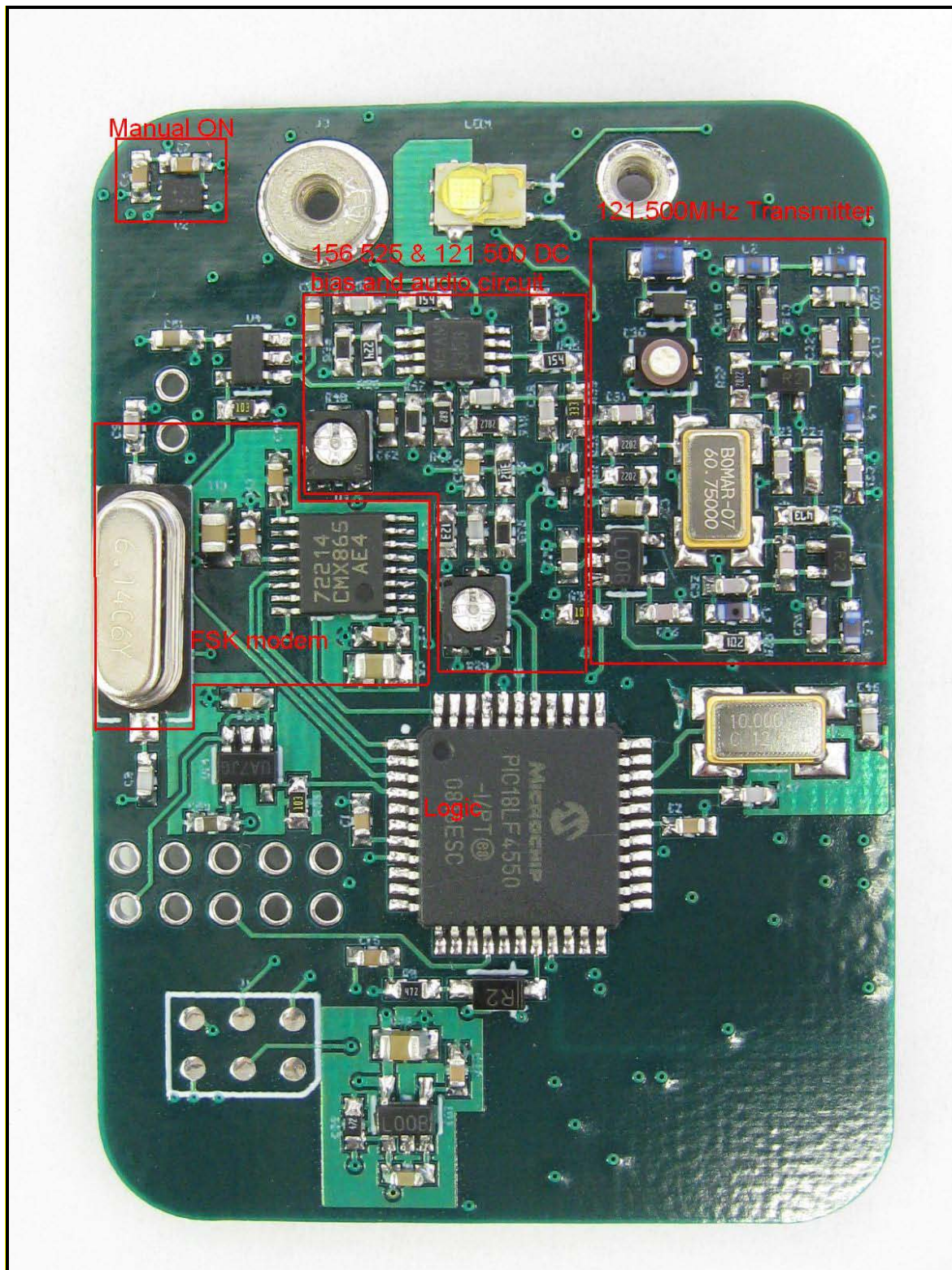
Photograph 6: Main PCB - Top
