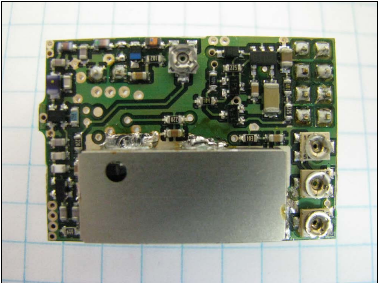
Photograph 10: DSC Transmitter – Bottom (with smaller shield)
