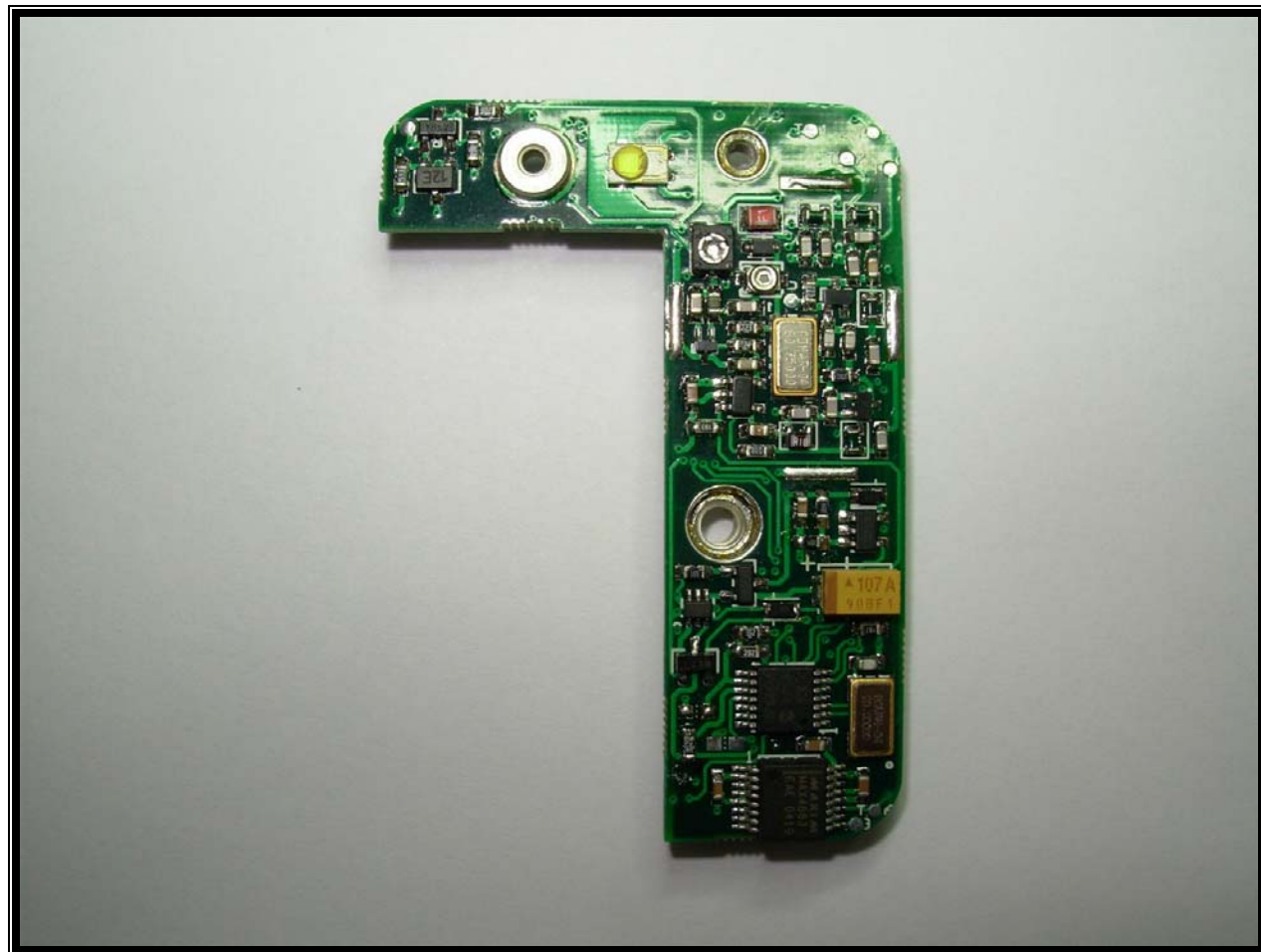
Photograph 6: PCB Top without Shield
