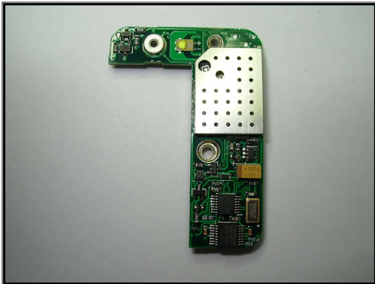
Photograph 5: PCB Top with Shield
