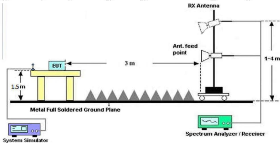
Figure 3. Above 1 GHz
