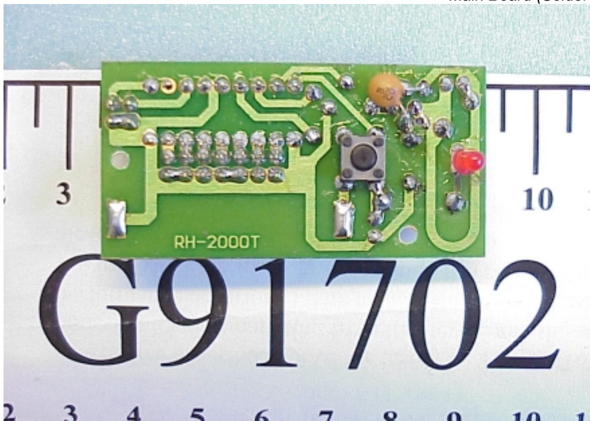
Photos 6 Main Board (Solder Side)
