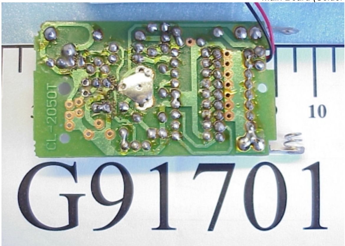
Photos 4 Main Board (Solder Side)
