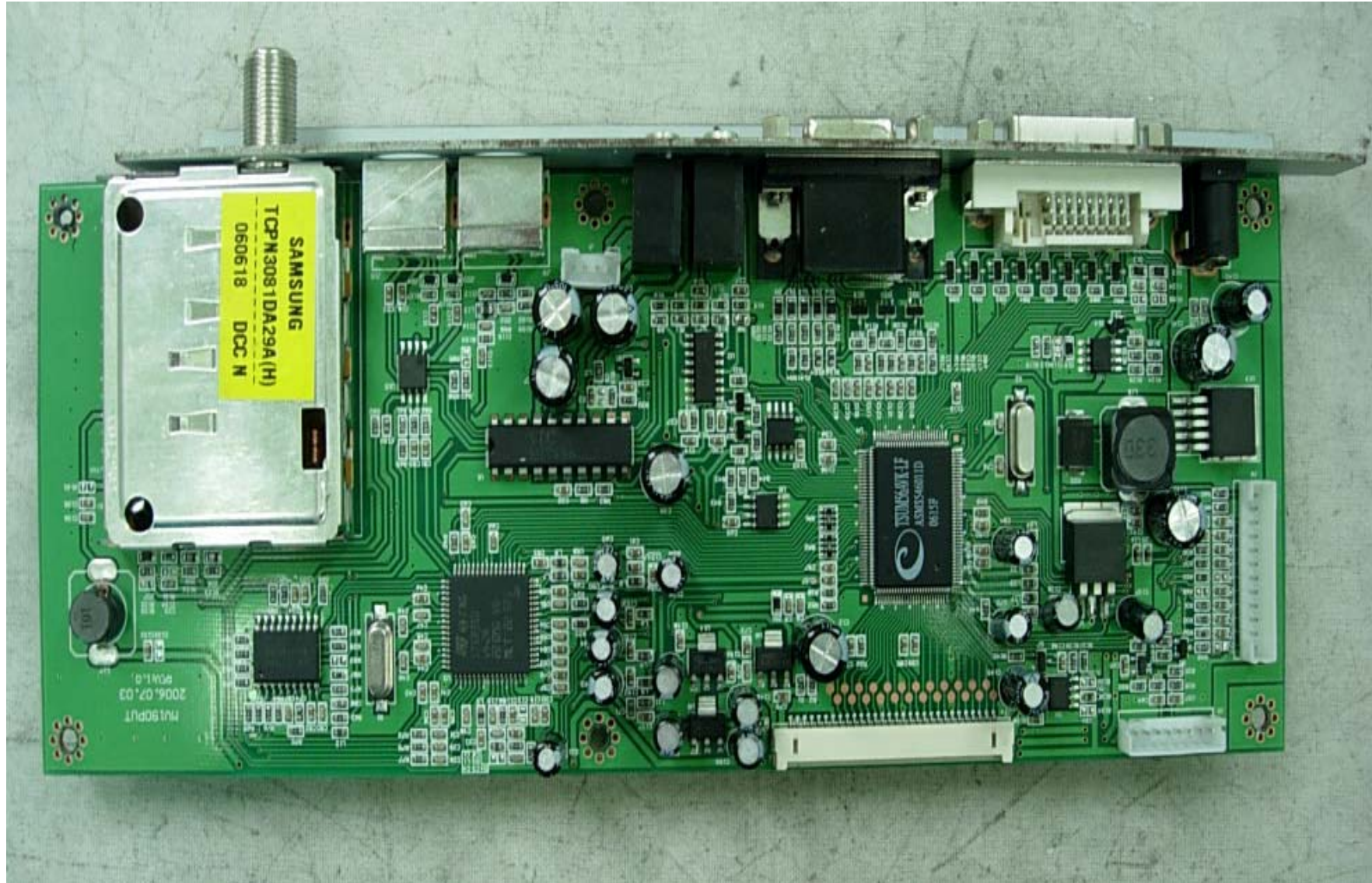
AD Board(Front)
