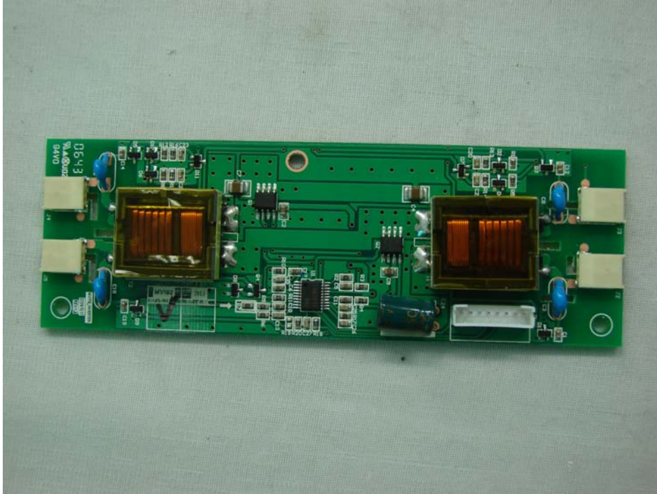
Inverter (Rear)
