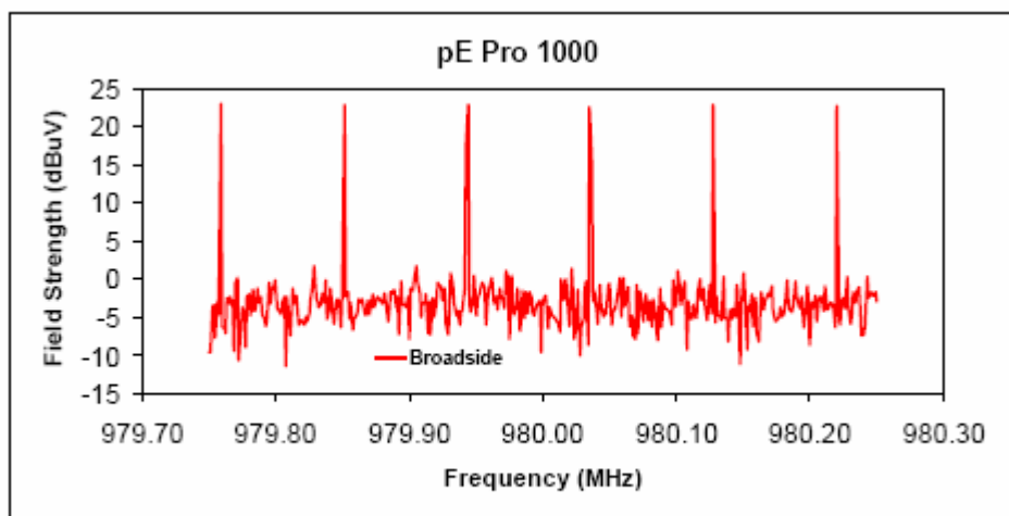
Plot 1: Pulse Repetition Frequency measurement
