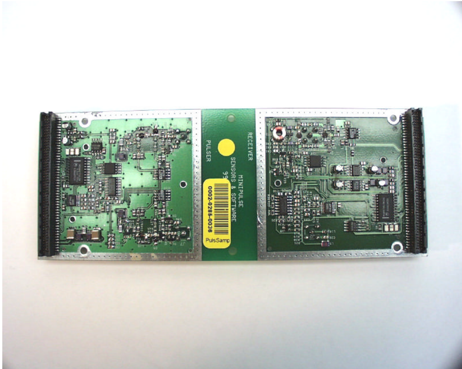
Radio Printed Circuit Board with Shield Cover opened
