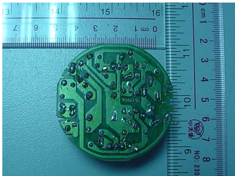
Figure 4 M/N: ETU-SS-11/15/20/24W Main Board, Cu Foil Side
