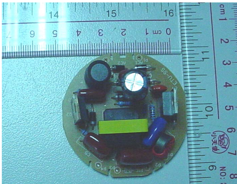
Figure 3 M/N: ETU-SS-11/15/20/24W Main Board, Component Side
