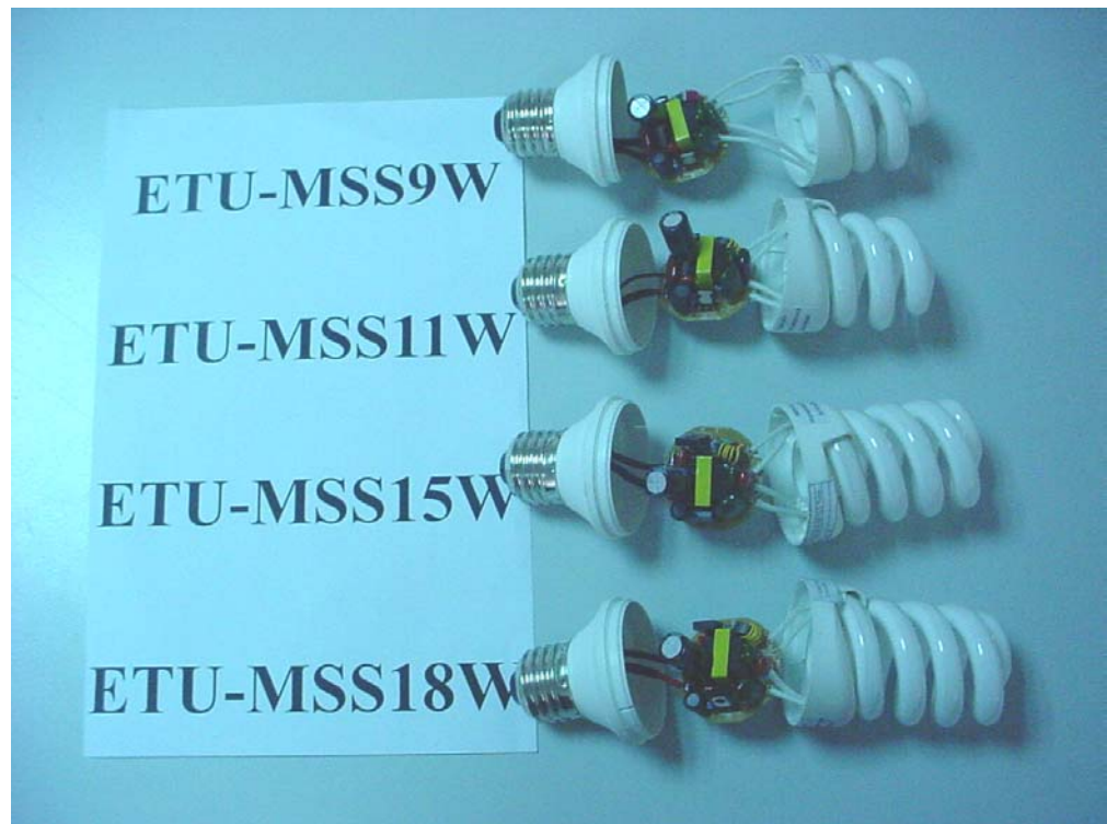
Figure 16 M/N: EBU-MSS-9/11/15/18W Internal Photographs
