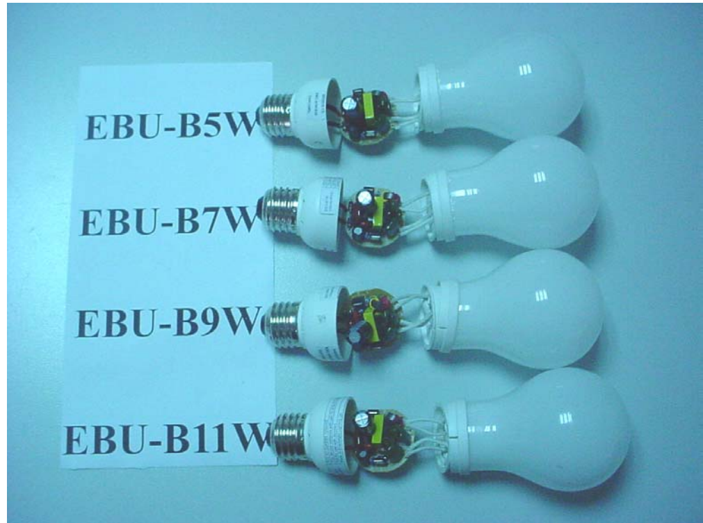
Figure 12 M/N: EBU-B-5/7/9/11W Internal Photographs
