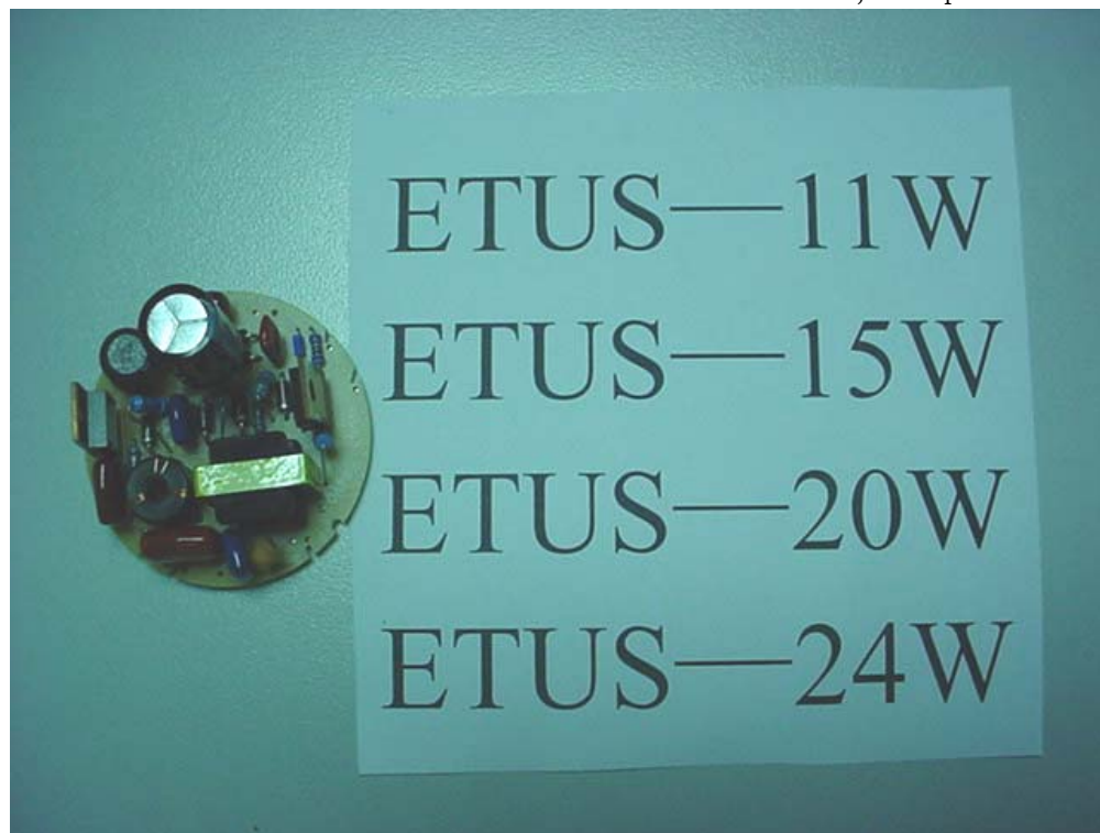
Figure 5 M/N: ETUS Series Main Board, Component Side
