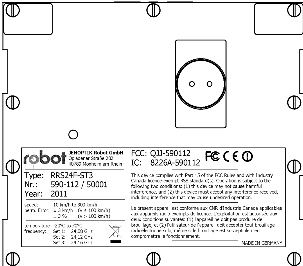
Label placement on rear of RRS24F-ST3
