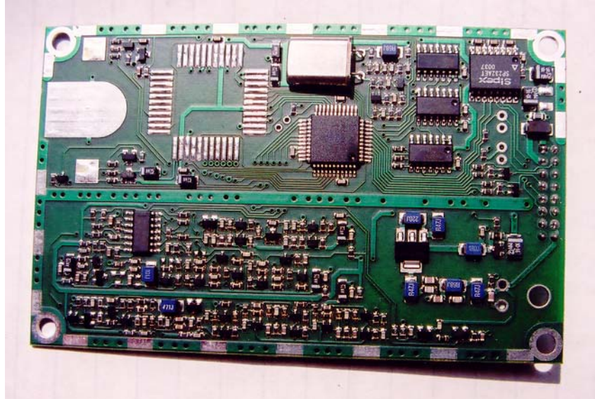
Component View
