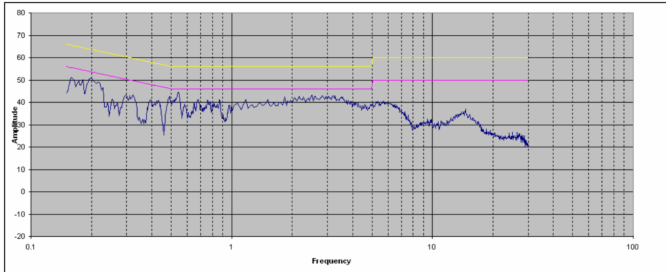
Conducted Emission Limits, Neutral Line Plot
