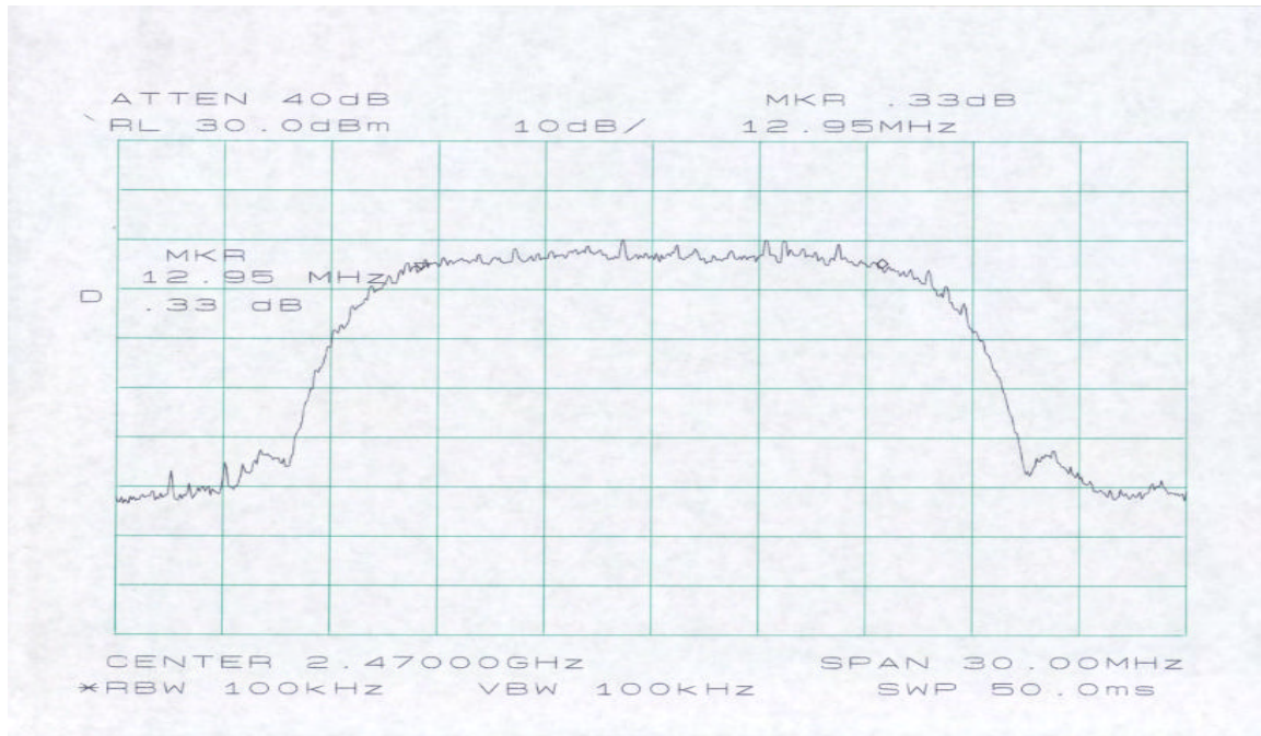
6 dB Bandwidth @ 2470 MHz (High channel)
