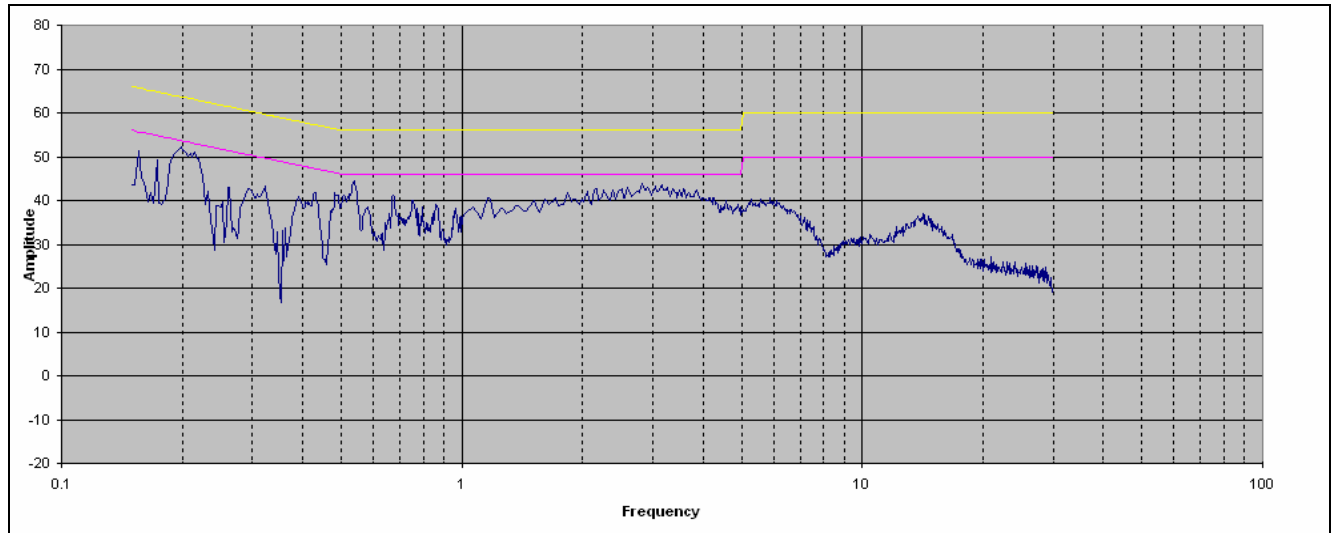
Conducted Emission Limits, Phase Line Plot
