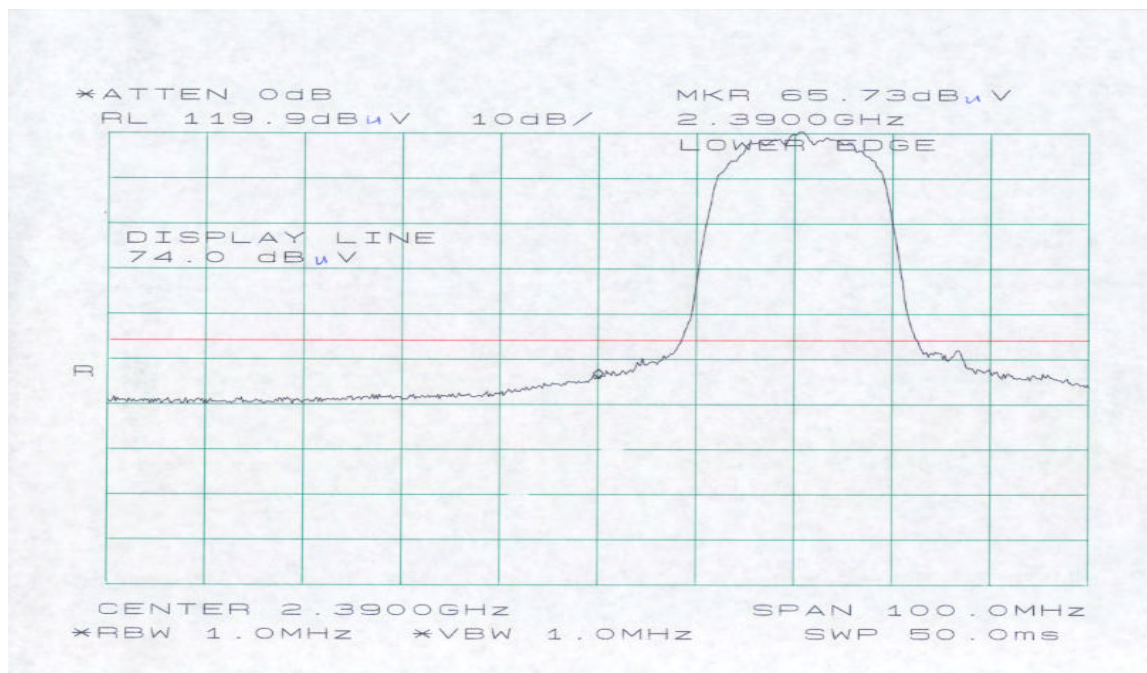
PEAK Limit at Lower Edge for 2410 MHz Plot
