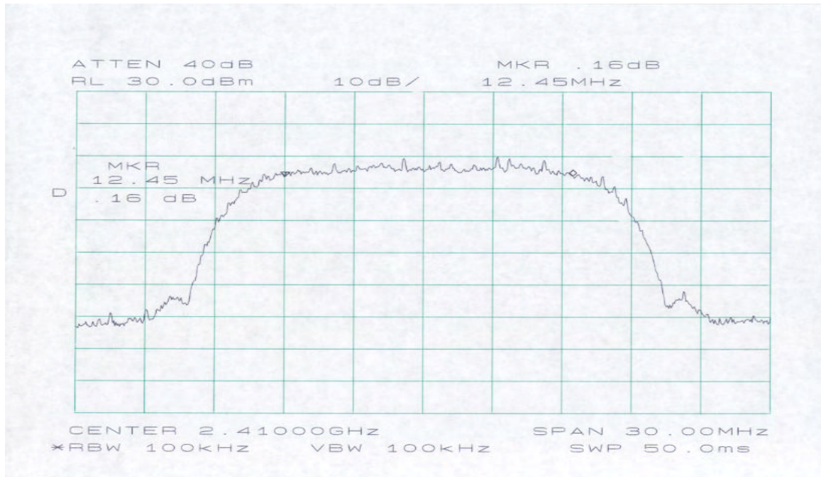
6 dB Bandwidth @ 2410 MHz (Low channel)
