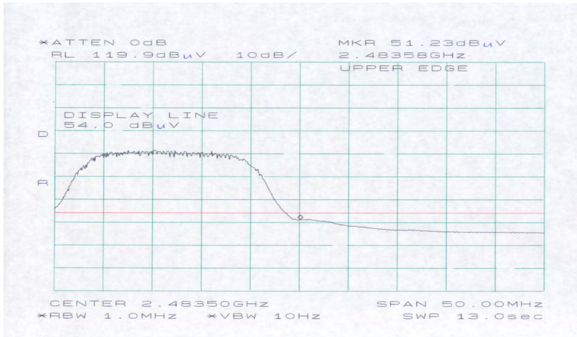
AVERAGE Limit at Upper Edge for 2470 MHz Plot
