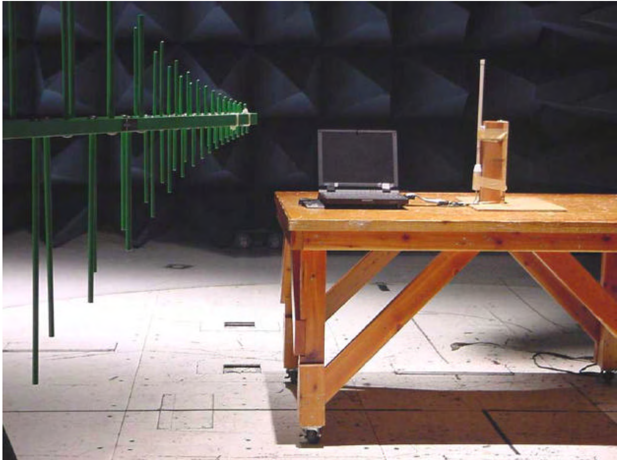
Photograph 2. Radiated Emission Limits (Below 1 GHz), Test Setup
