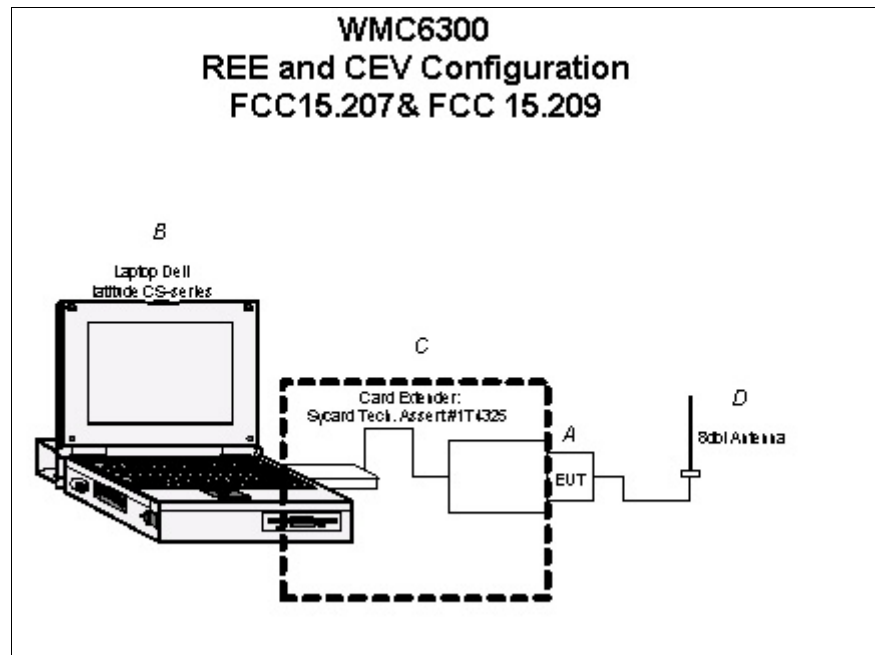
Figure 1. Block Diagram of Test Configuration (FCC 15.207 & FCC 15.209)
