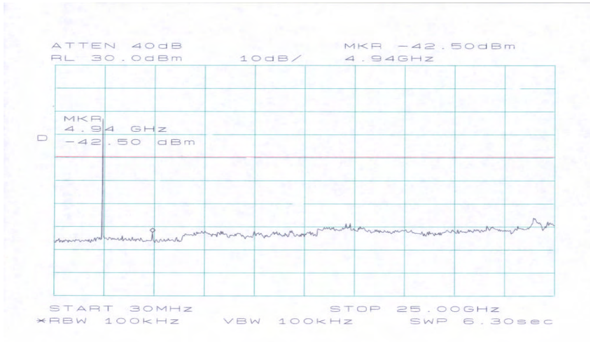
Conducted Spurious Emission for 2470 MHz (High channel)
