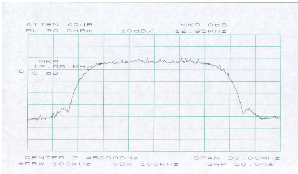
6 dB Bandwidth @ 2450 MHz (Mid channel)
