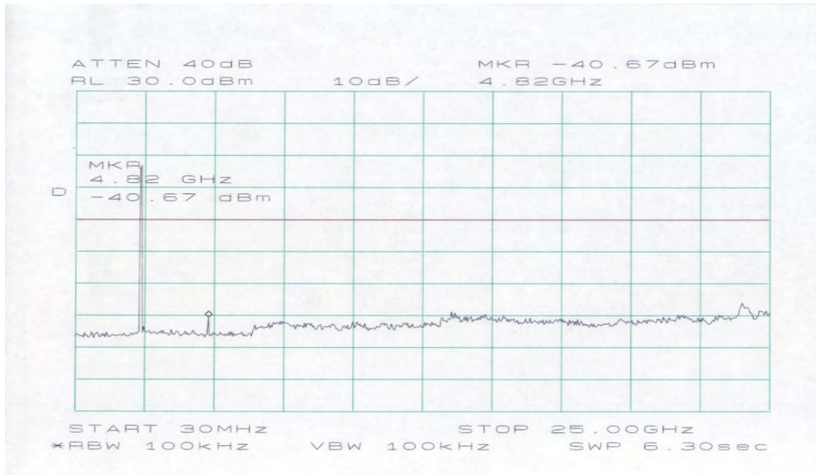
Conducted Spurious Emission for 2410 MHz (Low channel)
