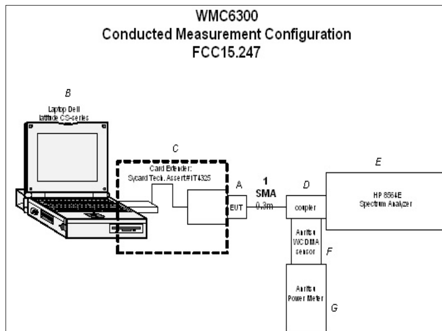
Figure 2. Block Diagram of Test Configuration (FCC 15.247)
