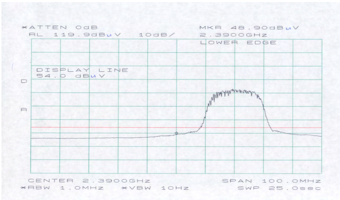
AVERAGE Limit at Lower Edge for 2410 MHz Plot
