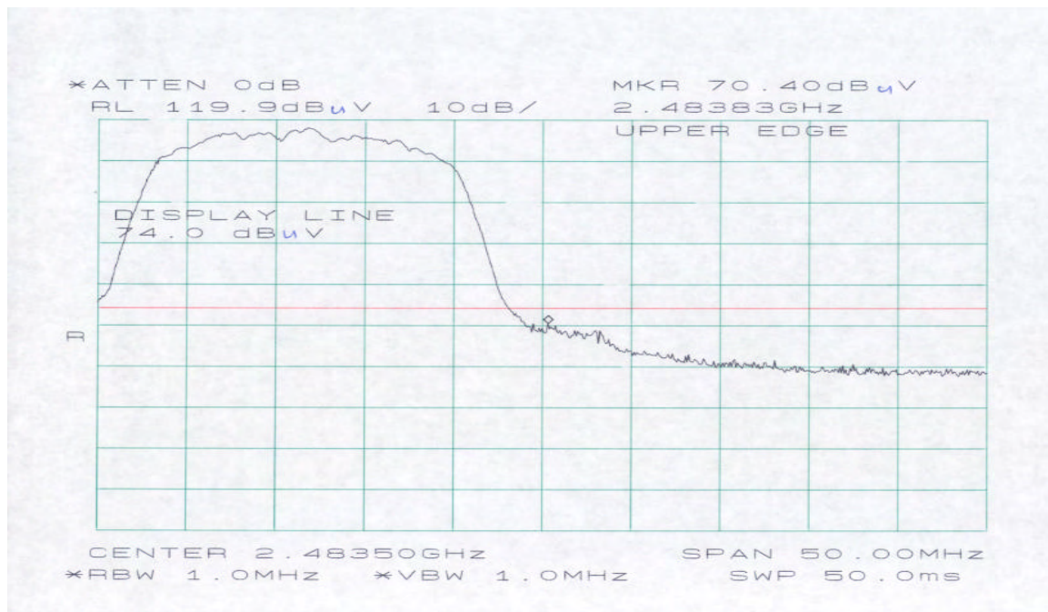
PEAK Limit at Upper Edge for 2470 MHz Plot
