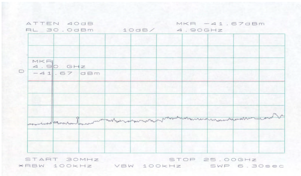
Conducted Spurious Emission for 2450 MHz (Mid channel)
