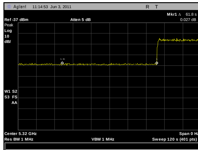
Plot 339. Channel Availability Check (CAC), 5320 MHz
