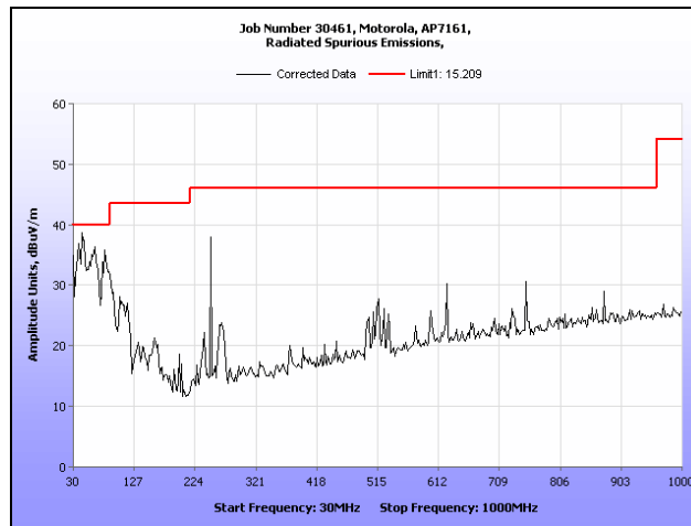
Plot 217. Radiated Spurious Emissions, 30 MHz – 1 GHz, 802.11n HT40, 5510 MHz
