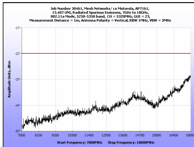
Plot 167. Radiated Spurious Emissions, 7 GHz – 18 GHz, 802.11a, 5320 MHz
