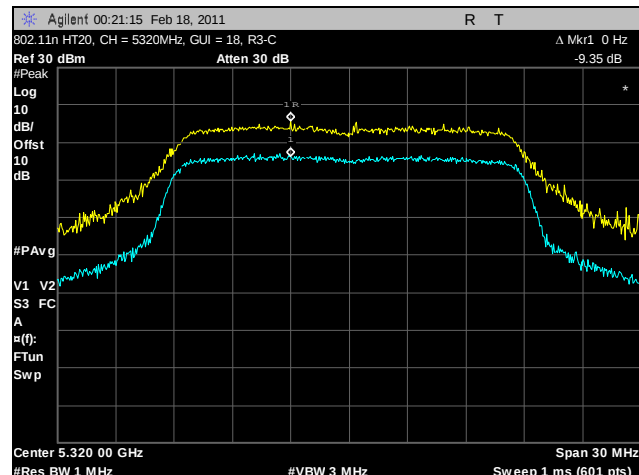
Plot 135. Peak Excursion Ratio, 802.11n HT20, 5320 MHz, R3-C
