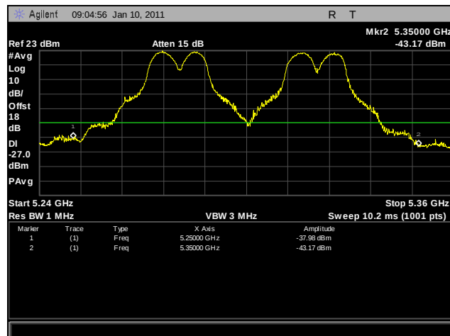
Plot 280. Frequency Stability, 60°C for 5250 MHz – 5350 MHz at 120 VAC
