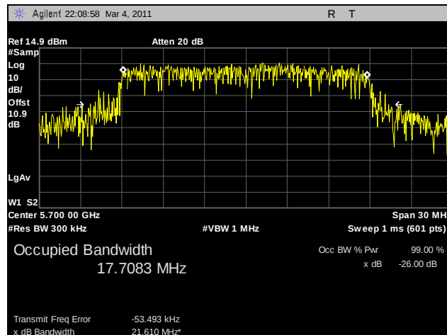
Plot 93. 99% Occupied Bandwidth, 802.11n HT20, 5700 MHz, R3-C
