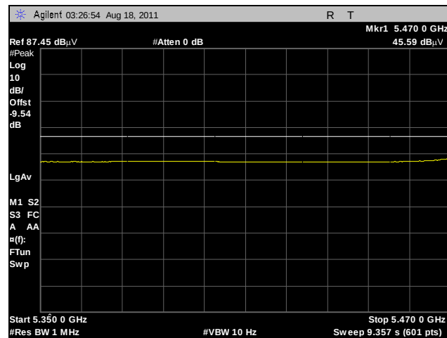
Plot 231. Radiated Restricted Band, 802.11a, 5500 MHz, Average
