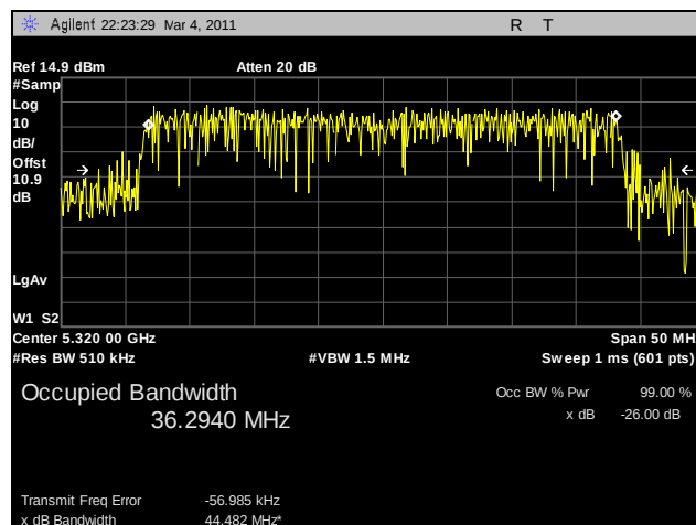
Plot 102. 99% Occupied Bandwidth, 802.11n HT40, 5320 MHz, R3-C
