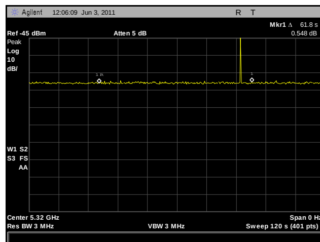
Plot 341. Channel Availability Check (CAC), End Burst, 5320 MHz
