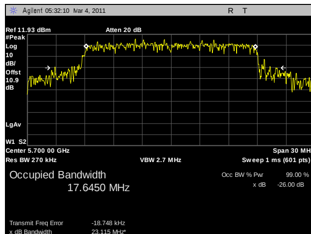
Plot 42. 26 dB Occupied Bandwidth, 802.11n HT20, 5700 MHz, R3-C
