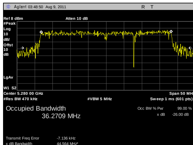
Plot 45. 26 dB Occupied Bandwidth, 802.11n HT40, 5280 MHz, R3-C
