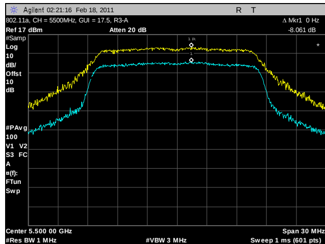
Plot 118. Peak Excursion Ratio, 802.11a, 5500 MHz, R3-A
