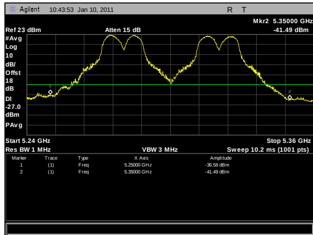
Plot 252. Frequency Stability, -30°C for 5250 MHz – 5350 MHz at 102 VAC
