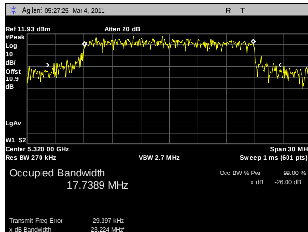
Plot 32. 26 dB Occupied Bandwidth, 802.11n HT20, 5320 MHz, R3-B
