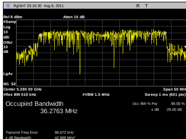
Plot 96. 99% Occupied Bandwidth, 802.11n HT40, 5280 MHz, R3-C
