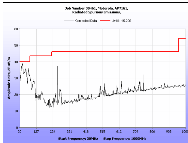
Plot 209. Radiated Spurious Emissions, 30 MHz – 1 GHz, 802.11n HT40, 5300 MHz
