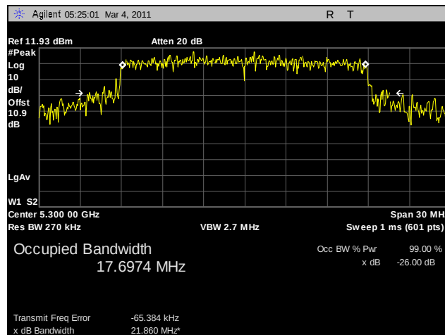
Plot 29. 26 dB Occupied Bandwidth, 802.11n HT20, 5300 MHz, R3-B
