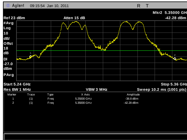
Plot 282. Frequency Stability, 70°C for 5250 MHz – 5350 MHz at 102 VAC
