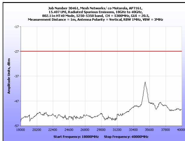
Plot 212. Radiated Spurious Emissions, 18 GHz – 40 GHz, 802.11n HT40, 5300 MHz
