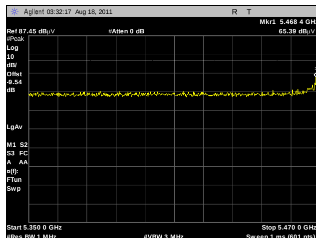
Plot 246. Radiated Restricted Band, 802.11n HT40, 5510 MHz, Peak
