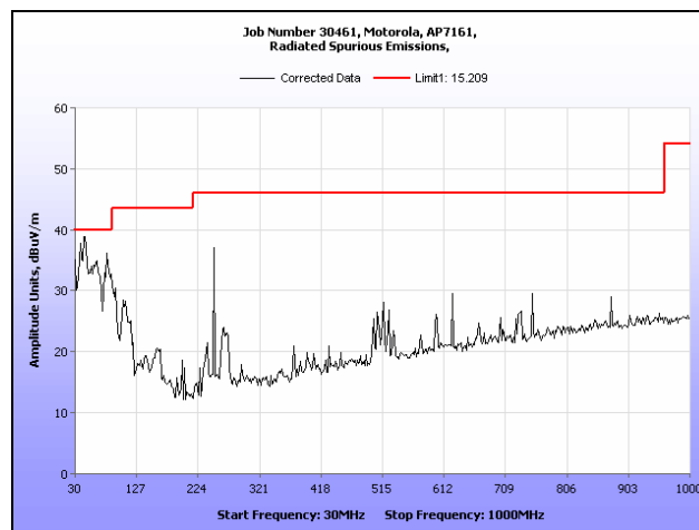
Plot 189. Radiated Spurious Emissions, 30 MHz – 1 GHz, 802.11n HT20, 5320 MHz
