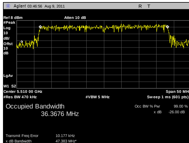
Plot 53. 26 dB Occupied Bandwidth, 802.11n HT40, 5510 MHz, R3-B
