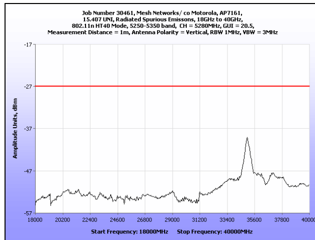
Plot 208. Radiated Spurious Emissions, 18 GHz – 40 GHz, 802.11n HT40, 5280 MHz
