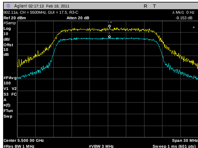
Plot 120. Peak Excursion Ratio, 802.11a, 5500 MHz, R3-C
