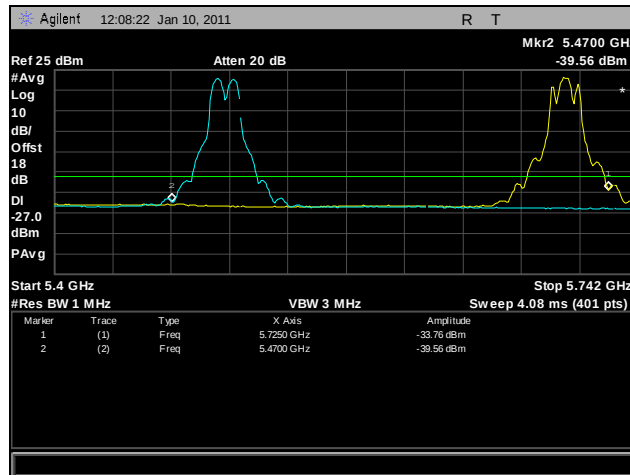
Plot 306. Frequency Stability, 30°C for 5470 MHz - 5725 MHz at 102 VAC
