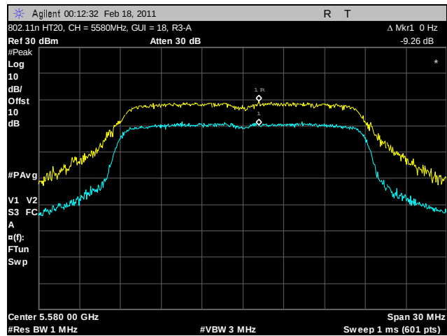
Plot 139. Peak Excursion Ratio, 802.11n HT20, 5580 MHz, R3-A
