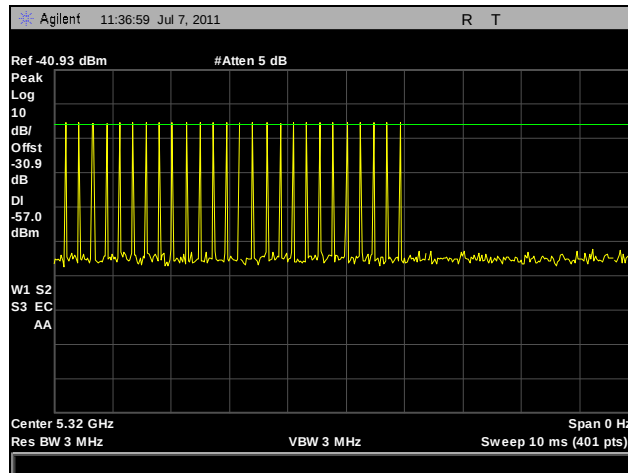
Plot 334. Bin 2 Radar Calibration for 5 dBi
