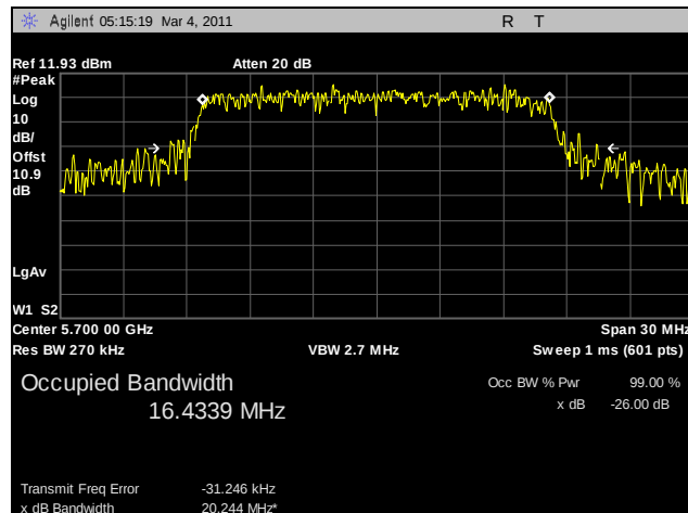
Plot 24. 26 dB Occupied Bandwidth, 802.11a, 5700 MHz, R3-C
