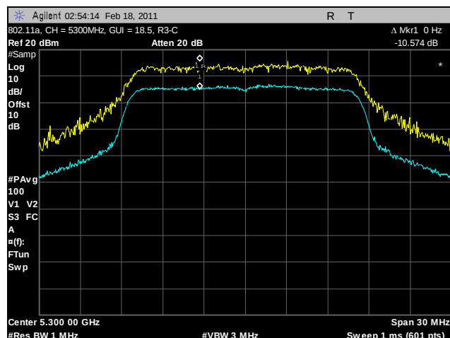
Plot 114. Peak Excursion Ratio, 802.11a, 5300 MHz, R3-C
