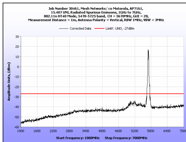
Plot 222. Radiated Spurious Emissions, 1 GHz – 7 GHz, 802.11n HT40, 5670 MHz
