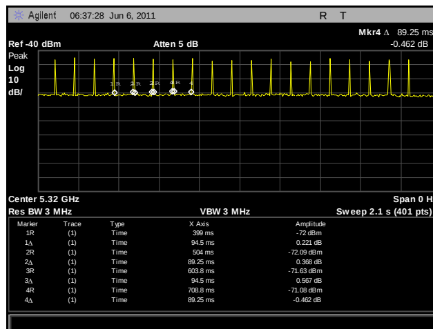
Plot 346. Channel Closing Transmission Time 2
