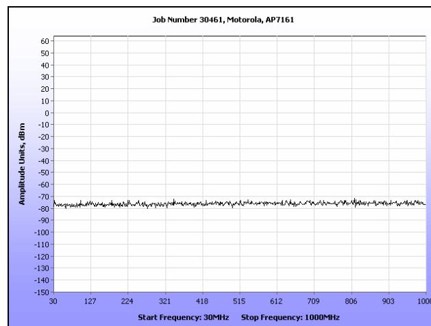
Plot 329. Receiver Spurious Emission, R3-B, 30 MHz – 1 GHz
