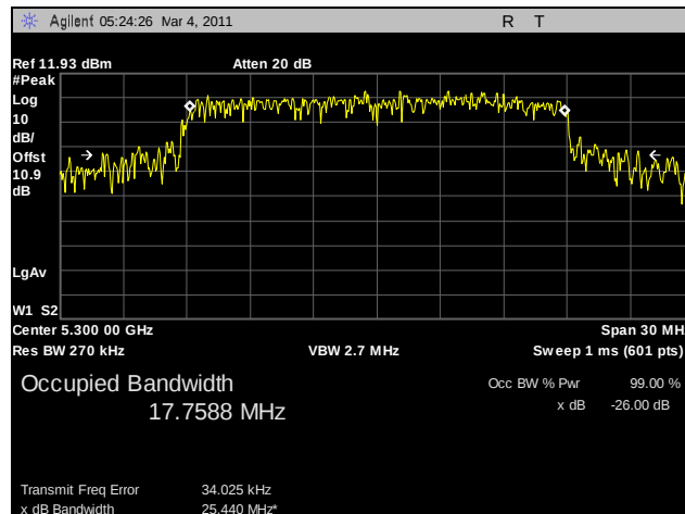
Plot 30. 26 dB Occupied Bandwidth, 802.11n HT20, 5300 MHz, R3-C
