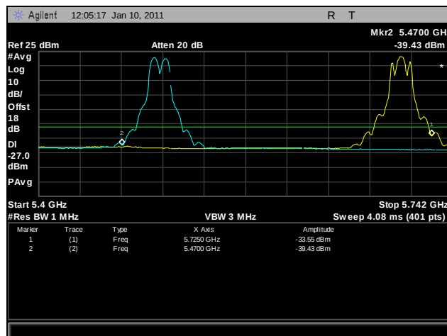
Plot 308. Frequency Stability, 30°C for 5470 MHz - 5725 MHz at 138 VAC
