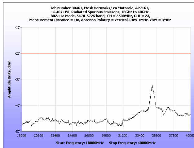
Plot 172. Radiated Spurious Emissions, 18 GHz – 40 GHz, 802.11a, 5500 MHz
