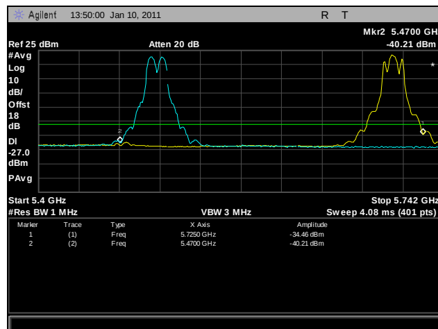
Plot 290. Frequency Stability, -30°C for 5470 MHz - 5725 MHz at 138 VAC
