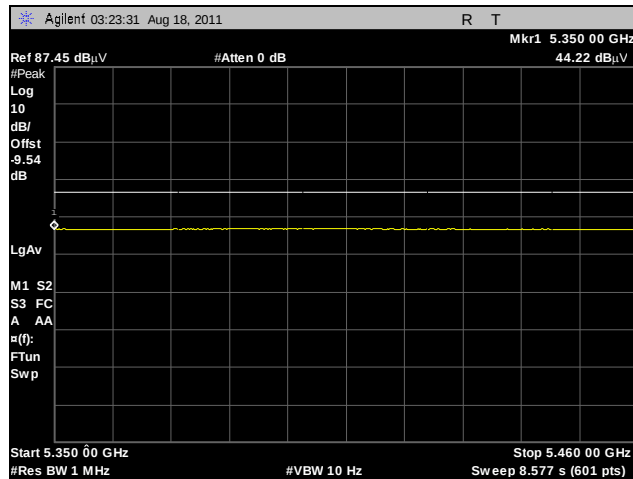
Plot 228. Radiated Restricted Band, 802.11a, 5320 MHz, Average
