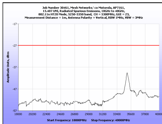
Plot 188. Radiated Spurious Emissions, 18 GHz – 40 GHz, 802.11n HT20, 5300 MHz
