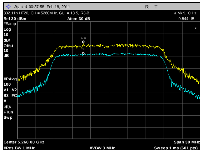
Plot 128. Peak Excursion Ratio, 802.11n HT20, 5260 MHz, R3-B
