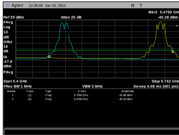
Plot 315. Frequency Stability, 60°C for 5470 MHz - 5725 MHz at 102 VAC
