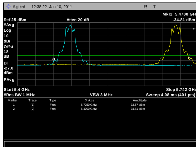
Plot 317. Frequency Stability, 60°C for 5470 MHz - 5725 MHz at 138 VAC
