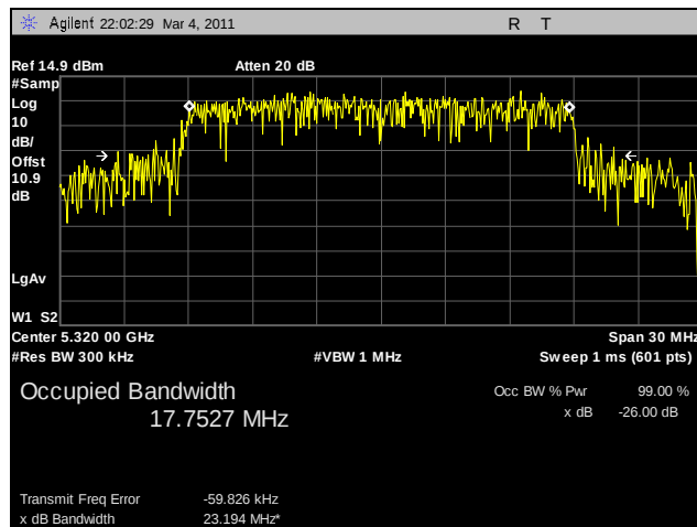
Plot 83. 99% Occupied Bandwidth, 802.11n HT20, 5320 MHz, R3-B
