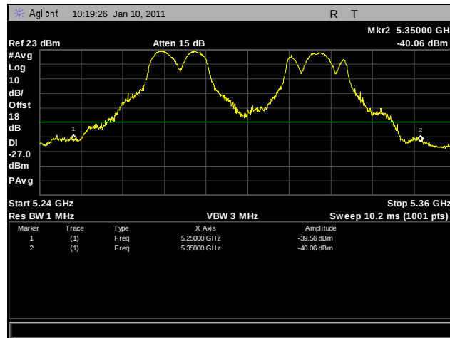
Plot 261. Frequency Stability, 0°C for 5250 MHz – 5350 MHz at 102 VAC
