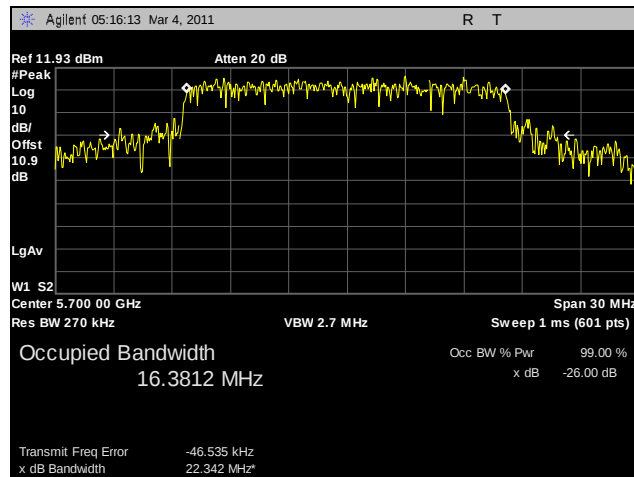
Plot 22. 26 dB Occupied Bandwidth, 802.11a, 5700 MHz, R3-A
