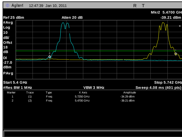
Plot 318. Frequency Stability, 70°C for 5470 MHz - 5725 MHz at 102 VAC
