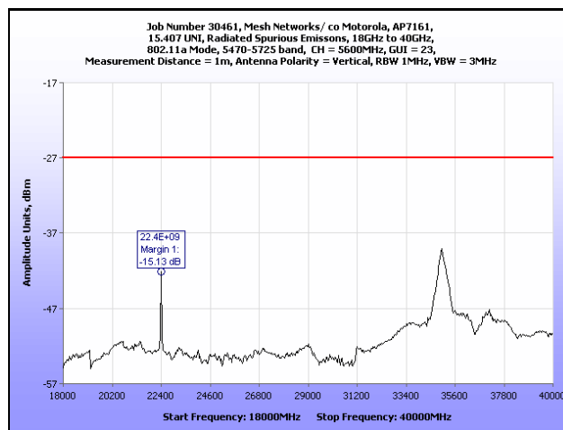
Plot 176. Radiated Spurious Emissions, 18 GHz – 40 GHz, 802.11a, 5600 MHz
