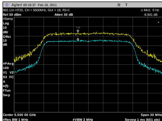
Plot 138. Peak Excursion Ratio, 802.11n HT20, 5500 MHz, R3-C
