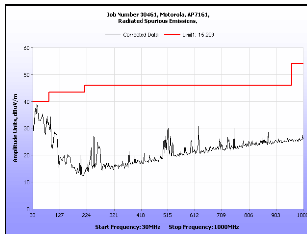
Plot 161. Radiated Spurious Emissions, 30 MHz – 1 GHz, 802.11a, 5300 MHz
