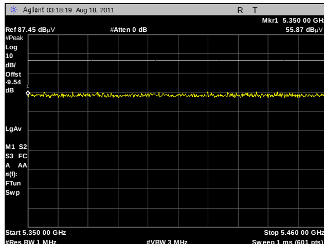
Plot 235. Radiated Restricted Band, 802.11n HT20, 5320 MHz, Peak
