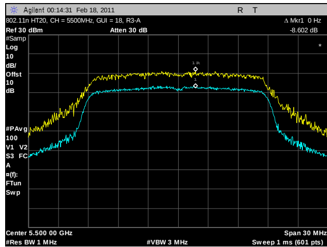
Plot 136. Peak Excursion Ratio, 802.11n HT20, 5500 MHz, R3-A
