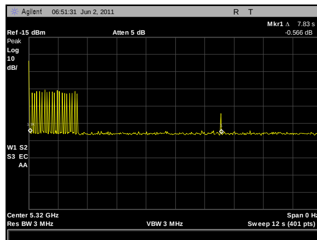
Plot 343. Channel Move Time, 5320 MHz
