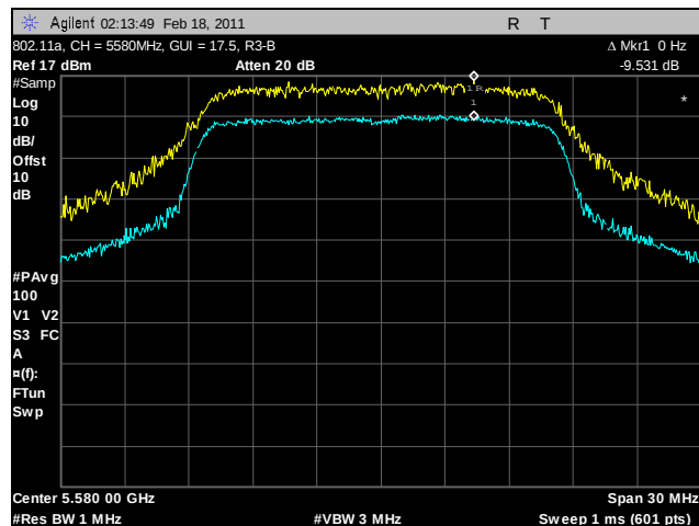
Plot 122. Peak Excursion Ratio, 802.11a, 5580 MHz, R3-B
