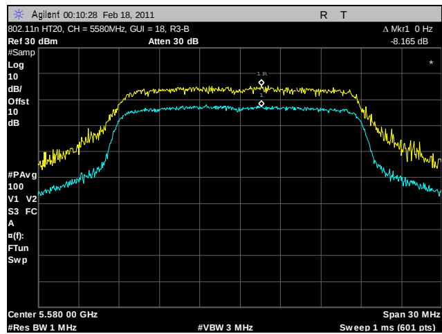
Plot 140. Peak Excursion Ratio, 802.11n HT20, 5580 MHz, R3-B
