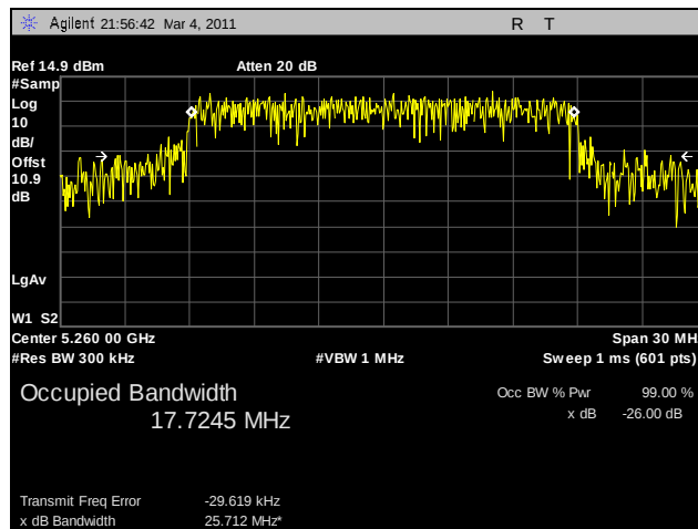
Plot 77. 99% Occupied Bandwidth, 802.11n HT20, 5260 MHz, R3-B
