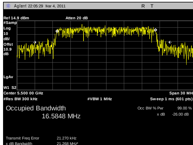
Plot 69. 99% Occupied Bandwidth, 802.11a, 5500 MHz, R3-C
