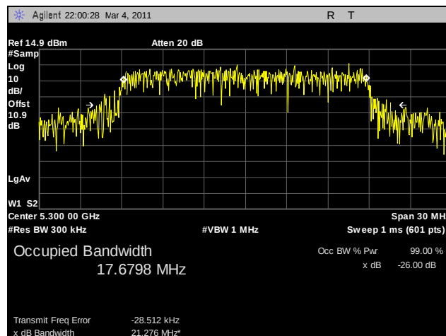
Plot 81. 99% Occupied Bandwidth, 802.11n HT20, 5300 MHz, R3-C
