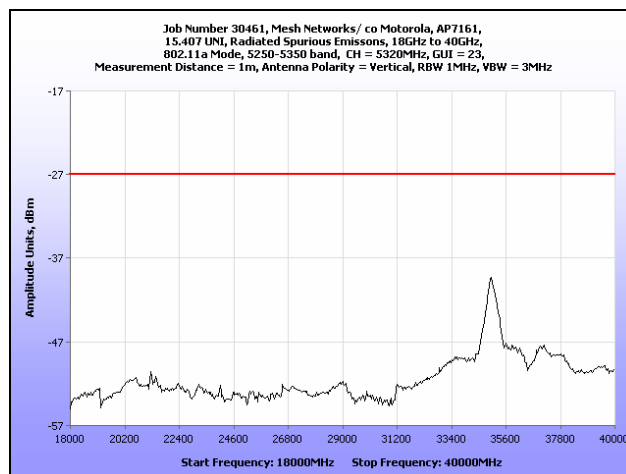
Plot 168. Radiated Spurious Emissions, 18 GHz – 40 GHz, 802.11a, 5320 MHz
