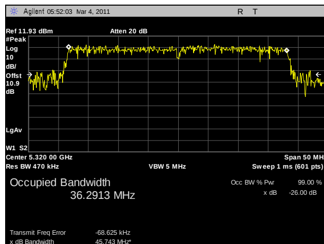
Plot 51. 26 dB Occupied Bandwidth, 802.11n HT40, 5320 MHz, R3-C
