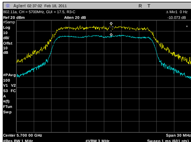
Plot 126. Peak Excursion Ratio, 802.11a, 5700 MHz, R3-C
