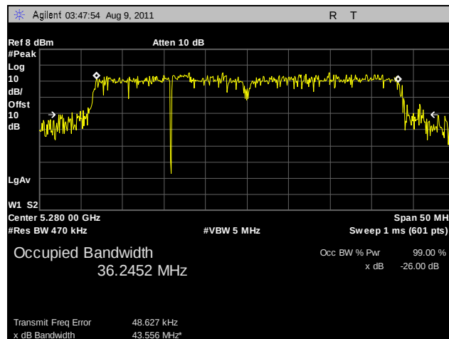
Plot 44. 26 dB Occupied Bandwidth, 802.11n HT40, 5280 MHz, R3-B
