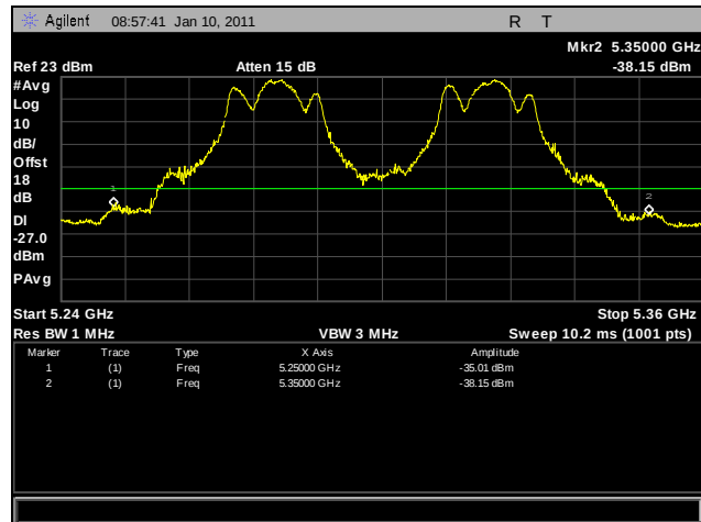
Plot 276. Frequency Stability, 50°C for 5250 MHz – 5350 MHz at 102 VAC
