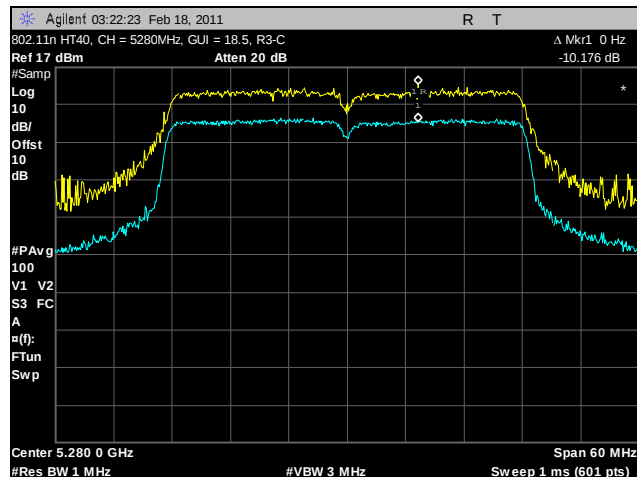
Plot 147. Peak Excursion Ratio, 802.11n HT40, 5280 MHz, R3-C
