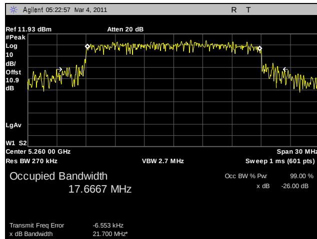
Plot 25. 26 dB Occupied Bandwidth, 802.11n HT20, 5260 MHz, R3-A
