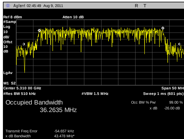
Plot 97. 99% Occupied Bandwidth, 802.11n HT40, 5310 MHz, R3-A
