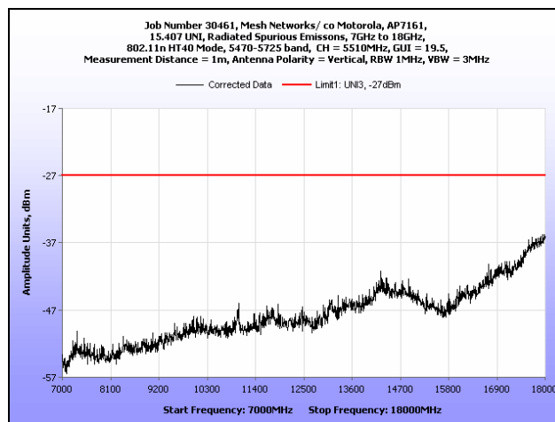
Plot 219. Radiated Spurious Emissions, 7 GHz – 18 GHz, 802.11n HT40, 5510 MHz
