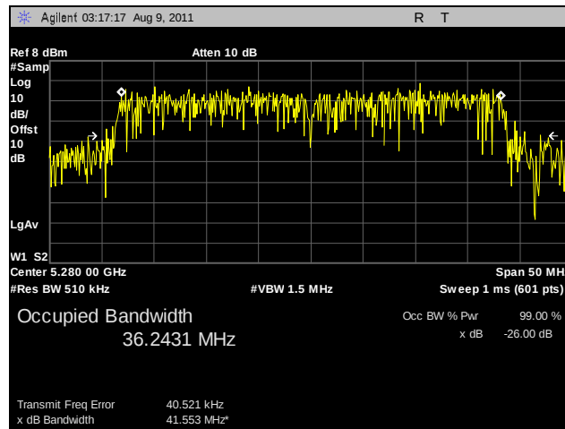
Plot 94. 99% Occupied Bandwidth, 802.11n HT40, 5280 MHz, R3-A
