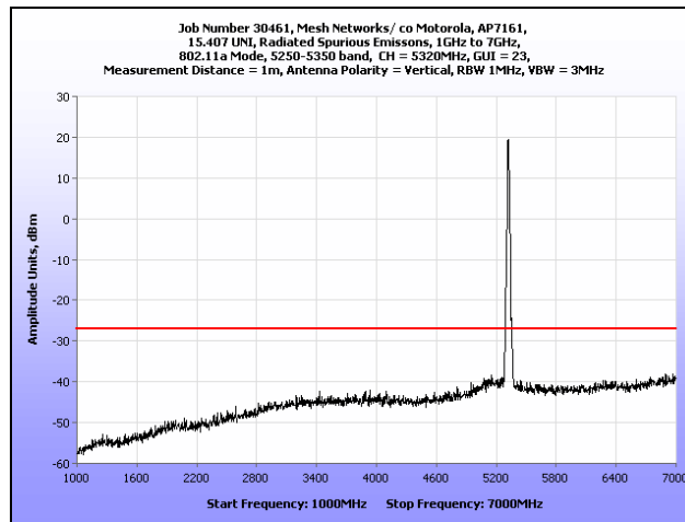
Plot 166. Radiated Spurious Emissions, 1 GHz – 7 GHz, 802.11a, 5320 MHz
