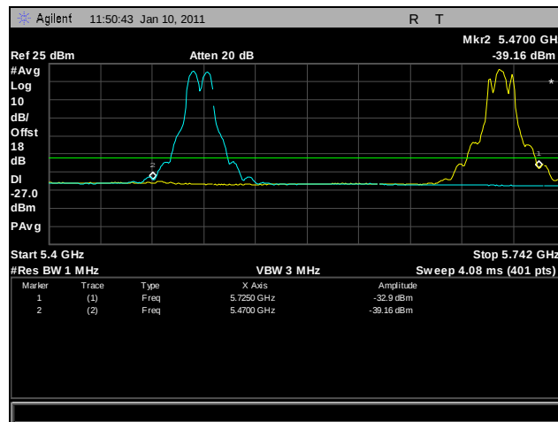
Plot 303. Frequency Stability, 20°C for 5470 MHz - 5725 MHz at 102 VAC
