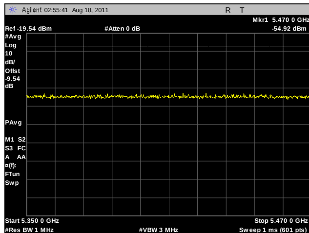
Plot 229. Radiated Band Edge, 802.11a, 5500 MHz
