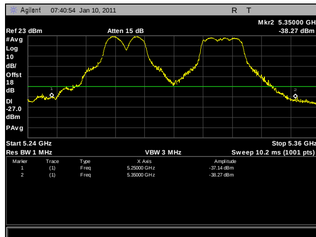
Plot 268. Frequency Stability, 20°C for 5250 MHz – 5350 MHz at 120 VAC
