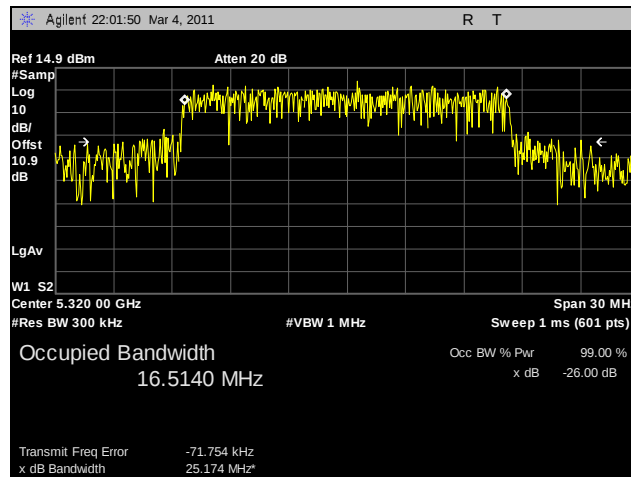
Plot 64. 99% Occupied Bandwidth, 802.11a, 5320 MHz, R3-A
