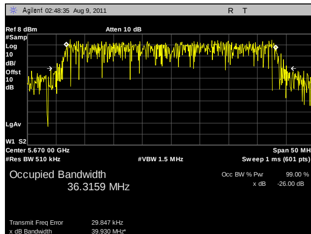
Plot 107. 99% Occupied Bandwidth, 802.11n HT40, 5670 MHz, R3-B
