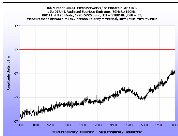
Plot 203. Radiated Spurious Emissions, 7 GHz – 18 GHz, 802.11n HT20, 5700 MHz
