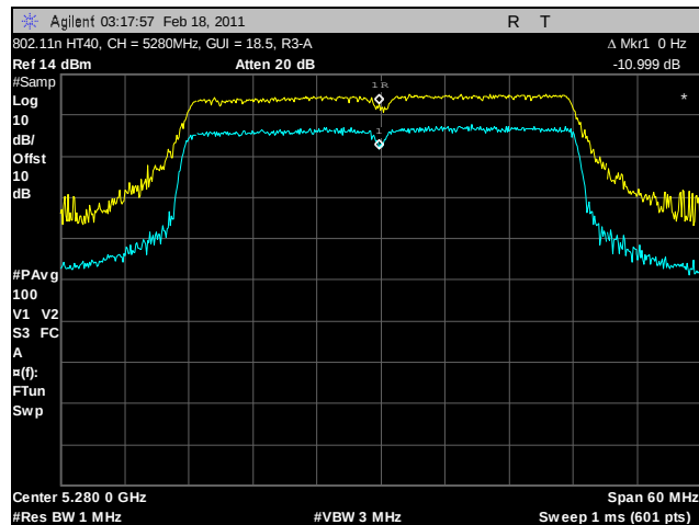
Plot 145. Peak Excursion Ratio, 802.11n HT40, 5280 MHz, R3-A
