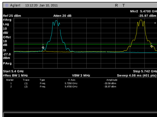
Plot 302. Frequency Stability, 10°C for 5470 MHz - 5725 MHz at 138 VAC
