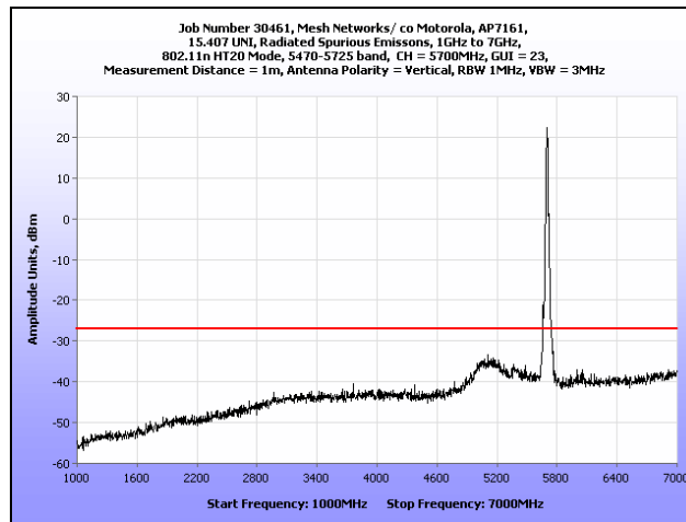
Plot 202. Radiated Spurious Emissions, 1 GHz – 7 GHz, 802.11n HT20, 5700 MHz
