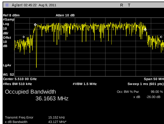
Plot 103. 99% Occupied Bandwidth, 802.11n HT40, 5510 MHz, R3-A
