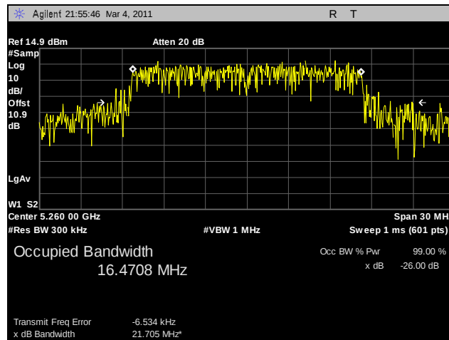
Plot 58. 99% Occupied Bandwidth, 802.11a, 5260 MHz, R3-A
