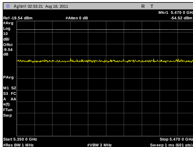
Plot 237. Radiated Band Edge, 802.11n HT20, 5500 MHz
