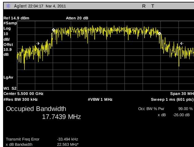
Plot 85. 99% Occupied Bandwidth, 802.11n HT20, 5500 MHz, R3-A
