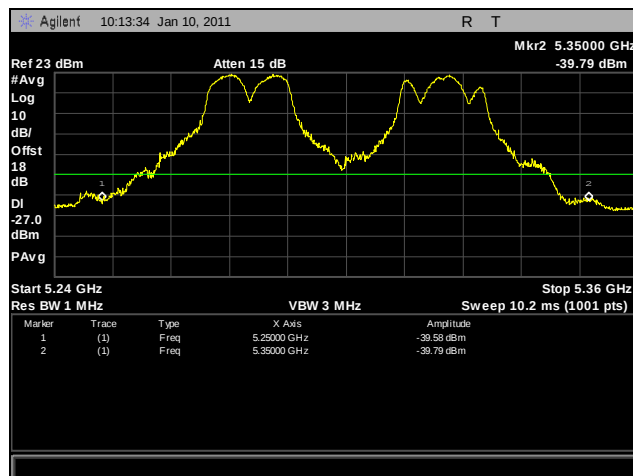
Plot 266. Frequency Stability, 10°C for 5250 MHz – 5350 MHz at 138 VAC
