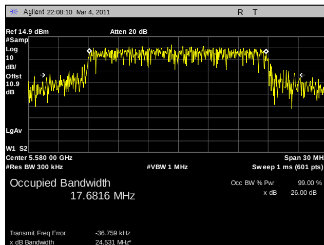
Plot 89. 99% Occupied Bandwidth, 802.11n HT20, 5580 MHz, R3-B
