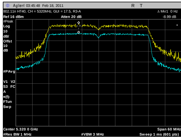
Plot 148. Peak Excursion Ratio, 802.11n HT40, 5320 MHz, R3-A
