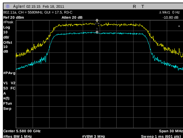
Plot 123. Peak Excursion Ratio, 802.11a, 5580 MHz, R3-C
