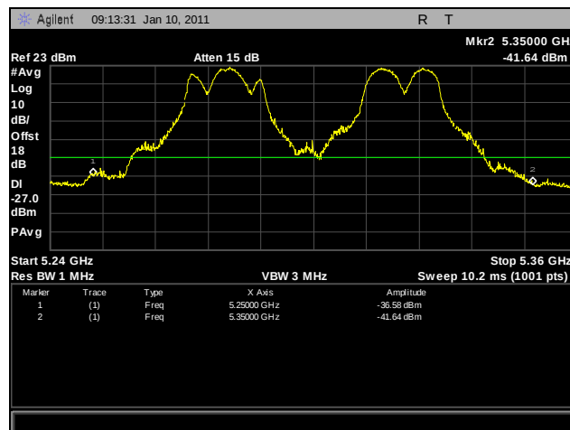
Plot 284. Frequency Stability, 70°C for 5250 MHz – 5350 MHz at 138 VAC
