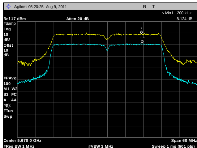
Plot 156. Peak Excursion Ratio, 802.11n HT40, 5670 MHz, R3-C
