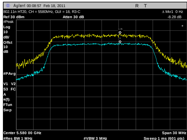
Plot 141. Peak Excursion Ratio, 802.11n HT20, 5580 MHz, R3-C
