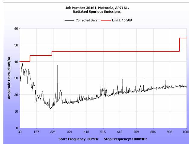
Plot 193. Radiated Spurious Emissions, 30 MHz – 1 GHz, 802.11n HT20, 5500 MHz
