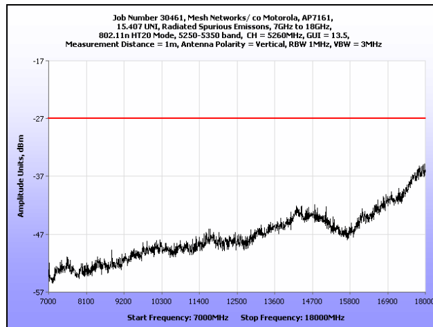
Plot 183. Radiated Spurious Emissions, 7 GHz – 18 GHz, 802.11n HT20, 5260 MHz
