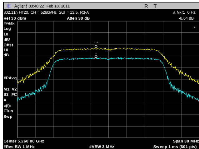
Plot 127. Peak Excursion Ratio, 802.11n HT20, 5260 MHz, R3-A
