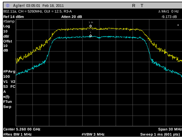
Plot 109. Peak Excursion Ratio, 802.11a, 5260 MHz, R3-A
