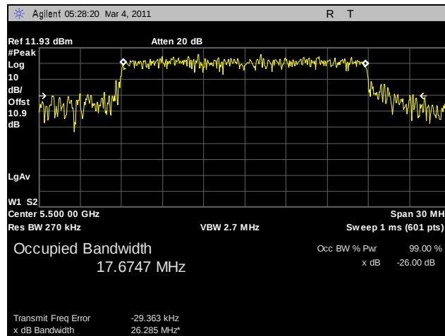
Plot 34. 26 dB Occupied Bandwidth, 802.11n HT20, 5500 MHz, R3-A
