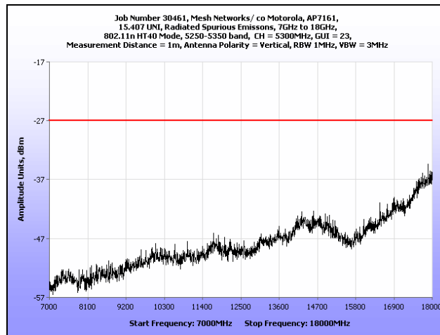
Plot 211. Radiated Spurious Emissions, 7 GHz – 18 GHz, 802.11n HT40, 5300 MHz
