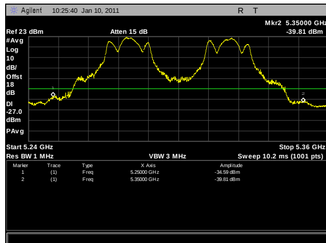
Plot 259. Frequency Stability, -10°C for 5250 MHz – 5350 MHz at 120 VAC
