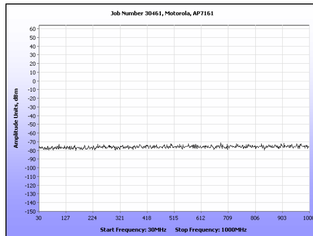
Plot 323. Receiver Spurious Emission, R3-B, 30 MHz – 1 GHz
