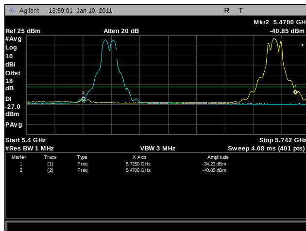
Plot 287. Frequency Stability, -40°C for 5470 MHz - 5725 MHz at 138 VAC
