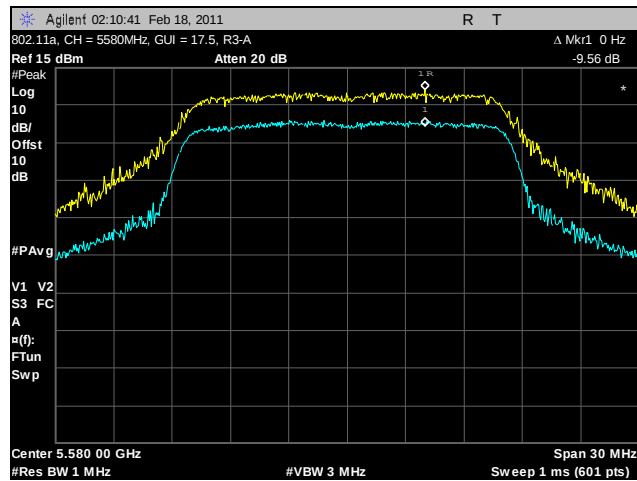
Plot 121. Peak Excursion Ratio, 802.11a, 5580 MHz, R3-A
