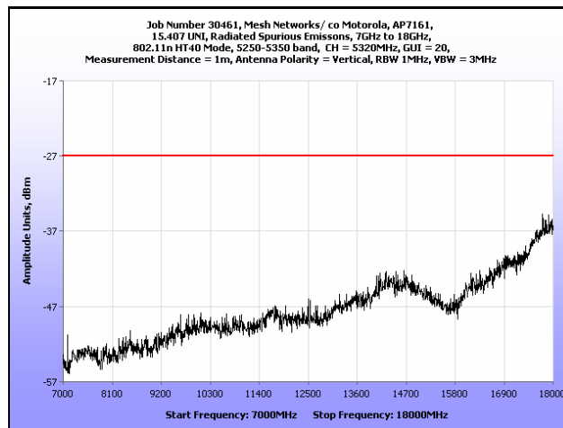
Plot 215. Radiated Spurious Emissions, 7 GHz – 18 GHz, 802.11n HT40, 5320 MHz
