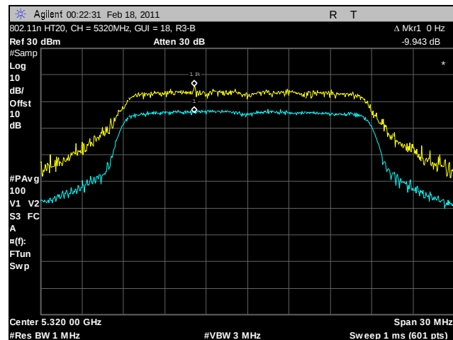
Plot 134. Peak Excursion Ratio, 802.11n HT20, 5320 MHz, R3-B
