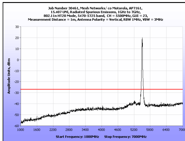
Plot 194. Radiated Spurious Emissions, 1 GHz – 7 GHz, 802.11n HT20, 5500 MHz
