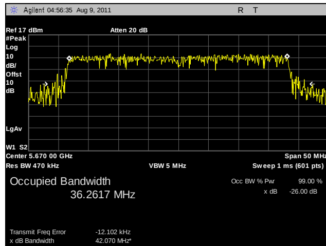
Plot 55. 26 dB Occupied Bandwidth, 802.11n HT40, 5670 MHz, R3-A
