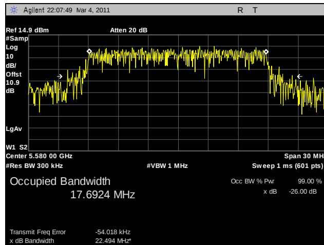
Plot 88. 99% Occupied Bandwidth, 802.11n HT20, 5580 MHz, R3-A
