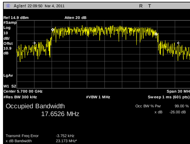
Plot 91. 99% Occupied Bandwidth, 802.11n HT20, 5700 MHz, R3-A
