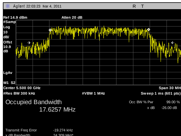
Plot 87. 99% Occupied Bandwidth, 802.11n HT20, 5500 MHz, R3-C
