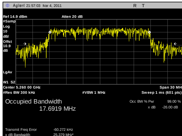
Plot 78. 99% Occupied Bandwidth, 802.11n HT20, 5260 MHz, R3-C
