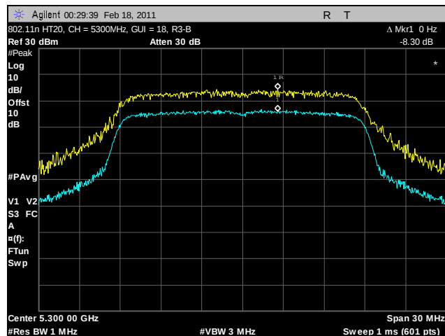
Plot 131. Peak Excursion Ratio, 802.11n HT20, 5300 MHz, R3-B
