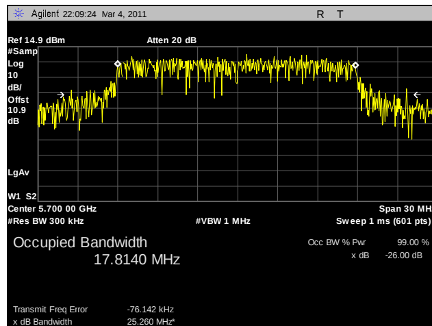
Plot 92. 99% Occupied Bandwidth, 802.11n HT20, 5700 MHz, R3-B
