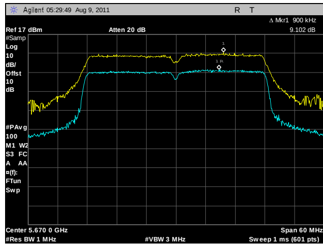
Plot 154. Peak Excursion Ratio, 802.11n HT40, 5670 MHz, R3-A
