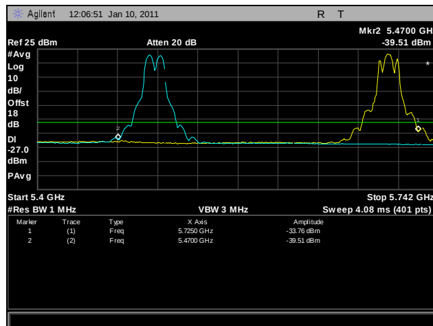
Plot 307. Frequency Stability, 30°C for 5470 MHz - 5725 MHz at 120 VAC
