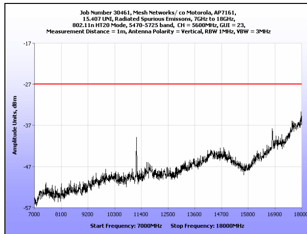
Plot 199. Radiated Spurious Emissions, 7 GHz – 18 GHz, 802.11n HT20, 5600 MHz
