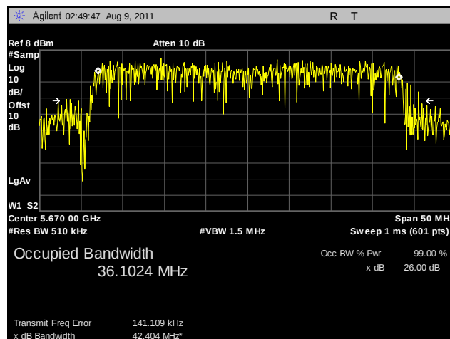
Plot 108. 99% Occupied Bandwidth, 802.11n HT40, 5670 MHz, R3-C
