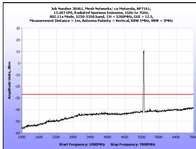
Plot 158. Radiated Spurious Emissions, 1 GHz – 7 GHz, 802.11a, 5260 MHz
