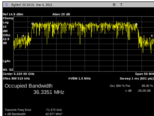
Plot 100. 99% Occupied Bandwidth, 802.11n HT40, 5320 MHz, R3-A
