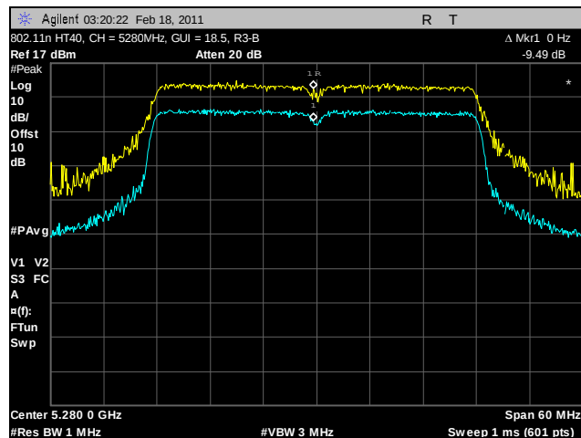
Plot 146. Peak Excursion Ratio, 802.11n HT40, 5280 MHz, R3-B
