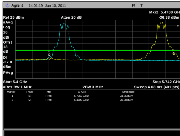
Plot 285. Frequency Stability, -40°C for 5470 MHz - 5725 MHz at 102 VAC
