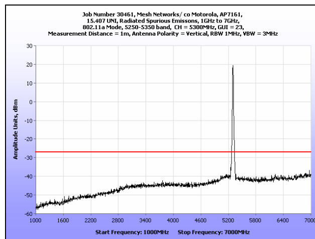
Plot 162. Radiated Spurious Emissions, 1 GHz – 7 GHz, 802.11a, 5300 MHz
