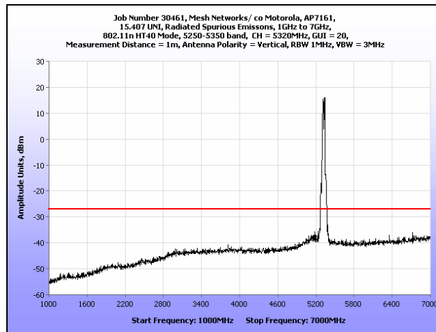
Plot 214. Radiated Spurious Emissions, 1 GHz – 7 GHz, 802.11n HT40, 5320 MHz
