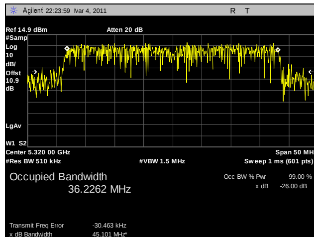
Plot 101. 99% Occupied Bandwidth, 802.11n HT40, 5320 MHz, R3-B
