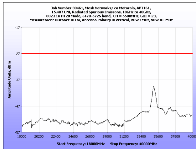
Plot 196. Radiated Spurious Emissions, 18 GHz – 40 GHz, 802.11n HT20, 5500 MHz
