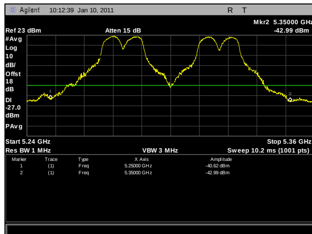
Plot 265. Frequency Stability, 10°C for 5250 MHz – 5350 MHz at 120 VAC
