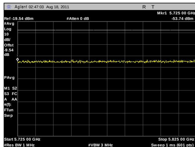
Plot 232. Radiated Band Edge, 802.11a, 5700 MHz
