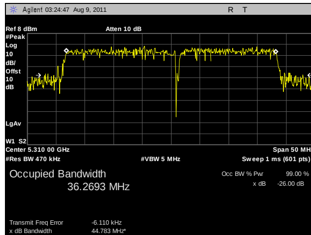
Plot 46. 26 dB Occupied Bandwidth, 802.11n HT40, 5310 MHz, R3-A
