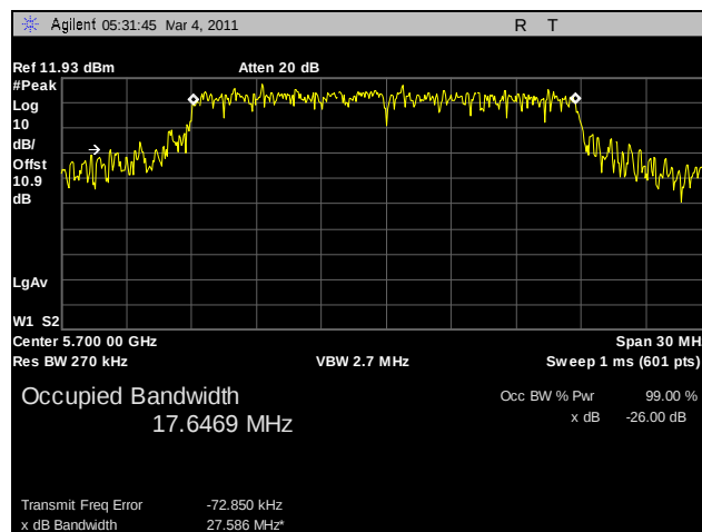
Plot 41. 26 dB Occupied Bandwidth, 802.11n HT20, 5700 MHz, R3-B
