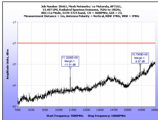
Plot 175. Radiated Spurious Emissions, 7 GHz – 18 GHz, 802.11a, 5600 MHz
