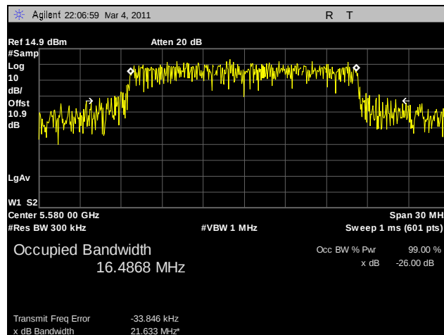
Plot 71. 99% Occupied Bandwidth, 802.11a, 5580 MHz, R3-B
