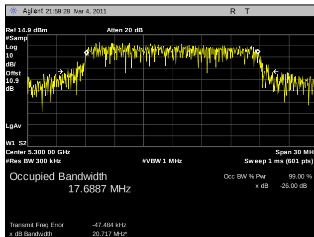
Plot 80. 99% Occupied Bandwidth, 802.11n HT20, 5300 MHz, R3-B
