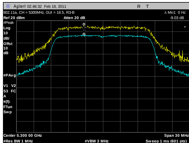
Plot 113. Peak Excursion Ratio, 802.11a, 5300 MHz, R3-B
