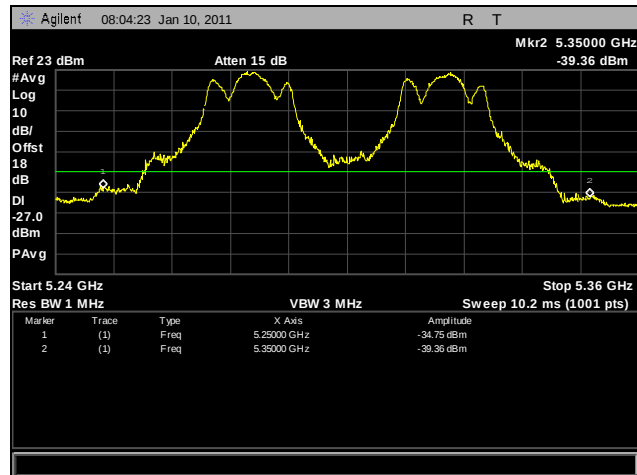
Plot 270. Frequency Stability, 30°C for 5250 MHz – 5350 MHz at 102 VAC
