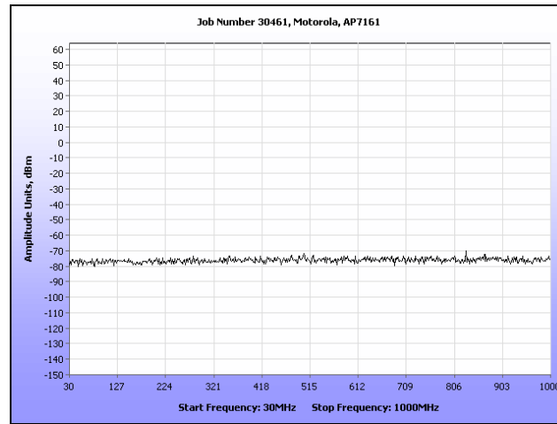
Plot 321. Receiver Spurious Emission, R3-A, 30 MHz – 1 GHz
