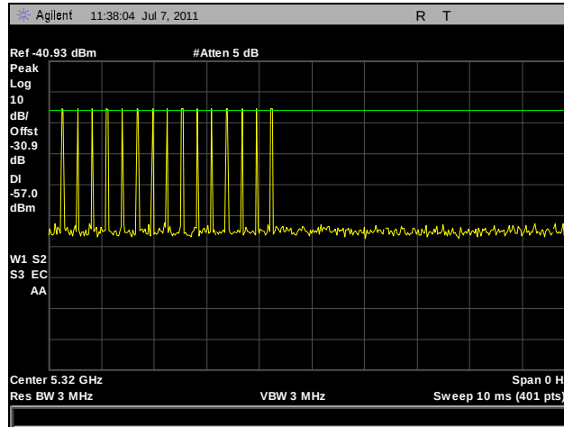
Plot 336. Bin 4 Radar Calibration for 5 dBi
