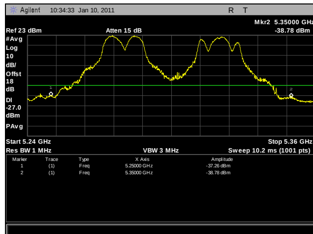
Plot 256. Frequency Stability, -20°C for 5250 MHz – 5350 MHz at 120 VAC
