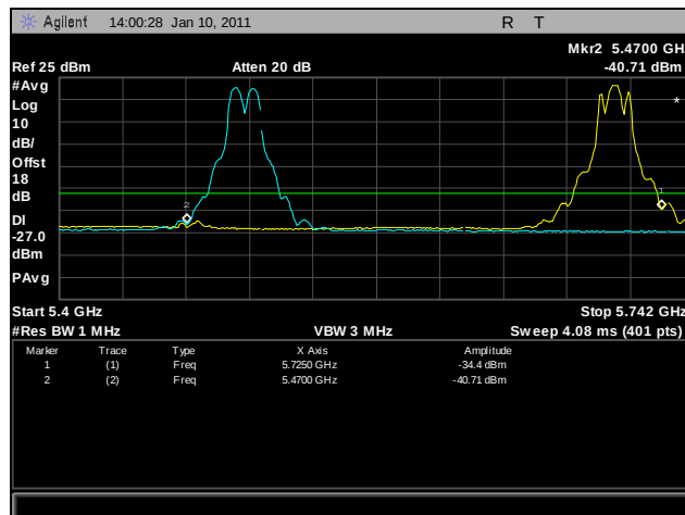
Plot 286. Frequency Stability, -40°C for 5470 MHz - 5725 MHz at 120 VAC
