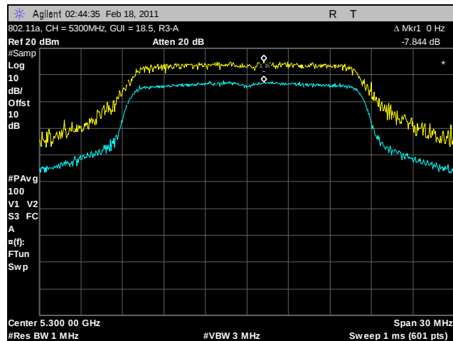
Plot 112. Peak Excursion Ratio, 802.11a, 5300 MHz, R3-A
