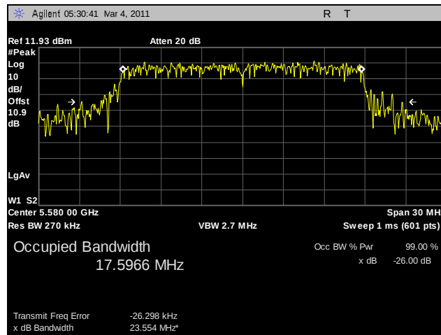
Plot 37. 26 dB Occupied Bandwidth, 802.11n HT20, 5580 MHz, R3-A
