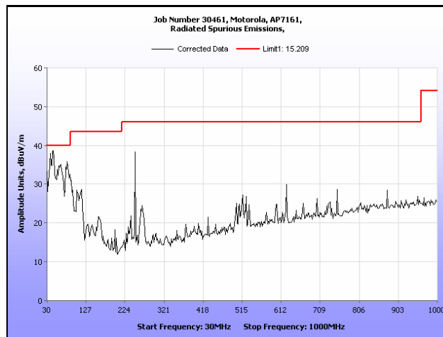
Plot 197. Radiated Spurious Emissions, 30 MHz – 1 GHz, 802.11n HT20, 5580 MHz
