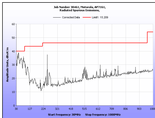
Plot 213. Radiated Spurious Emissions, 30 MHz – 1 GHz, 802.11n HT40, 5320 MHz
