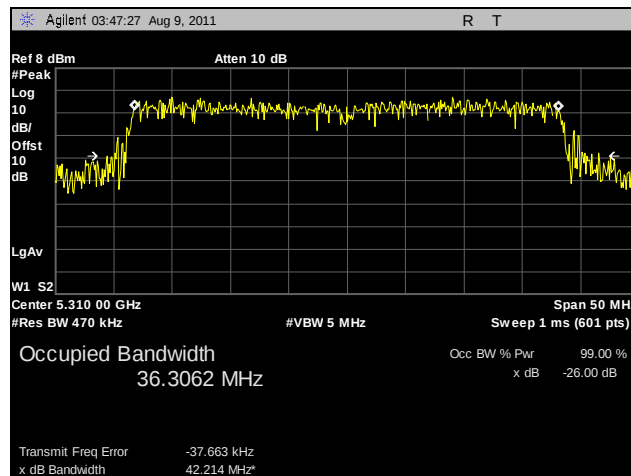
Plot 47. 26 dB Occupied Bandwidth, 802.11n HT40, 5310 MHz, R3-B
