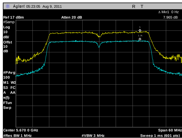
Plot 155. Peak Excursion Ratio, 802.11n HT40, 5670 MHz, R3-B
