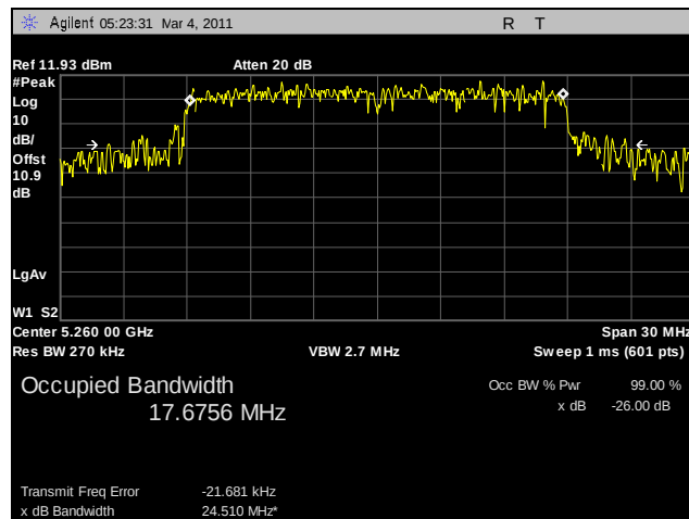
Plot 26. 26 dB Occupied Bandwidth, 802.11n HT20, 5260 MHz, R3-B
