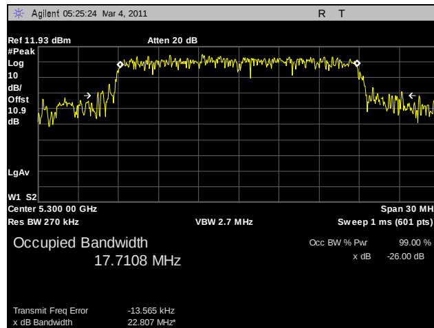
Plot 28. 26 dB Occupied Bandwidth, 802.11n HT20, 5300 MHz, R3-A
