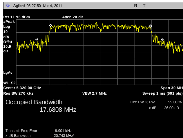
Plot 31. 26 dB Occupied Bandwidth, 802.11n HT20, 5320 MHz, R3-A
