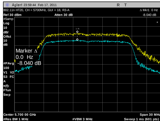
Plot 142. Peak Excursion Ratio, 802.11n HT20, 5700 MHz, R3-A
