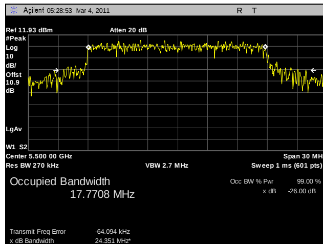
Plot 35. 26 dB Occupied Bandwidth, 802.11n HT20, 5500 MHz, R3-B
