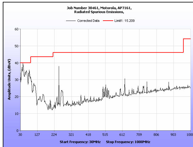
Plot 157. Radiated Spurious Emissions, 30 MHz – 1 GHz, 802.11a, 5260 MHz
