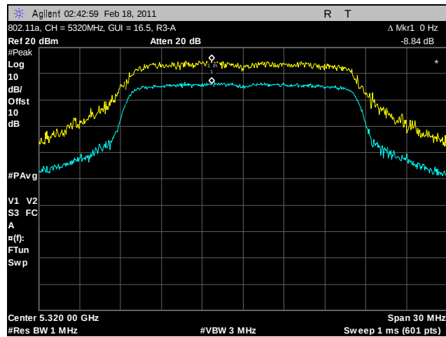
Plot 115. Peak Excursion Ratio, 802.11a, 5320 MHz, R3-A
