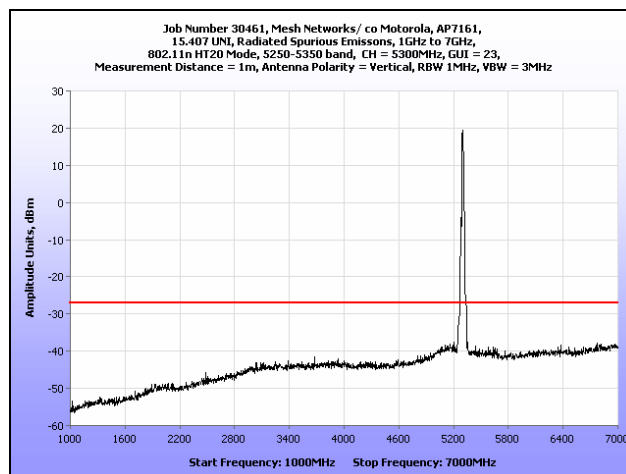
Plot 186. Radiated Spurious Emissions, 1 GHz – 7 GHz, 802.11n HT20, 5300 MHz
