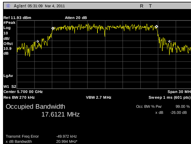
Plot 40. 26 dB Occupied Bandwidth, 802.11n HT20, 5700 MHz, R3-A
