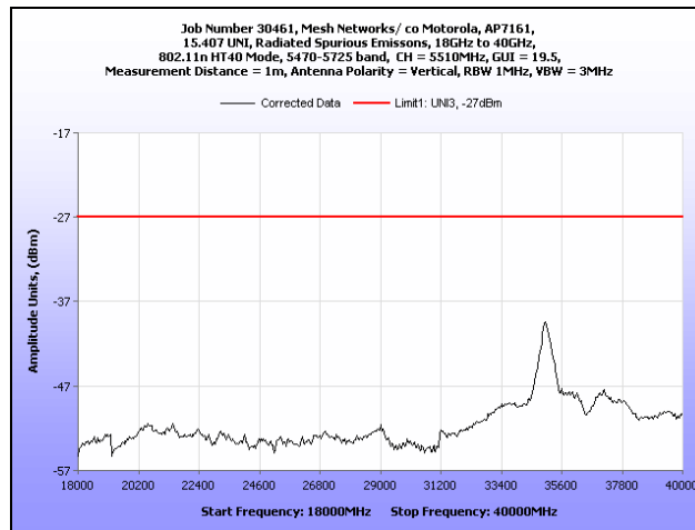
Plot 220. Radiated Spurious Emissions, 18 GHz – 40 GHz, 802.11n HT40, 5510 MHz
