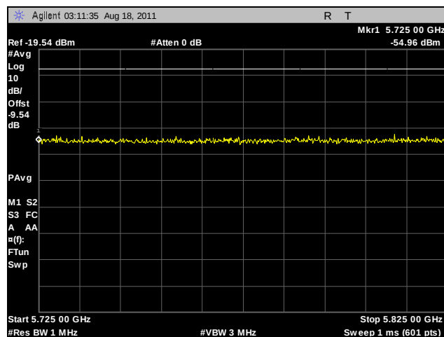
Plot 248. Radiated Band Edge, 802.11n HT40, 5670 MHz
