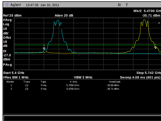
Plot 288. Frequency Stability, -30°C for 5470 MHz - 5725 MHz at 102 VAC
