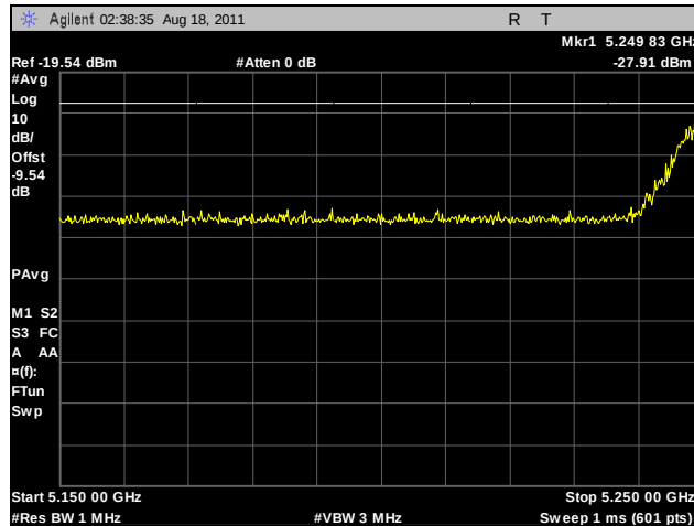
Plot 225. Radiated Band Edge, 802.11a, 5260 MHz
