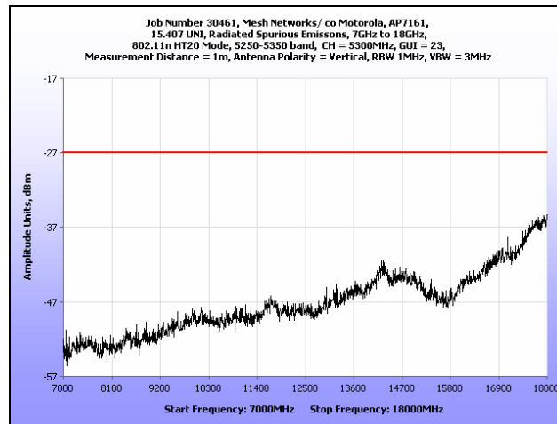
Plot 187. Radiated Spurious Emissions, 7 GHz – 18 GHz, 802.11n HT20, 5300 MHz
