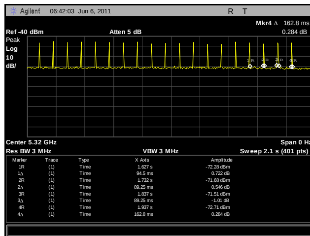
Plot 349. Channel Closing Transmission Time 5
