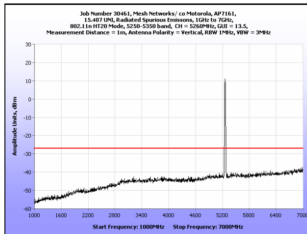
Plot 182. Radiated Spurious Emissions, 1 GHz – 7 GHz, 802.11n HT20, 5260 MHz
