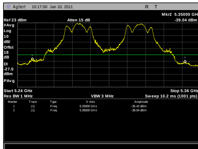
Plot 263. Frequency Stability, 0°C for 5250 MHz – 5350 MHz at 138 VAC
