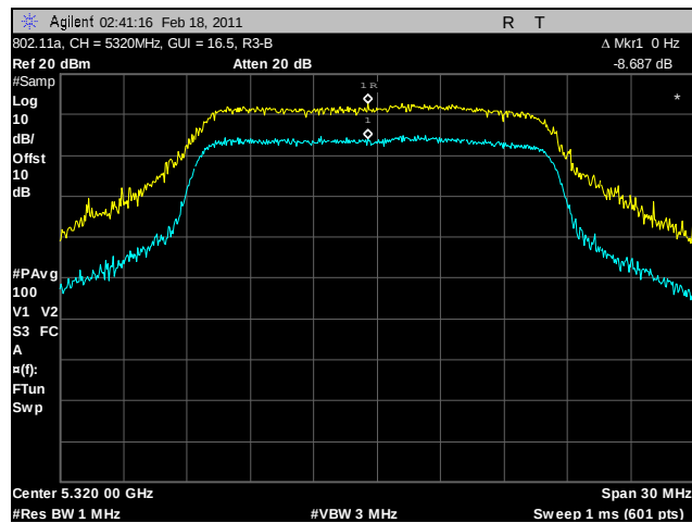
Plot 116. Peak Excursion Ratio, 802.11a, 5320 MHz, R3-B
