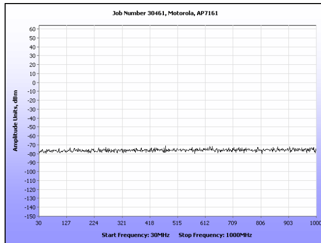
Plot 331. Receiver Spurious Emission, R3-C, 30 MHz - 1 GHz
