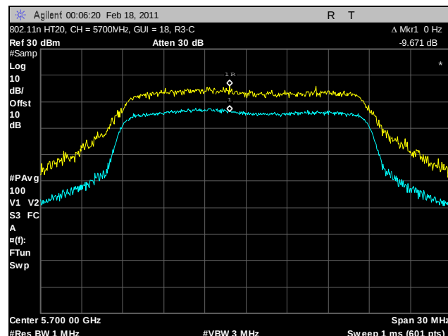
Plot 144. Peak Excursion Ratio, 802.11n HT20, 5700 MHz, R3-C
