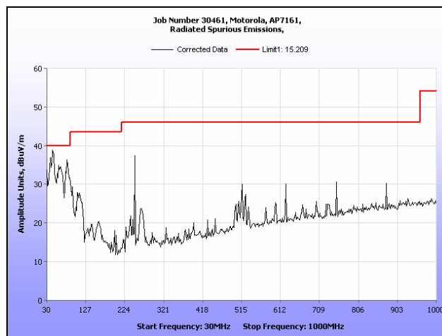
Plot 165. Radiated Spurious Emissions, 30 MHz – 1 GHz, 802.11a, 5320 MHz
