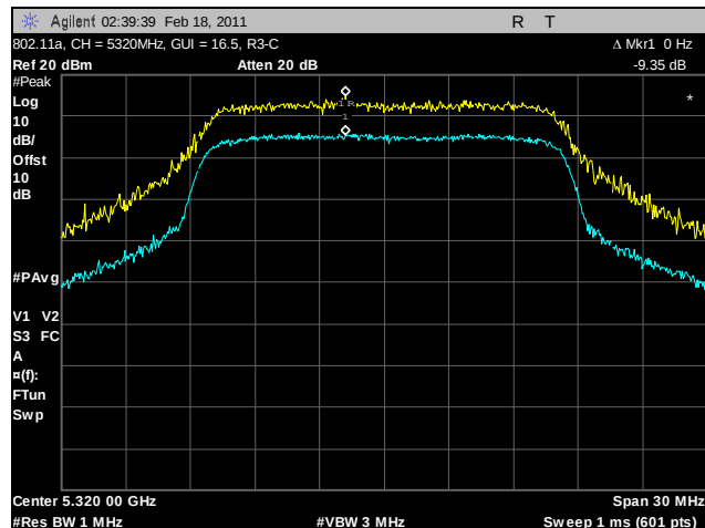
Plot 117. Peak Excursion Ratio, 802.11a, 5320 MHz, R3-C
