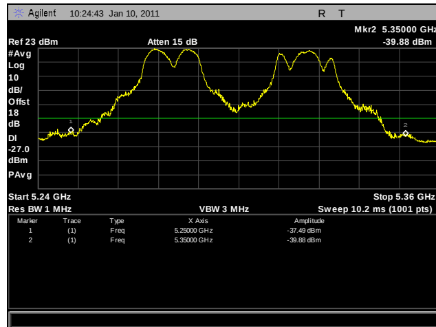
Plot 258. Frequency Stability, -10°C for 5250 MHz – 5350 MHz at 102 VAC
