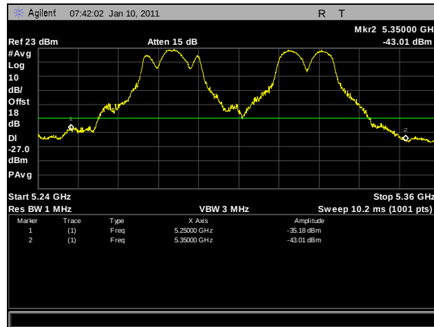
Plot 267. Frequency Stability, 20°C for 5250 MHz – 5350 MHz at 102 VAC
