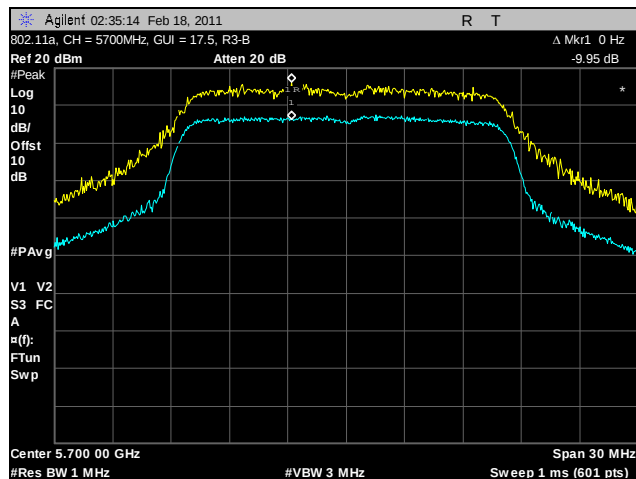
Plot 125. Peak Excursion Ratio, 802.11a, 5700 MHz, R3-B
