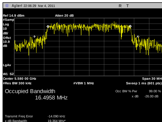
Plot 72. 99% Occupied Bandwidth, 802.11a, 5580 MHz, R3-C
