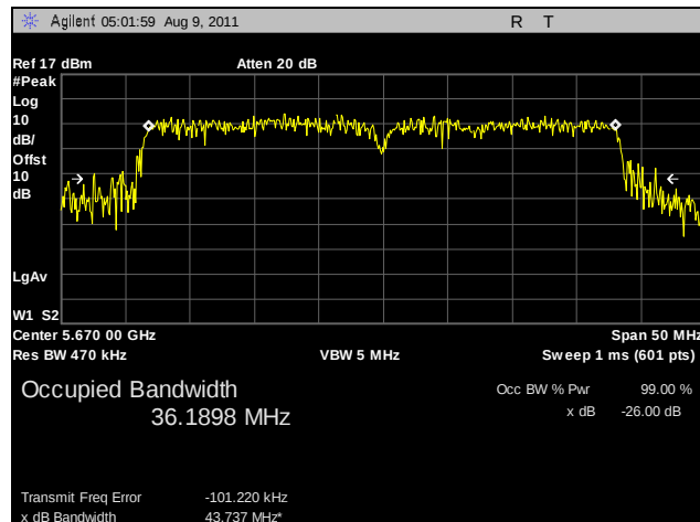
Plot 57. 26 dB Occupied Bandwidth, 802.11n HT40, 5670 MHz, R3-C
