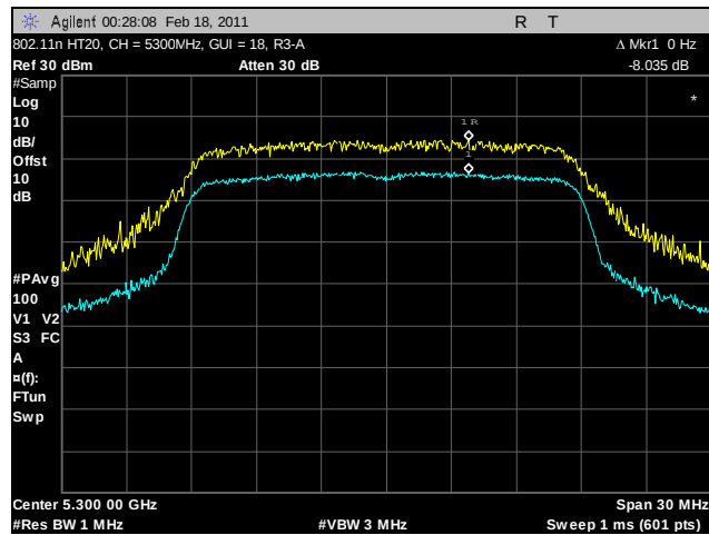
Plot 130. Peak Excursion Ratio, 802.11n HT20, 5300 MHz, R3-A
