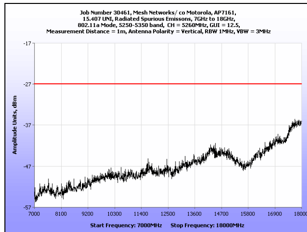
Plot 159. Radiated Spurious Emissions, 7 GHz – 18 GHz, 802.11a, 5260 MHz
