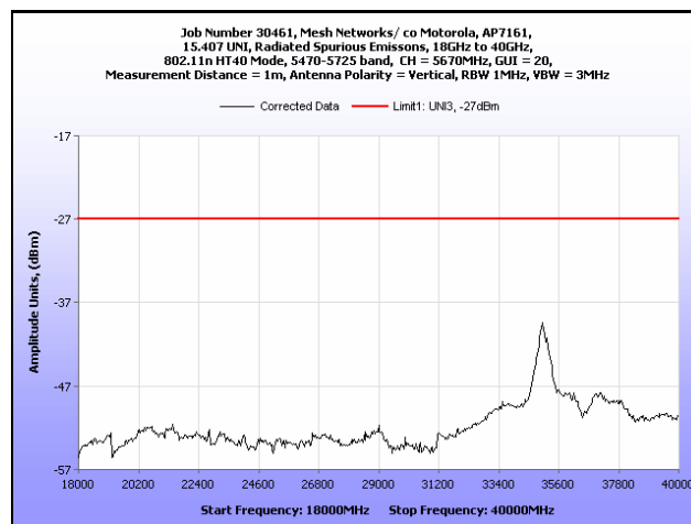
Plot 224. Radiated Spurious Emissions, 18 GHz – 40 GHz, 802.11n HT40, 5670 MHz
