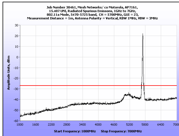
Plot 178. Radiated Spurious Emissions, 1 GHz – 7 GHz, 802.11a, 5700 MHz
