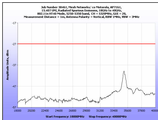
Plot 216. Radiated Spurious Emissions, 18 GHz – 40 GHz, 802.11n HT40, 5320 MHz
