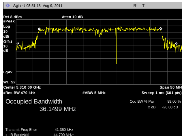
Plot 48. 26 dB Occupied Bandwidth, 802.11n HT40, 5310 MHz, R3-C
