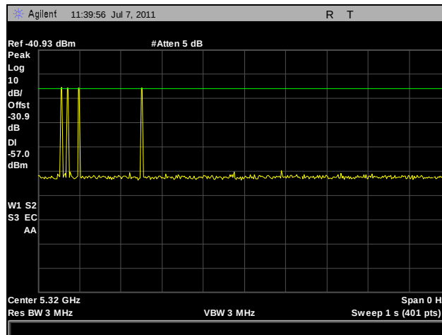
Plot 338. Bin 6 Radar Calibration for 5 dBi
