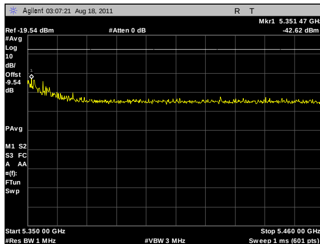
Plot 242. Radiated Band Edge, 802.11n HT40, 5320 MHz
