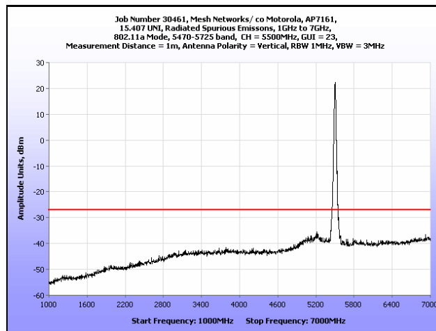
Plot 170. Radiated Spurious Emissions, 1 GHz – 7 GHz, 802.11a, 5500 MHz
