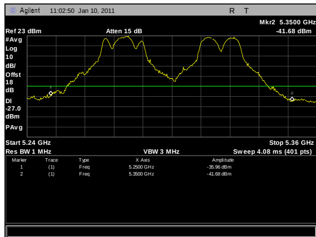
Plot 250. Frequency Stability, -40°C for 5250 MHz – 5350 MHz at 120 VAC
