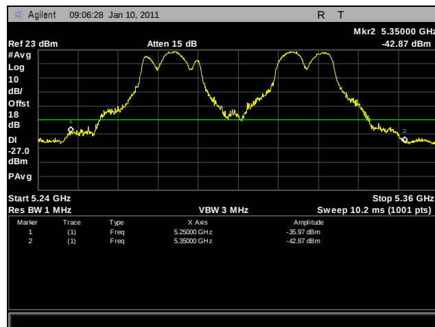
Plot 281. Frequency Stability, 60°C for 5250 MHz – 5350 MHz at 138 VAC
