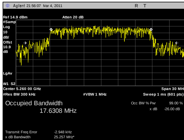
Plot 76. 99% Occupied Bandwidth, 802.11n HT20, 5260 MHz, R3-A
