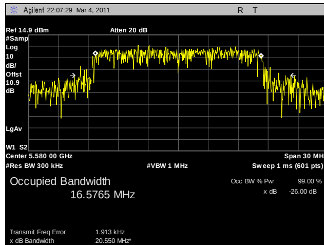
Plot 70. 99% Occupied Bandwidth, 802.11a, 5580 MHz, R3-A
