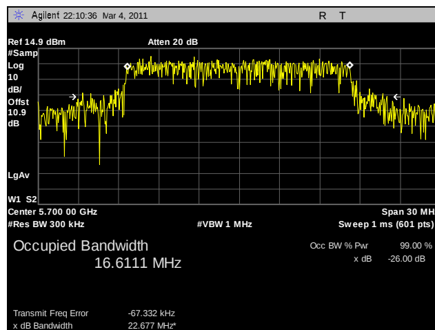
Plot 74. 99% Occupied Bandwidth, 802.11a, 5700 MHz, R3-B
