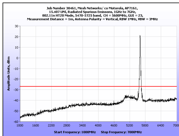
Plot 198. Radiated Spurious Emissions, 1 GHz – 7 GHz, 802.11n HT20, 5600 MHz
