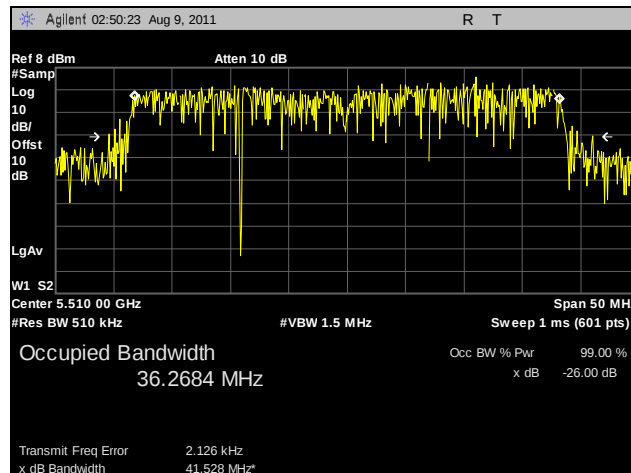
Plot 105. 99% Occupied Bandwidth, 802.11n HT40, 5510 MHz, R3-C
