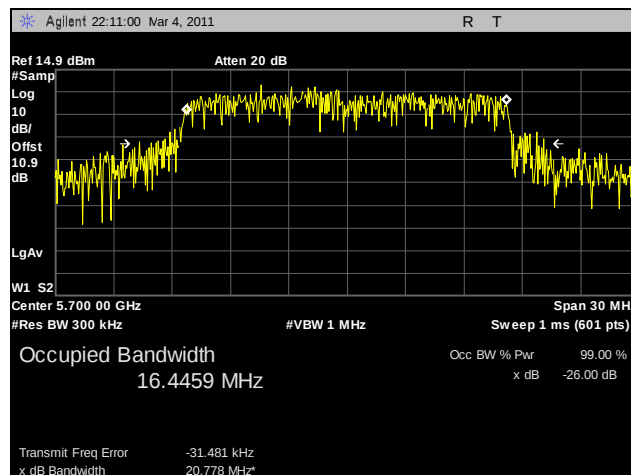
Plot 75. 99% Occupied Bandwidth, 802.11a, 5700 MHz, R3-C
