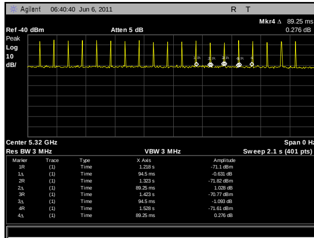
Plot 348. Channel Closing Transmission Time 4
