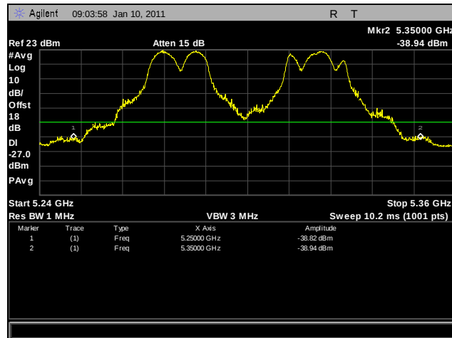
Plot 279. Frequency Stability, 60°C for 5250 MHz – 5350 MHz at 102 VAC
