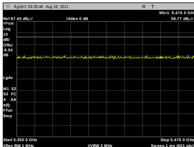
Plot 238. Radiated Restricted Band, 802.11n HT20, 5500 MHz, Peak
