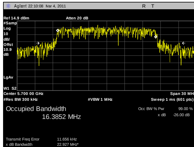
Plot 73. 99% Occupied Bandwidth, 802.11a, 5700 MHz, R3-A
