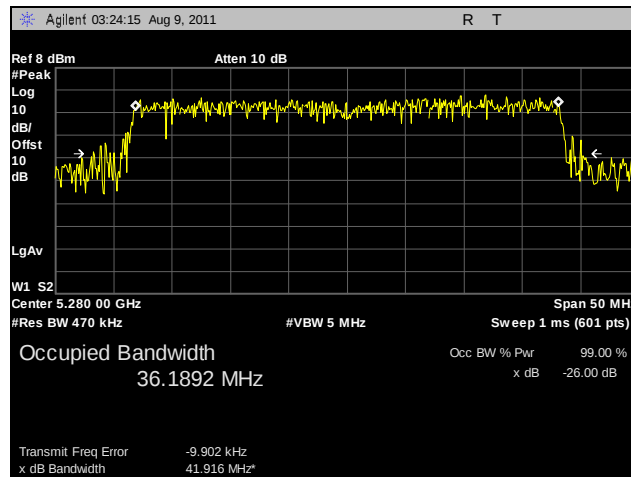
Plot 43. 26 dB Occupied Bandwidth, 802.11n HT40, 5280 MHz, R3-A
