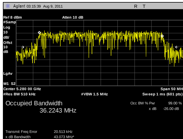
Plot 95. 99% Occupied Bandwidth, 802.11n HT40, 5280 MHz, R3-B
