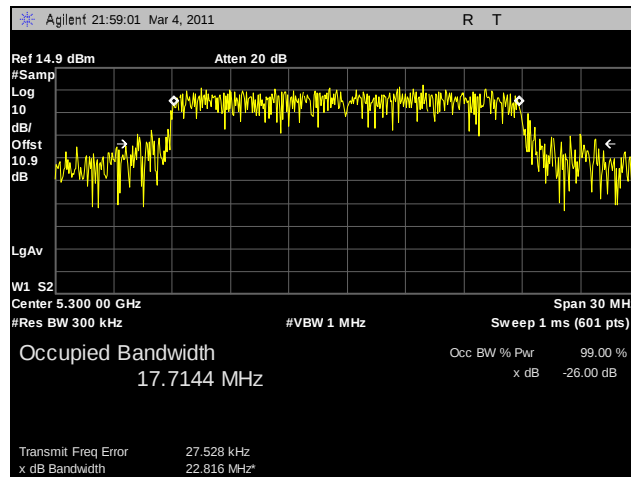
Plot 79. 99% Occupied Bandwidth, 802.11n HT20, 5300 MHz, R3-A
