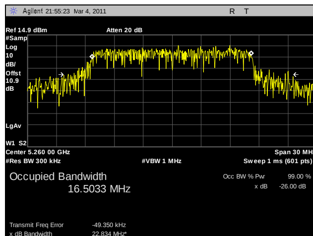
Plot 60. 99% Occupied Bandwidth, 802.11a, 5260 MHz, R3-C
