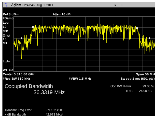
Plot 98. 99% Occupied Bandwidth, 802.11n HT40, 5310 MHz, R3-B
