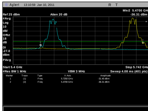
Plot 301. Frequency Stability, 10°C for 5470 MHz - 5725 MHz at 120 VAC
