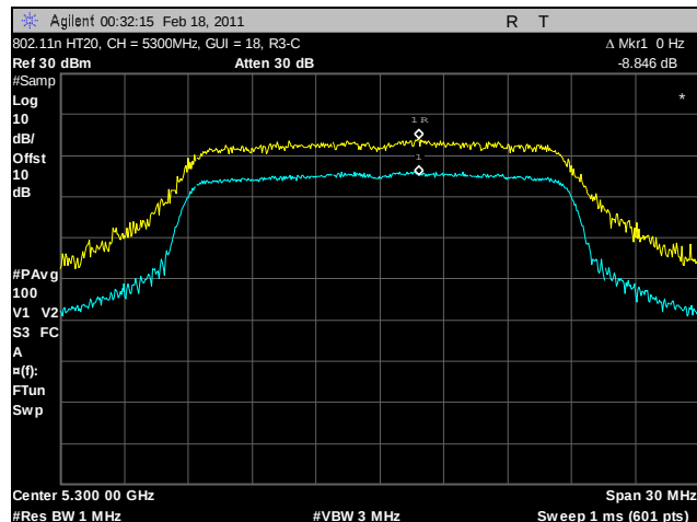
Plot 132. Peak Excursion Ratio, 802.11n HT20, 5300 MHz, R3-C
