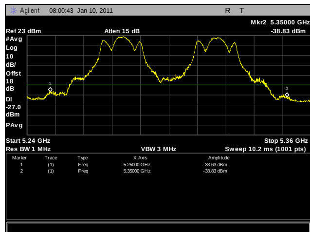
Plot 272. Frequency Stability, 30°C for 5250 MHz – 5350 MHz at 138 VAC
