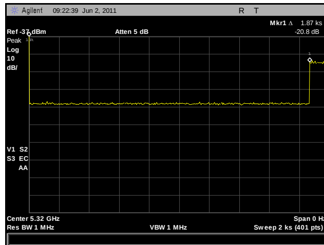
Plot 342. Non-Occupancy Period
