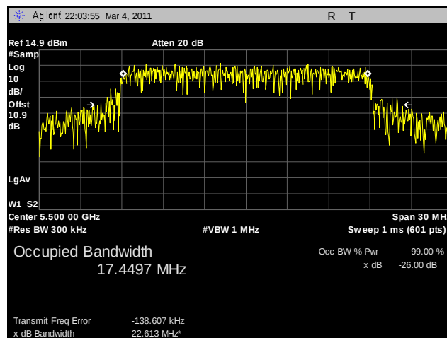
Plot 86. 99% Occupied Bandwidth, 802.11n HT20, 5500 MHz, R3-B
