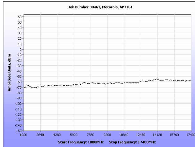
Plot 330. Receiver Spurious Emission, R3-B, 1 GHz - 17.4 GHz
