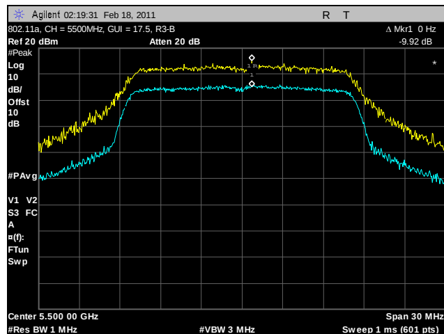
Plot 119. Peak Excursion Ratio, 802.11a, 5500 MHz, R3-B
