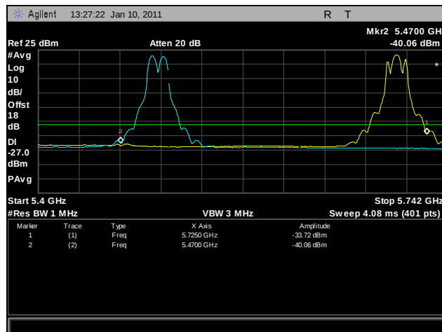
Plot 295. Frequency Stability, -10°C for 5470 MHz - 5725 MHz at 120 VAC
