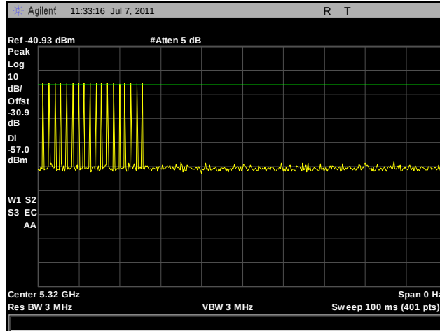
Plot 333. Bin 1 Radar Calibration for 5 dBi
