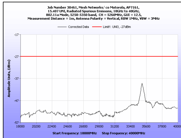
Plot 160. Radiated Spurious Emissions, 18 GHz – 40 GHz, 802.11a, 5260 MHz
