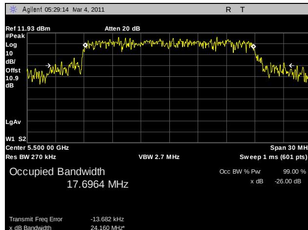
Plot 36. 26 dB Occupied Bandwidth, 802.11n HT20, 5500 MHz, R3-C
