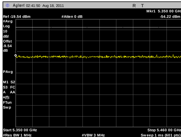
Plot 226. Radiated Band Edge, 802.11a, 5320 MHz
