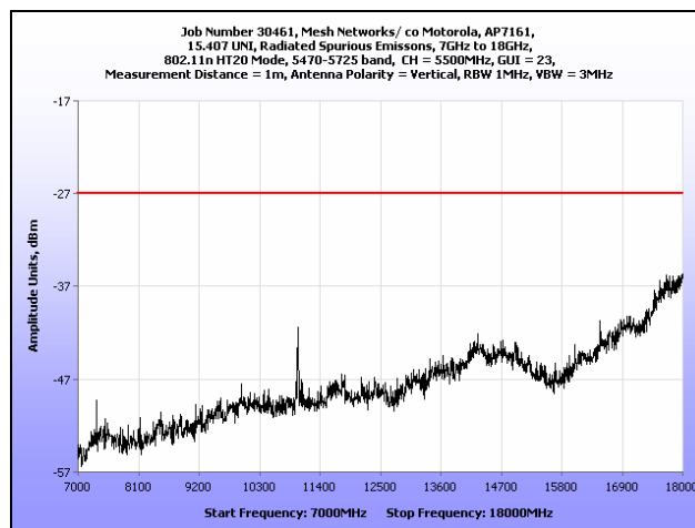
Plot 195. Radiated Spurious Emissions, 7 GHz – 18 GHz, 802.11n HT20, 5500 MHz
