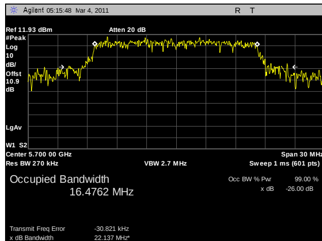
Plot 23. 26 dB Occupied Bandwidth, 802.11a, 5700 MHz, R3-B
