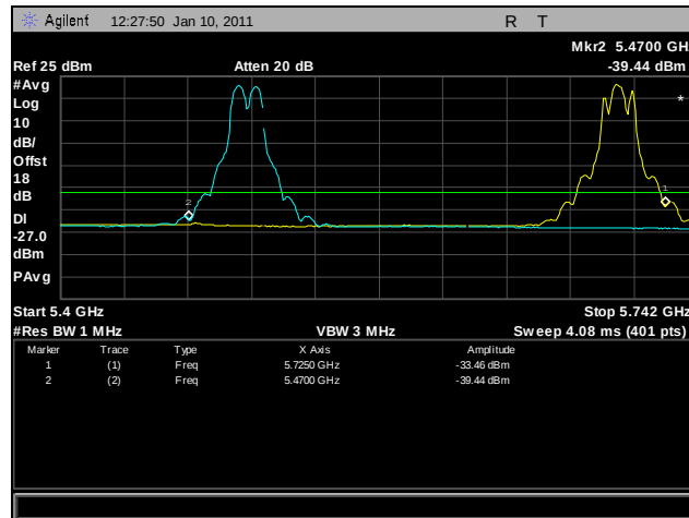
Plot 312. Frequency Stability, 50°C for 5470 MHz - 5725 MHz at 102 VAC
