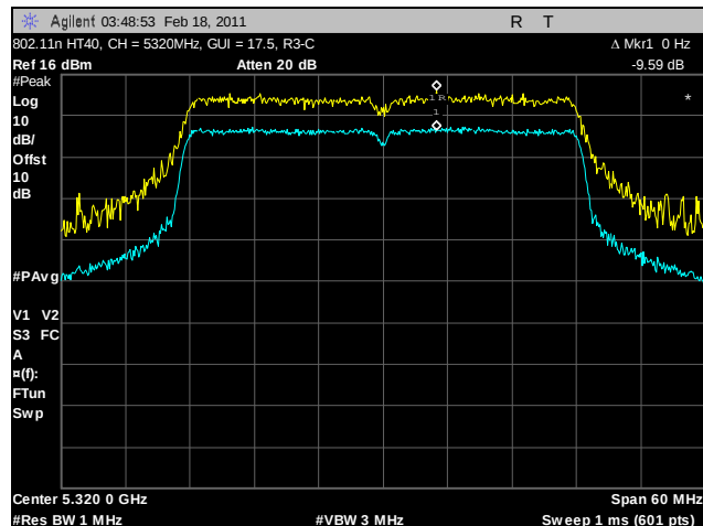
Plot 150. Peak Excursion Ratio, 802.11n HT40, 5320 MHz, R3-C
