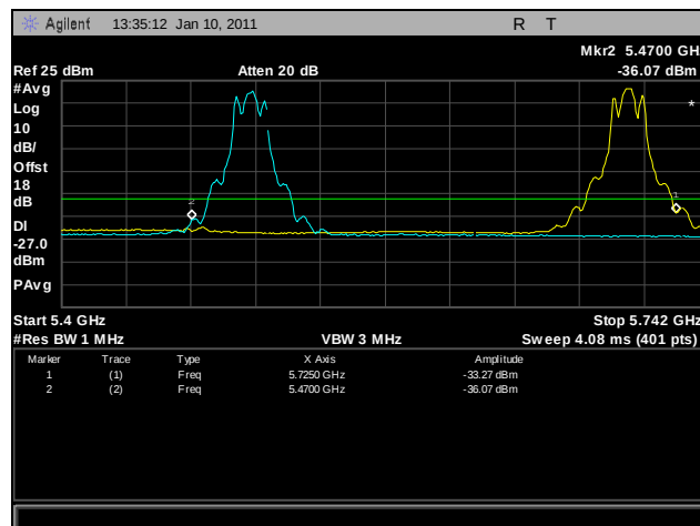
Plot 293. Frequency Stability, -20°C for 5470 MHz - 5725 MHz at 138 VAC
