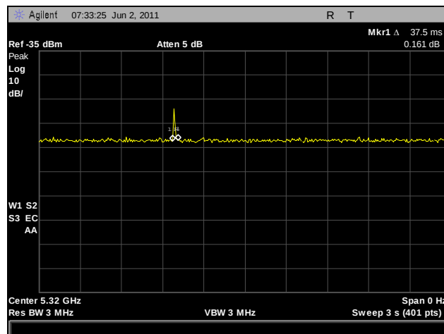
Plot 350. Channel Closing Transmission Time 6
