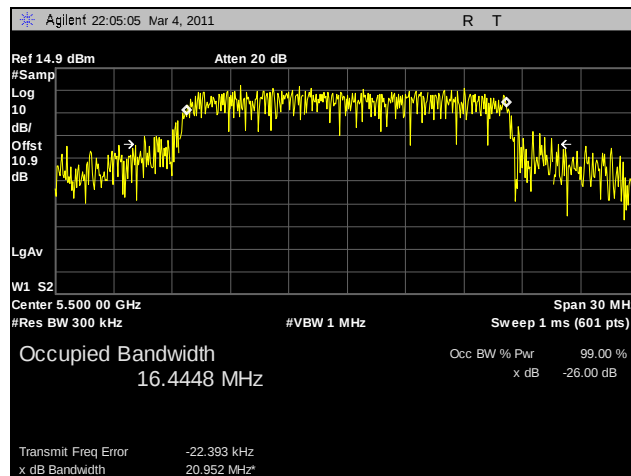
Plot 68. 99% Occupied Bandwidth, 802.11a, 5500 MHz, R3-B
