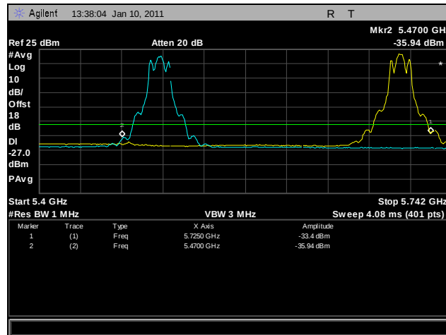
Plot 291. Frequency Stability, -20°C for 5470 MHz - 5725 MHz at 102 VAC
