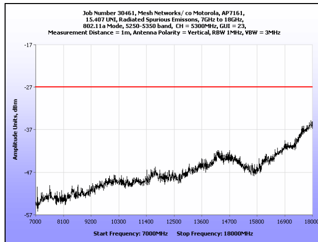
Plot 163. Radiated Spurious Emissions, 7 GHz – 18 GHz, 802.11a, 5300 MHz
