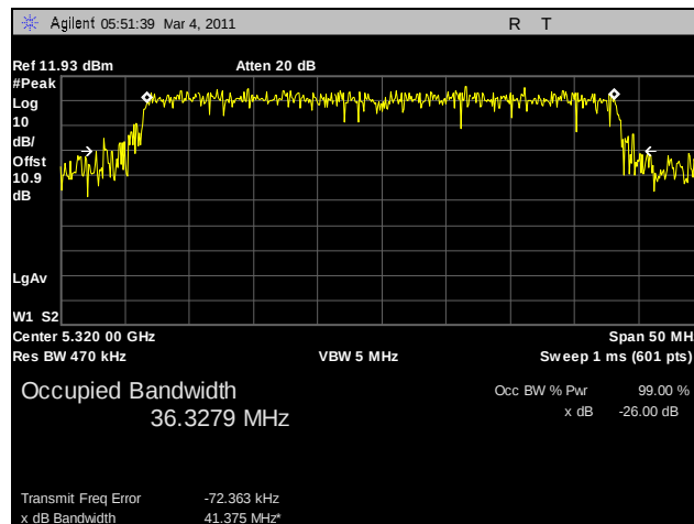
Plot 50. 26 dB Occupied Bandwidth, 802.11n HT40, 5320 MHz, R3-B
