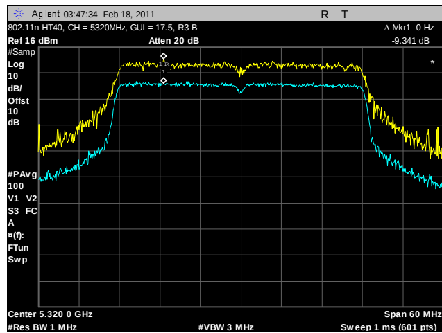
Plot 149. Peak Excursion Ratio, 802.11n HT40, 5320 MHz, R3-B
