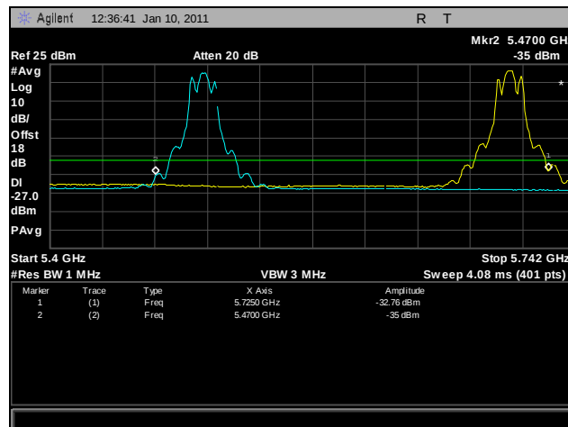
Plot 316. Frequency Stability, 60°C for 5470 MHz - 5725 MHz at 120 VAC
