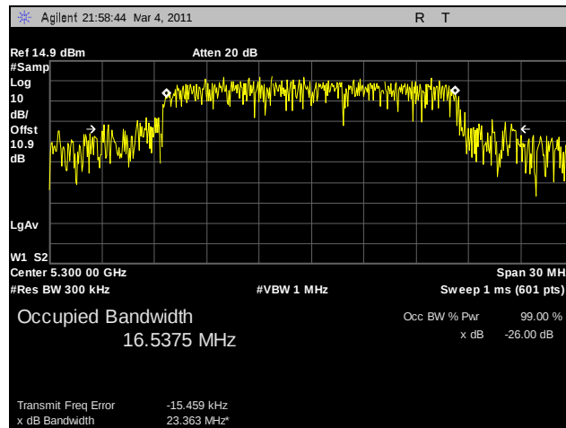
Plot 61. 99% Occupied Bandwidth, 802.11a, 5300 MHz, R3-A
