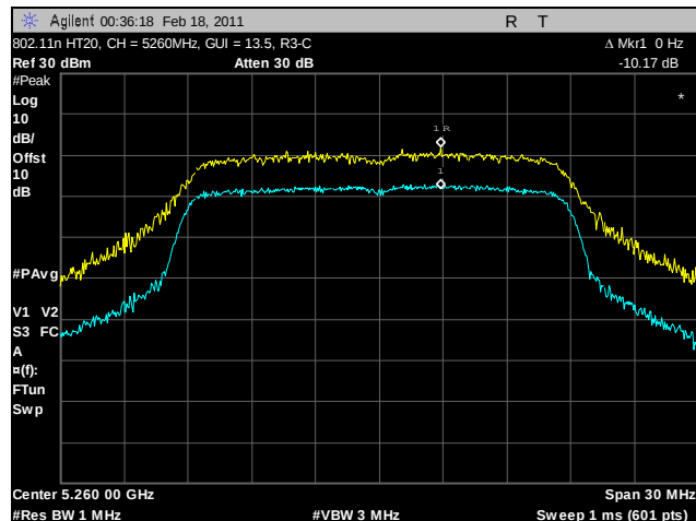
Plot 129. Peak Excursion Ratio, 802.11n HT20, 5260 MHz, R3-C
