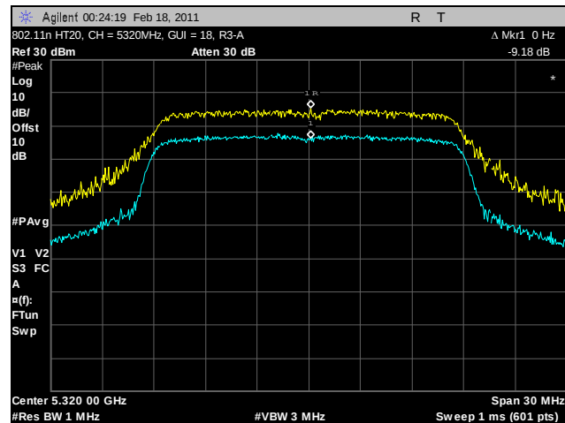
Plot 133. Peak Excursion Ratio, 802.11n HT20, 5320 MHz, R3-A
