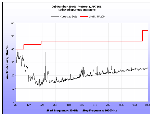
Plot 221. Radiated Spurious Emissions, 30 MHz – 1 GHz, 802.11n HT40, 5670 MHz
