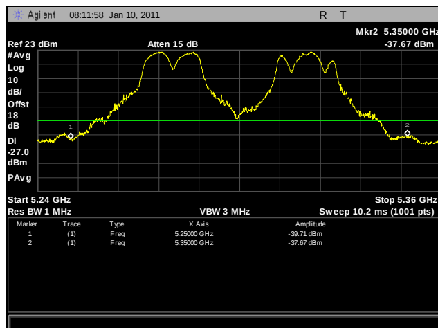
Plot 275. Frequency Stability, 40°C for 5250 MHz – 5350 MHz at 138 VAC
