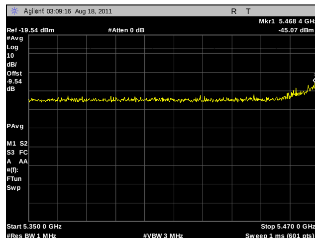
Plot 245. Radiated Band Edge, 802.11n HT40, 5510 MHz
