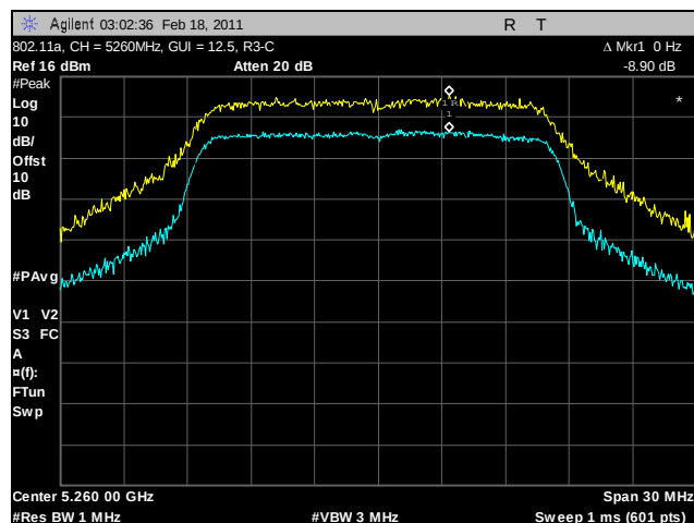
Plot 111. Peak Excursion Ratio, 802.11a, 5260 MHz, R3-C
