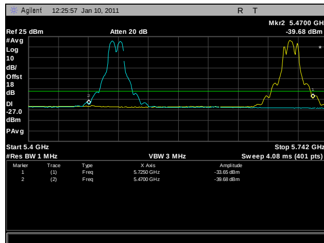
Plot 313. Frequency Stability, 50°C for 5470 MHz - 5725 MHz at 120 VAC
