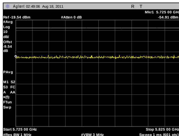
Plot 240. Radiated Band Edge, 802.11n HT20, 5700 MHz
