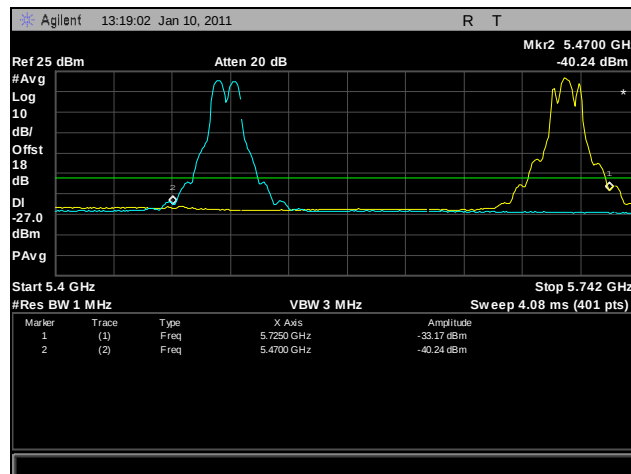
Plot 298. Frequency Stability, 0°C for 5470 MHz - 5725 MHz at 120 VAC
