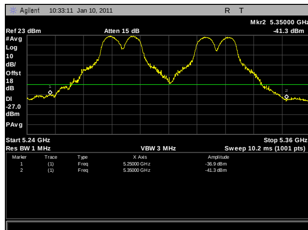
Plot 257. Frequency Stability, -20°C for 5250 MHz – 5350 MHz at 138 VAC
