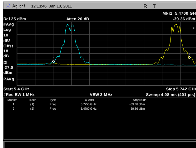
Plot 309. Frequency Stability, 40°C for 5470 MHz - 5725 MHz at 102 VAC
