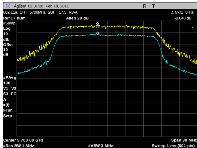
Plot 124. Peak Excursion Ratio, 802.11a, 5700 MHz, R3-A
