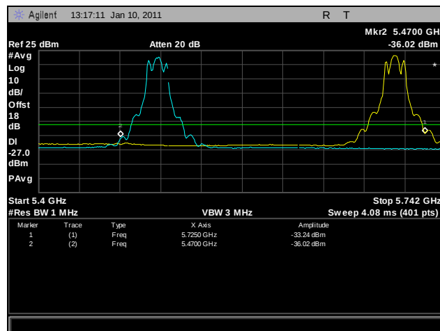
Plot 299. Frequency Stability, 0°C for 5470 MHz - 5725 MHz at 138 VAC
