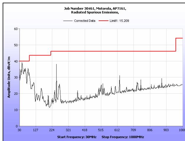
Plot 177. Radiated Spurious Emissions, 30 MHz – 1 GHz, 802.11a, 5700 MHz
