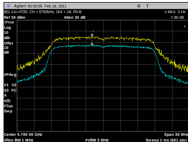
Plot 143. Peak Excursion Ratio, 802.11n HT20, 5700 MHz, R3-B
