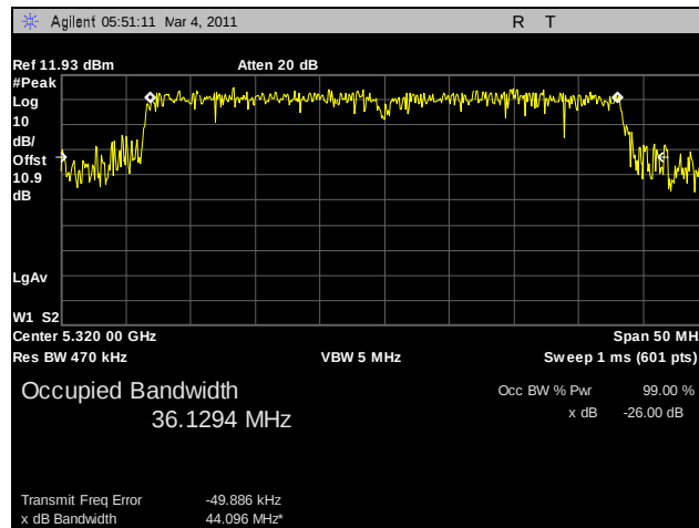
Plot 49. 26 dB Occupied Bandwidth, 802.11n HT40, 5320 MHz, R3-A
