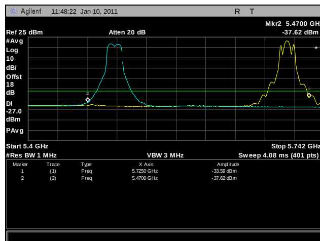
Plot 304. Frequency Stability, 20°C for 5470 MHz - 5725 MHz at 120 VAC
