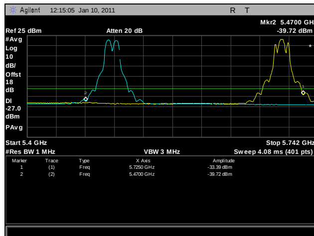
Plot 310. Frequency Stability, 40°C for 5470 MHz - 5725 MHz at 120 VAC
