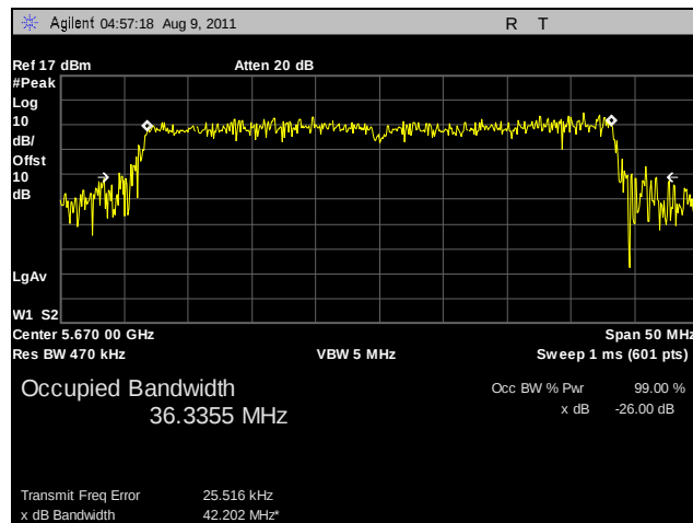
Plot 56. 26 dB Occupied Bandwidth, 802.11n HT40, 5670 MHz, R3-B
