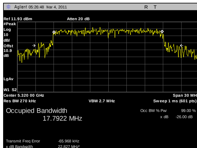
Plot 33. 26 dB Occupied Bandwidth, 802.11n HT20, 5320 MHz, R3-C
