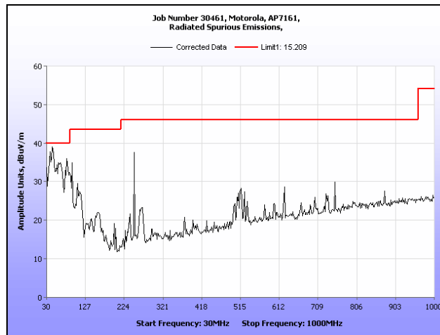
Plot 205. Radiated Spurious Emissions, 30 MHz – 1 GHz, 802.11n HT40, 5280 MHz
