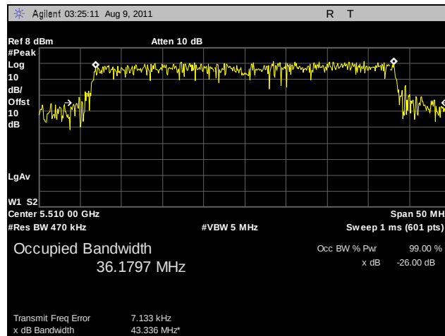
Plot 52. 26 dB Occupied Bandwidth, 802.11n HT40, 5510 MHz, R3-A
