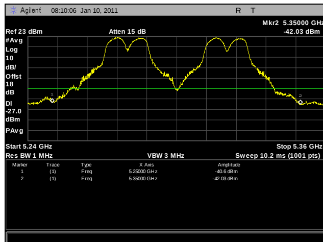
Plot 274. Frequency Stability, 40°C for 5250 MHz – 5350 MHz at 120 VAC
