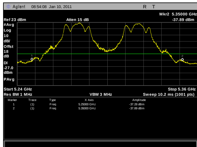
Plot 278. Frequency Stability, 50°C for 5250 MHz – 5350 MHz at 138 VAC
