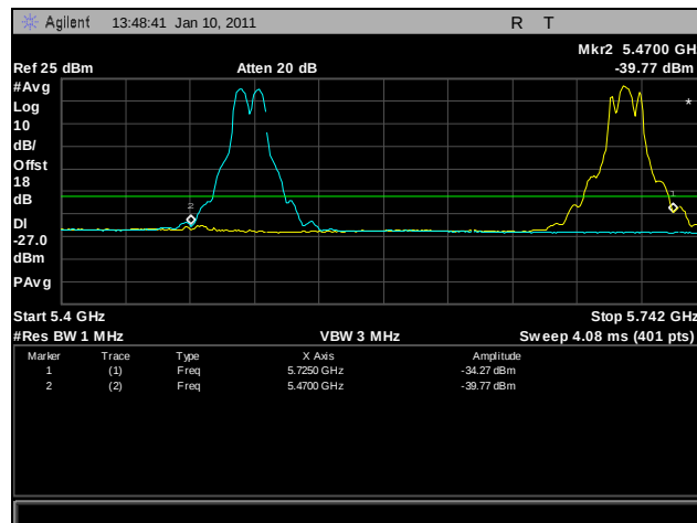
Plot 289. Frequency Stability, -30°C for 5470 MHz - 5725 MHz at 120 VAC
