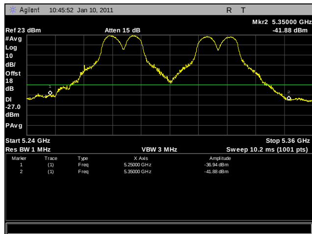
Plot 253. Frequency Stability, -30°C for 5250 MHz – 5350 MHz at 120 VAC
