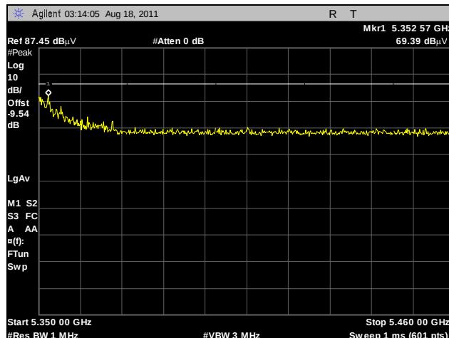
Plot 243. Radiated Restricted Band, 802.11n HT40, 5320 MHz, Peak
