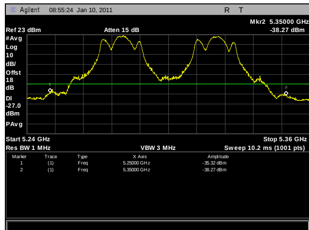
Plot 277. Frequency Stability, 50°C for 5250 MHz – 5350 MHz at 120 VAC
