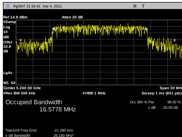
Plot 59. 99% Occupied Bandwidth, 802.11a, 5260 MHz, R3-B
