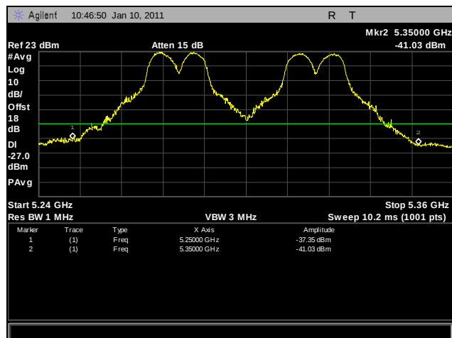
Plot 254. Frequency Stability, -30°C for 5250 MHz – 5350 MHz at 138 VAC
