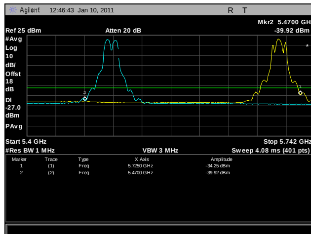
Plot 319. Frequency Stability, 70°C for 5470 MHz - 5725 MHz at 120 VAC
