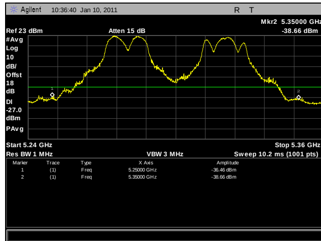
Plot 255. Frequency Stability, -20°C for 5250 MHz – 5350 MHz at 102 VAC
