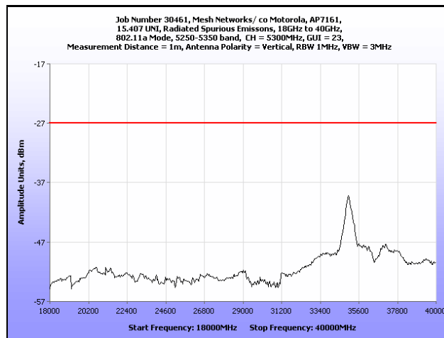
Plot 164. Radiated Spurious Emissions, 18 GHz – 40 GHz, 802.11a, 5300 MHz
