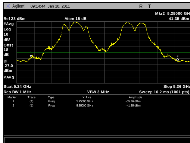
Plot 283. Frequency Stability, 70°C for 5250 MHz – 5350 MHz at 120 VAC
