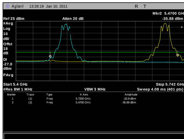
Plot 296. Frequency Stability, -10°C for 5470 MHz - 5725 MHz at 138 VAC
