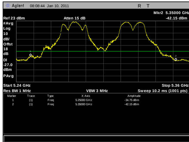
Plot 273. Frequency Stability, 40°C for 5250 MHz – 5350 MHz at 102 VAC
