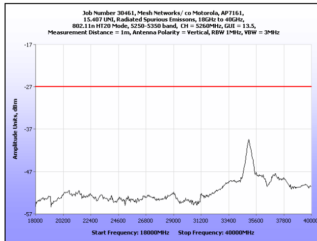
Plot 184. Radiated Spurious Emissions, 18 GHz – 40 GHz, 802.11n HT20, 5260 MHz
