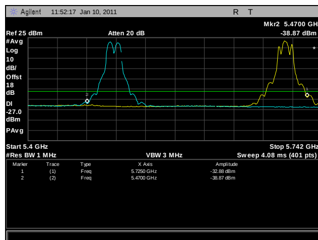
Plot 305. Frequency Stability, 20°C for 5470 MHz - 5725 MHz at 138 VAC
