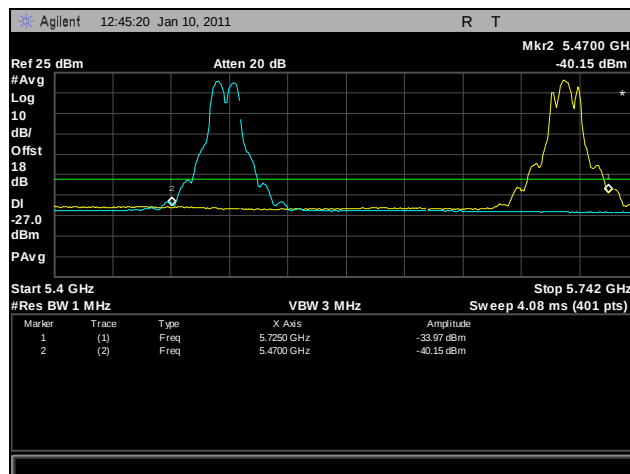
Plot 320. Frequency Stability, 70°C for 5470 MHz - 5725 MHz at 138 VAC
