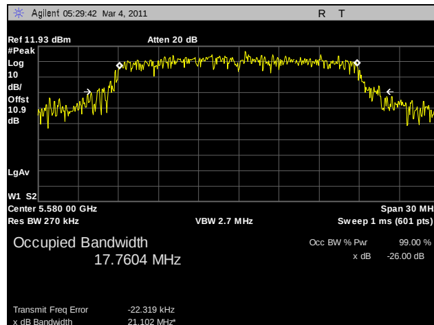
Plot 39. 26 dB Occupied Bandwidth, 802.11n HT20, 5580 MHz, R3-C
