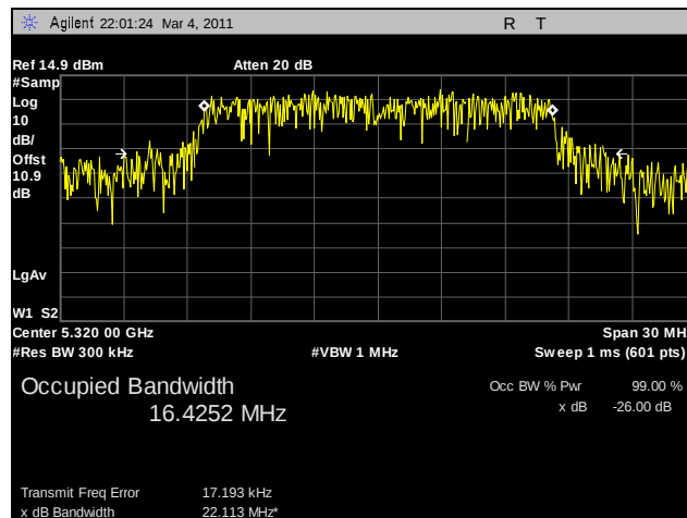
Plot 65. 99% Occupied Bandwidth, 802.11a, 5320 MHz, R3-B
