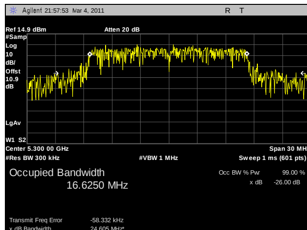
Plot 63. 99% Occupied Bandwidth, 802.11a, 5300 MHz, R3-C
