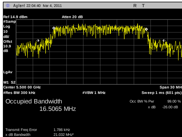
Plot 67. 99% Occupied Bandwidth, 802.11a, 5500 MHz, R3-A
