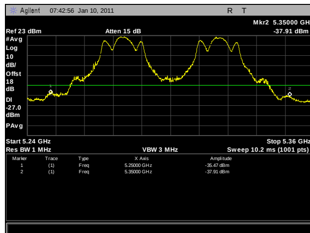
Plot 269. Frequency Stability, 20°C for 5250 MHz – 5350 MHz at 138 VAC
