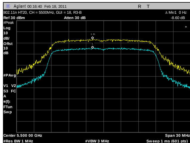
Plot 137. Peak Excursion Ratio, 802.11n HT20, 5500 MHz, R3-B
