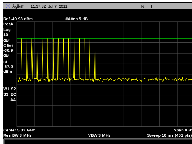
Plot 335. Bin 3 Radar Calibration for 5 dBi
