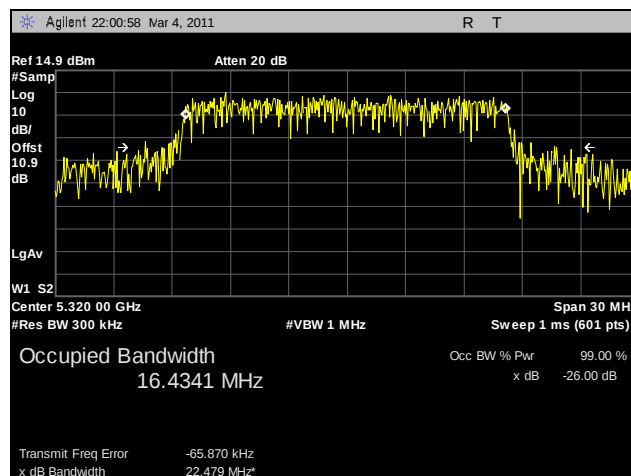
Plot 66. 99% Occupied Bandwidth, 802.11a, 5320 MHz, R3-C
