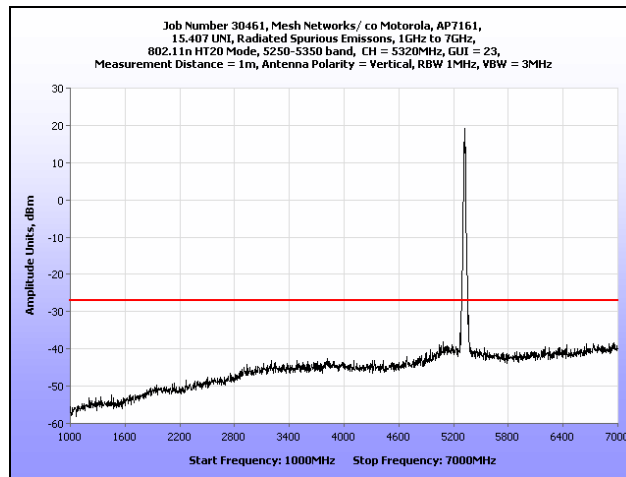
Plot 190. Radiated Spurious Emissions, 1 GHz – 7 GHz, 802.11n HT20, 5320 MHz
