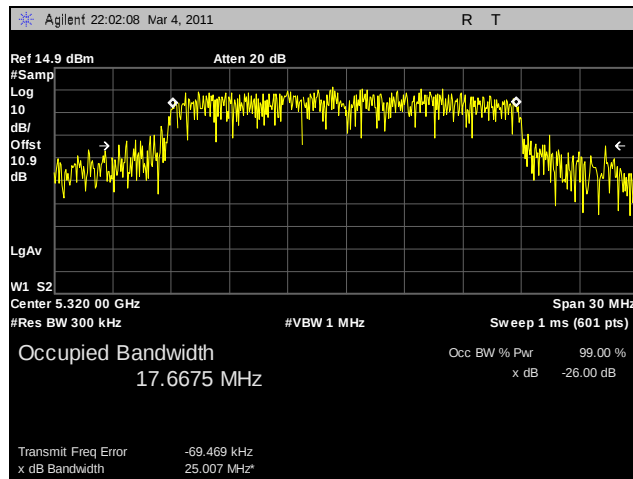
Plot 82. 99% Occupied Bandwidth, 802.11n HT20, 5320 MHz, R3-A
