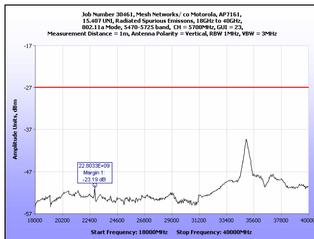
Plot 180. Radiated Spurious Emissions, 18 GHz – 40 GHz, 802.11a, 5700 MHz
