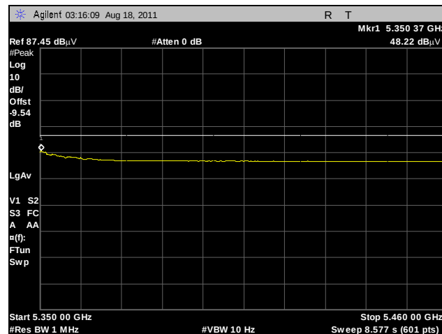
Plot 244. Radiated Restricted Band, 802.11n HT40, 5320 MHz, Average
