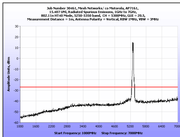
Plot 210. Radiated Spurious Emissions, 1 GHz – 7 GHz, 802.11n HT40, 5300 MHz
