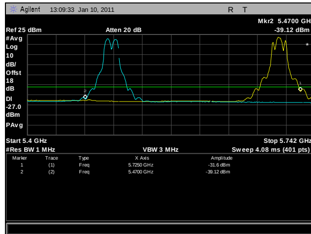
Plot 300. Frequency Stability, 10°C for 5470 MHz - 5725 MHz at 102 VAC
