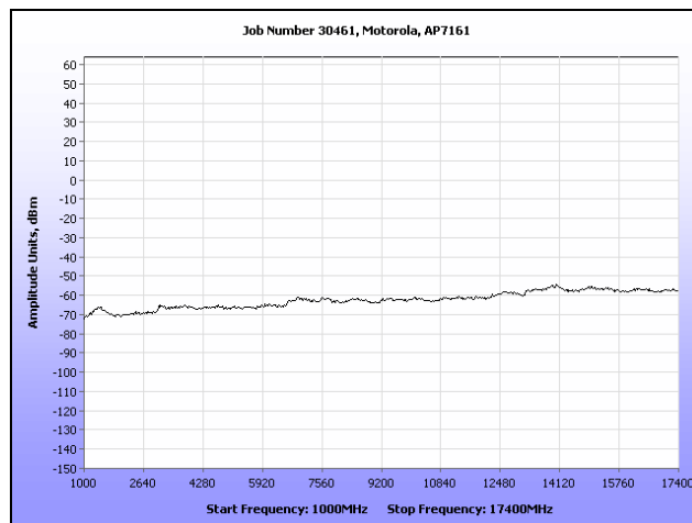
Plot 332. Receiver Spurious Emission, R3-C, 1 GHz - 17.4 GHz
