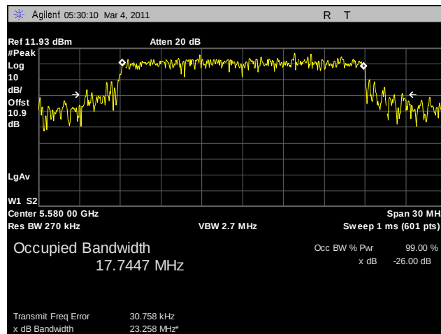
Plot 38. 26 dB Occupied Bandwidth, 802.11n HT20, 5580 MHz, R3-B
