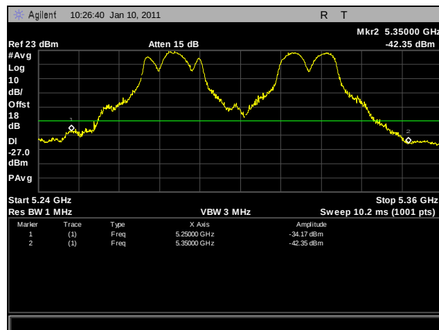
Plot 260. Frequency Stability, -10°C for 5250 MHz – 5350 MHz at 138 VAC
