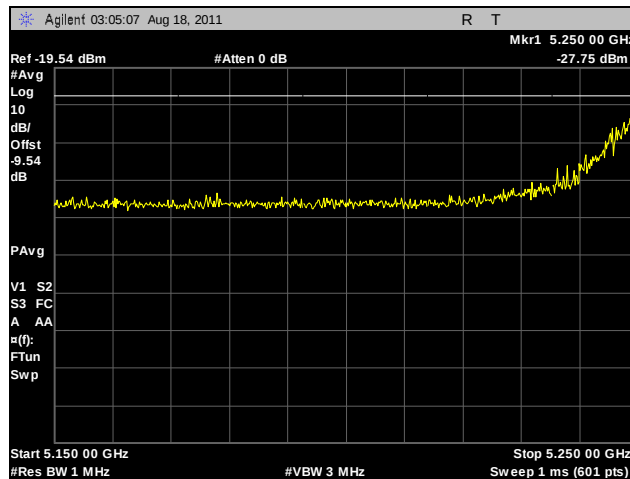
Plot 241. Radiated Band Edge, 802.11n HT40, 5270 MHz
