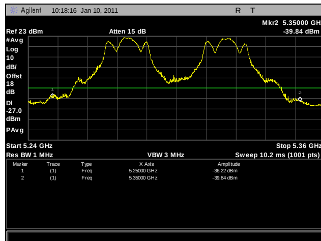
Plot 262. Frequency Stability, 0°C for 5250 MHz – 5350 MHz at 120 VAC
