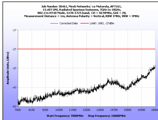
Plot 223. Radiated Spurious Emissions, 7 GHz – 18 GHz, 802.11n HT40, 5670 MHz
