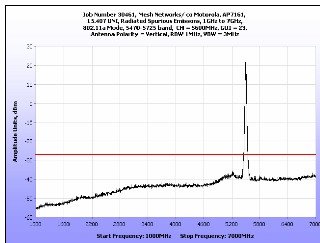
Plot 174. Radiated Spurious Emissions, 1 GHz – 7 GHz, 802.11a, 5600 MHz
