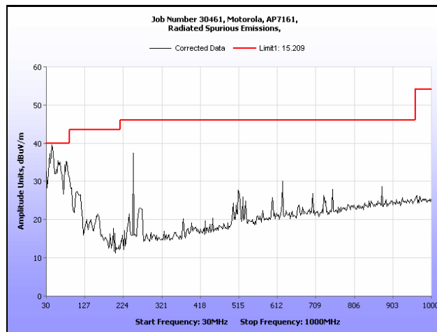
Plot 173. Radiated Spurious Emissions, 30 MHz – 1 GHz, 802.11a, 5580 MHz
