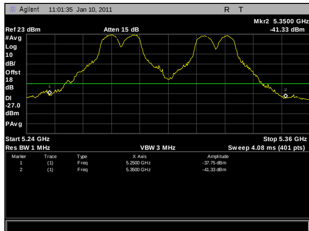
Plot 251. Frequency Stability, -40°C for 5250 MHz – 5350 MHz at 138 VAC
