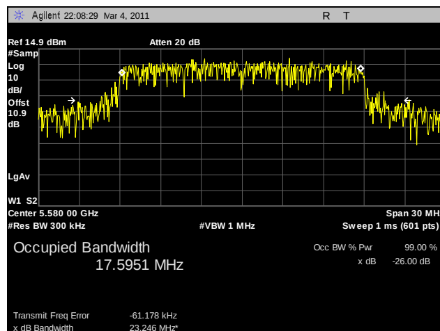
Plot 90. 99% Occupied Bandwidth, 802.11n HT20, 5580 MHz, R3-C
