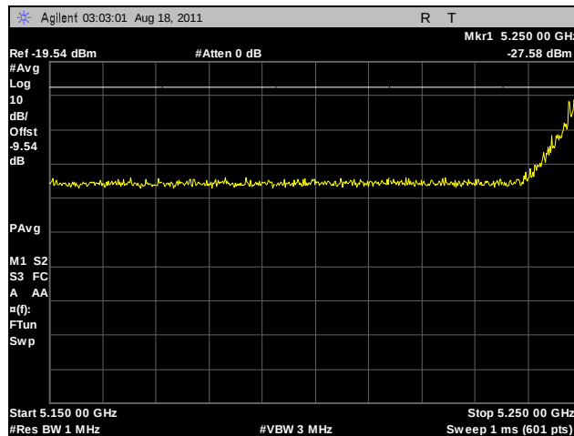
Plot 233. Radiated Band Edge, 802.11n HT20, 5260 MHz
