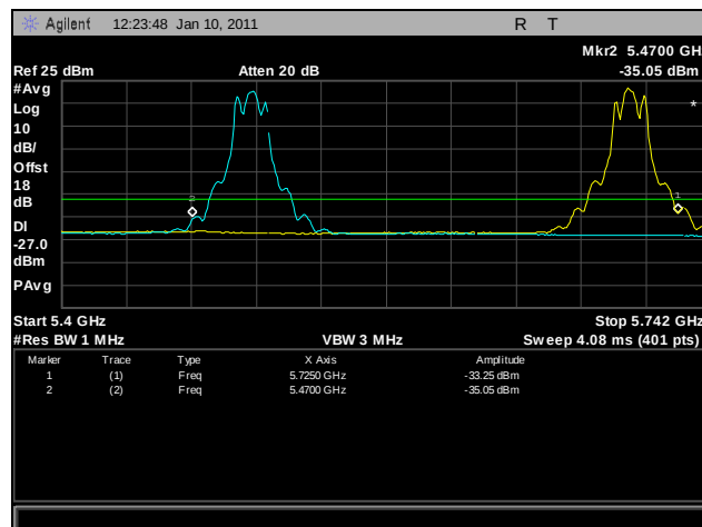
Plot 314. Frequency Stability, 50°C for 5470 MHz - 5725 MHz at 138 VAC
