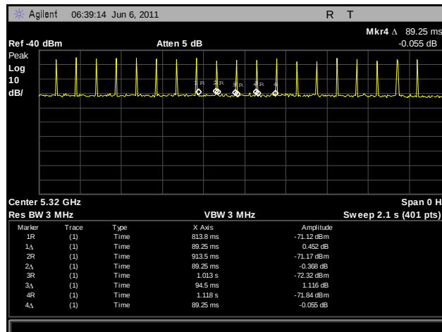
Plot 347. Channel Closing Transmission Time 3
