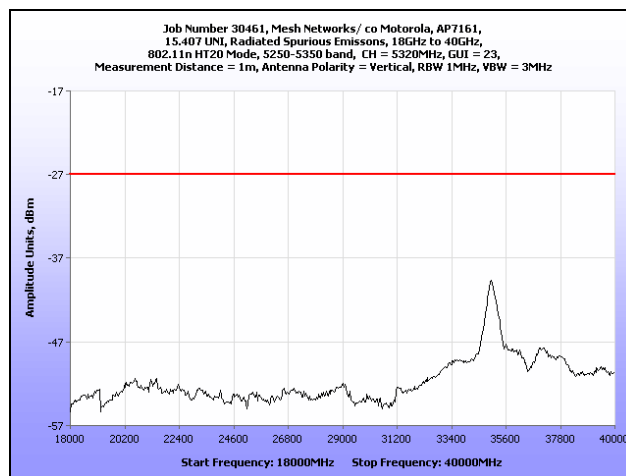
Plot 192. Radiated Spurious Emissions, 18 GHz – 40 GHz, 802.11n HT20, 5320 MHz
