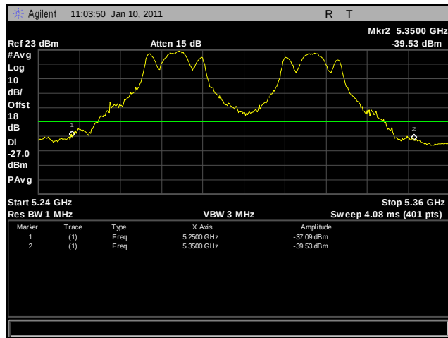
Plot 249. Frequency Stability, -40°C for 5250 MHz – 5350 MHz at 102 VAC
