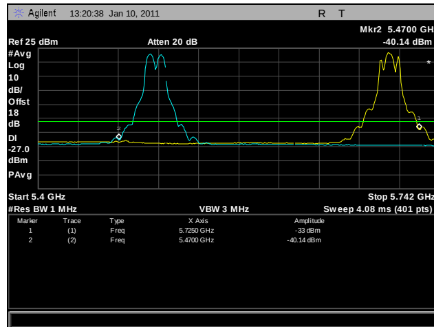
Plot 297. Frequency Stability, 0°C for 5470 MHz - 5725 MHz at 102 VAC
