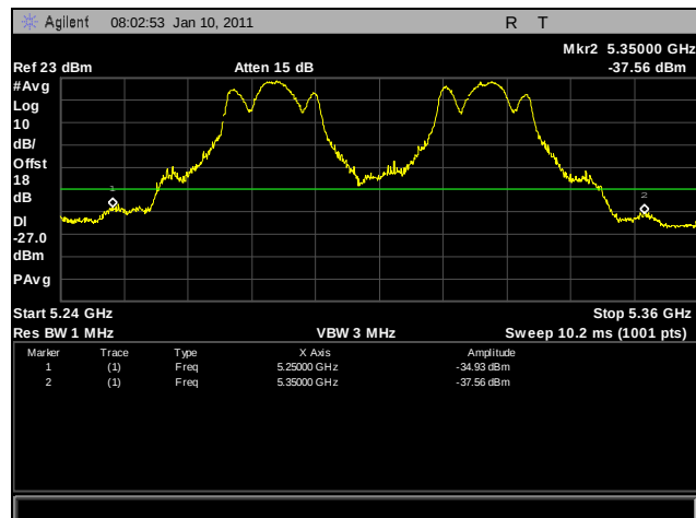
Plot 271. Frequency Stability, 30°C for 5250 MHz – 5350 MHz at 120 VAC
