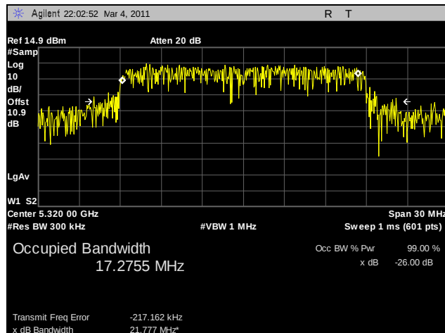
Plot 84. 99% Occupied Bandwidth, 802.11n HT20, 5320 MHz, R3-C
