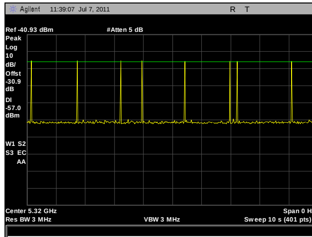
Plot 337. Bin 5 Radar Calibration for 5 dBi
