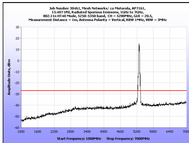
Plot 206. Radiated Spurious Emissions, 1 GHz – 7 GHz, 802.11n HT40, 5280 MHz
