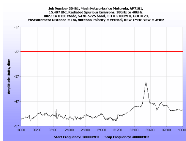
Plot 204. Radiated Spurious Emissions, 18 GHz – 40 GHz, 802.11n HT20, 5700 MHz
