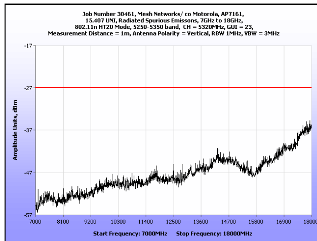
Plot 191. Radiated Spurious Emissions, 7 GHz – 18 GHz, 802.11n HT20, 5320 MHz
