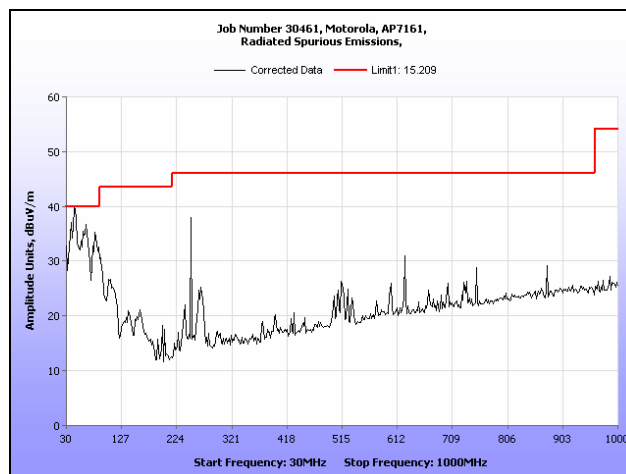
Plot 201. Radiated Spurious Emissions, 30 MHz – 1 GHz, 802.11n HT20, 5700 MHz
