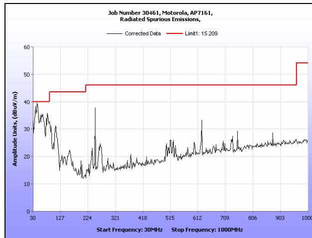
Plot 181. Radiated Spurious Emissions, 30 MHz – 1 GHz, 802.11n HT20, 5260 MHz
