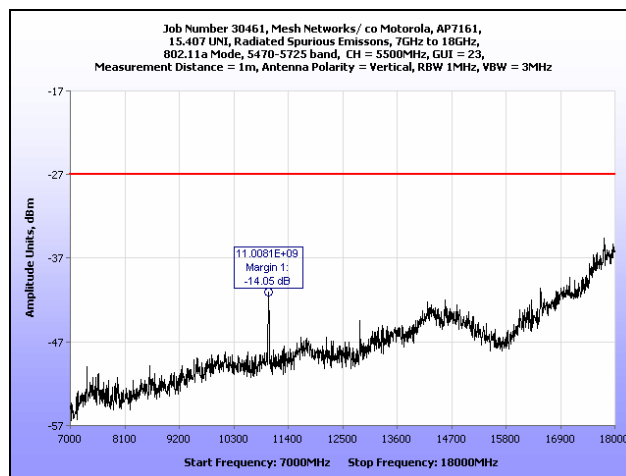
Plot 171. Radiated Spurious Emissions, 7 GHz – 18 GHz, 802.11a, 5500 MHz
