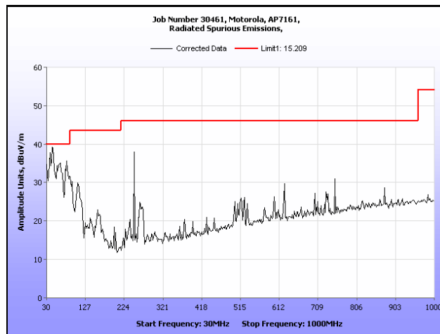
Plot 185. Radiated Spurious Emissions, 30 MHz – 1 GHz, 802.11n HT20, 5300 MHz
