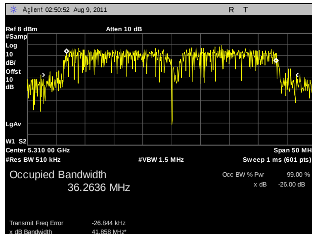
Plot 99. 99% Occupied Bandwidth, 802.11n HT40, 5310 MHz, R3-C
