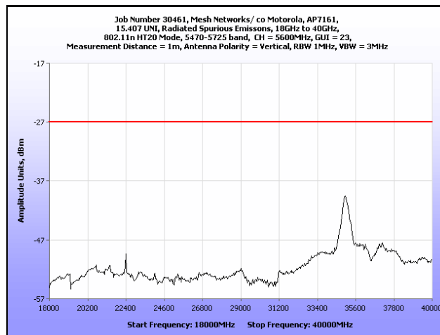
Plot 200. Radiated Spurious Emissions, 18 GHz – 40 GHz, 802.11n HT20, 5600 MHz
