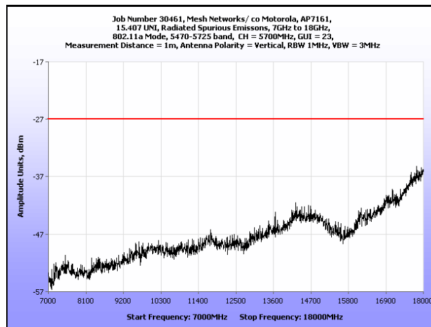
Plot 179. Radiated Spurious Emissions, 7 GHz – 18 GHz, 802.11a, 5700 MHz
