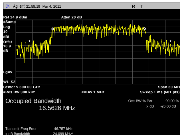
Plot 62. 99% Occupied Bandwidth, 802.11a, 5300 MHz, R3-B
