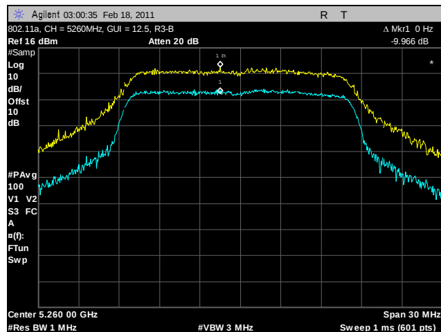
Plot 110. Peak Excursion Ratio, 802.11a, 5260 MHz, R3-B
