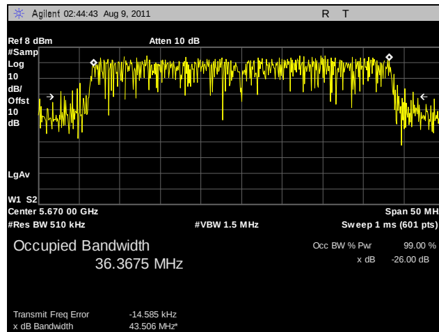
Plot 106. 99% Occupied Bandwidth, 802.11n HT40, 5670 MHz, R3-A
