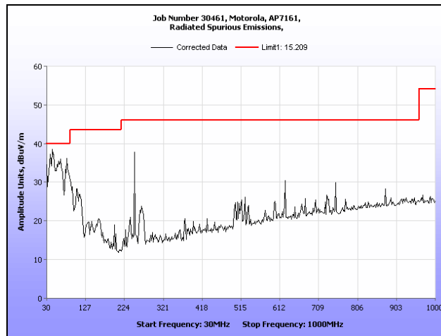
Plot 169. Radiated Spurious Emissions, 30 MHz – 1 GHz, 802.11a, 5500 MHz
