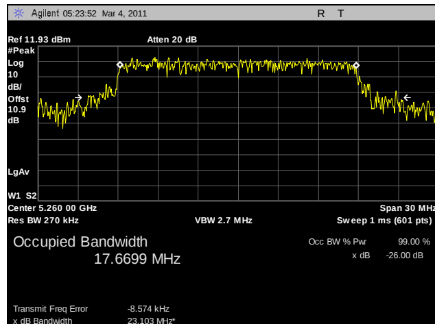
Plot 27. 26 dB Occupied Bandwidth, 802.11n HT20, 5260 MHz, R3-C
