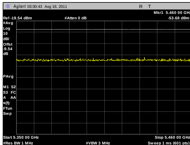
Plot 234. Radiated Band Edge, 802.11n HT20, 5320 MHz
