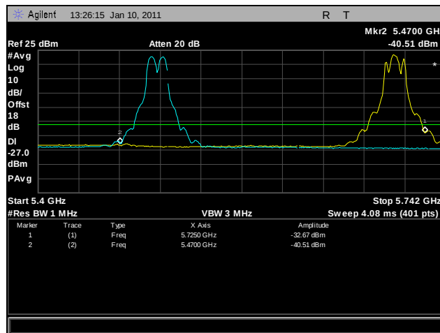
Plot 294. Frequency Stability, -10°C for 5470 MHz - 5725 MHz at 102 VAC
