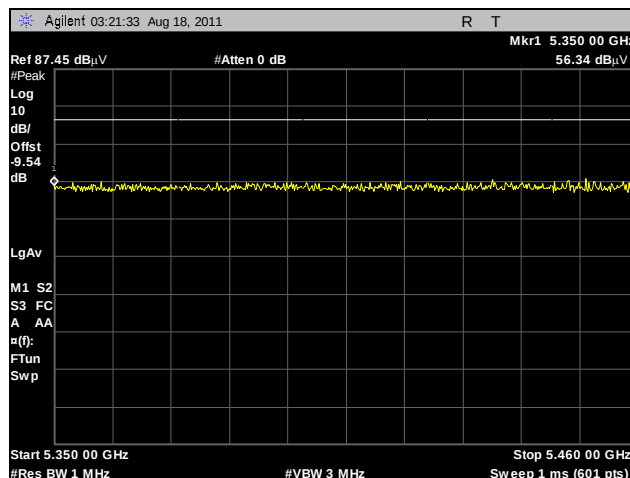
Plot 227. Radiated Restricted Band, 802.11a, 5320 MHz, Peak
