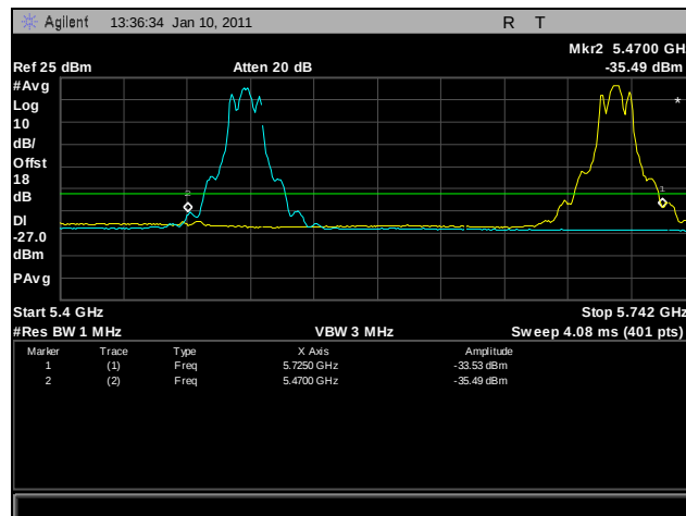
Plot 292. Frequency Stability, -20°C for 5470 MHz - 5725 MHz at 120 VAC
