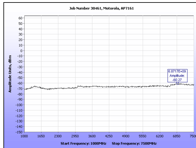
Plot 322. Receiver Spurious Emission, R3-A, 1 GHz - 7.5 GHz
