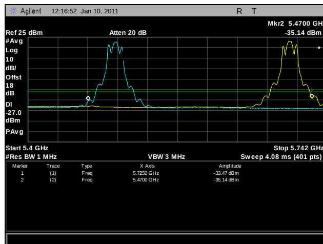
Plot 311. Frequency Stability, 40°C for 5470 MHz - 5725 MHz at 139 VAC
