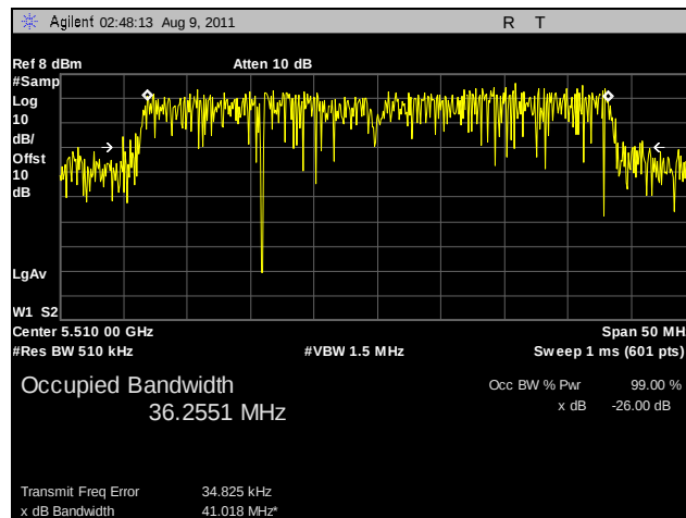
Plot 104. 99% Occupied Bandwidth, 802.11n HT40, 5510 MHz, R3-B
