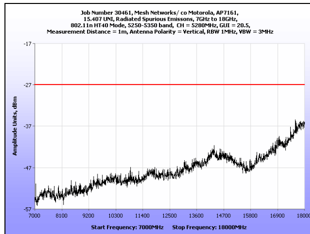
Plot 207. Radiated Spurious Emissions, 7 GHz – 18 GHz, 802.11n HT40, 5280 MHz
