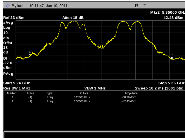
Plot 264. Frequency Stability, 10°C for 5250 MHz – 5350 MHz at 102 VAC
