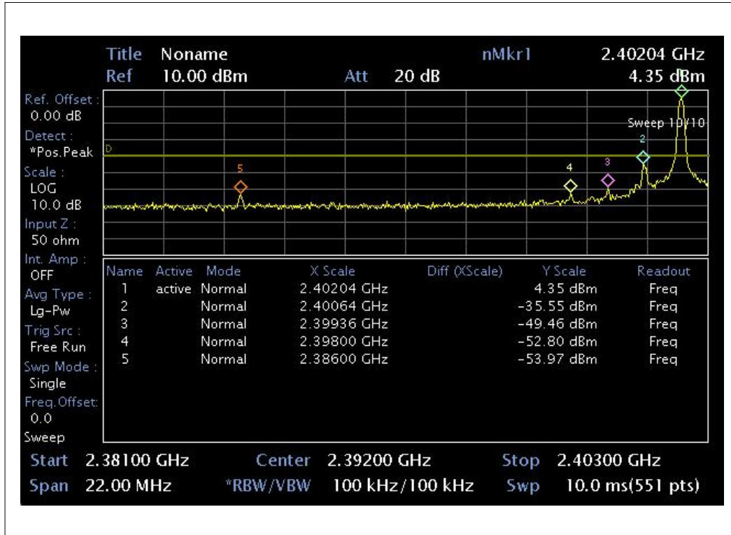
Figure 6. Plot of the Band Edge
