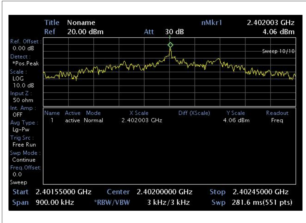
Figure 10. Plot of the Peak Power Spectral Density
