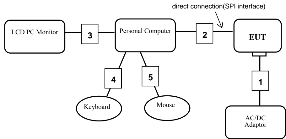
[ System Block Diagram of Test Configuration ]
