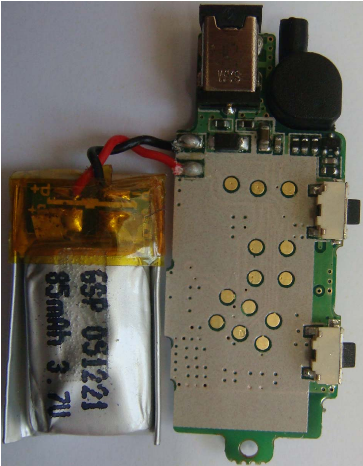
<Photograph 3: Internal Board Rear>
