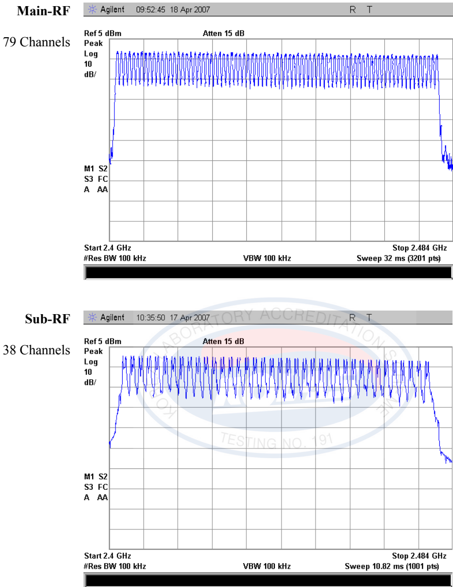
Figure 4: Number of Hopping Channels (Conducted)
