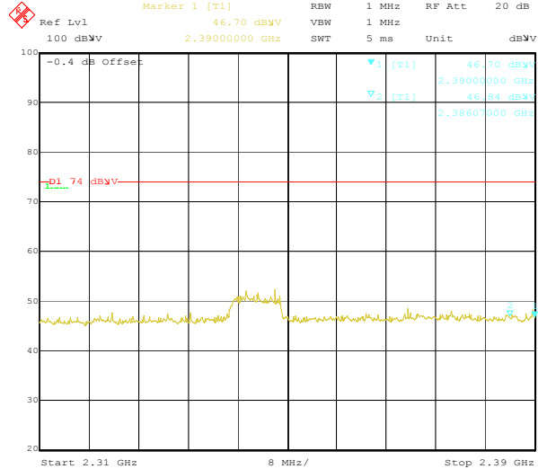
Main-RF Lowest Channel (operating at 2402 MHz): PEAK
