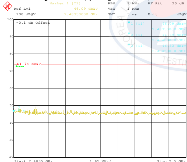
Main-RF Highest Channel (operating at 2480 MHz): PEAK
