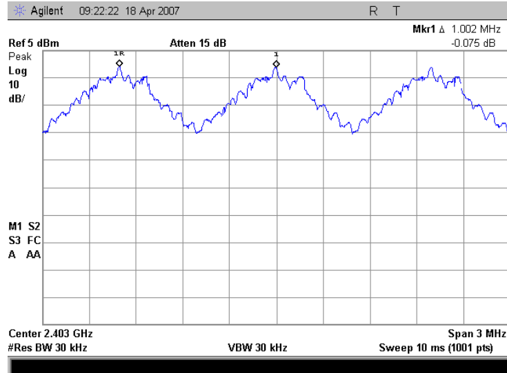
Figure 2: Carrier Frequency Separation (Conducted)
