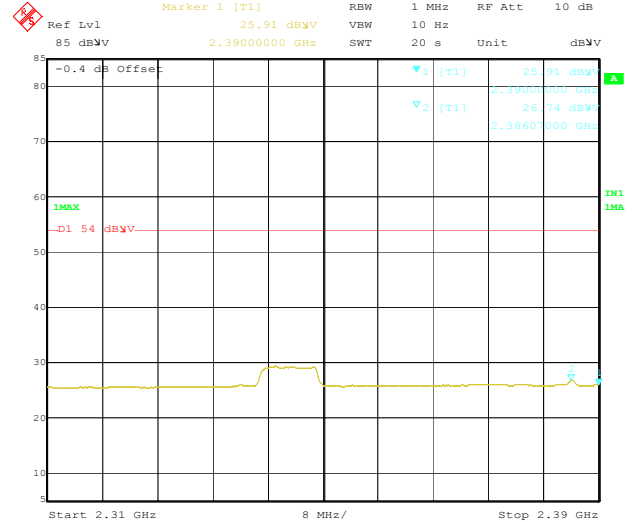
Main-RF Lowest Channel (operating at 2402 MHz): AVERAGE
