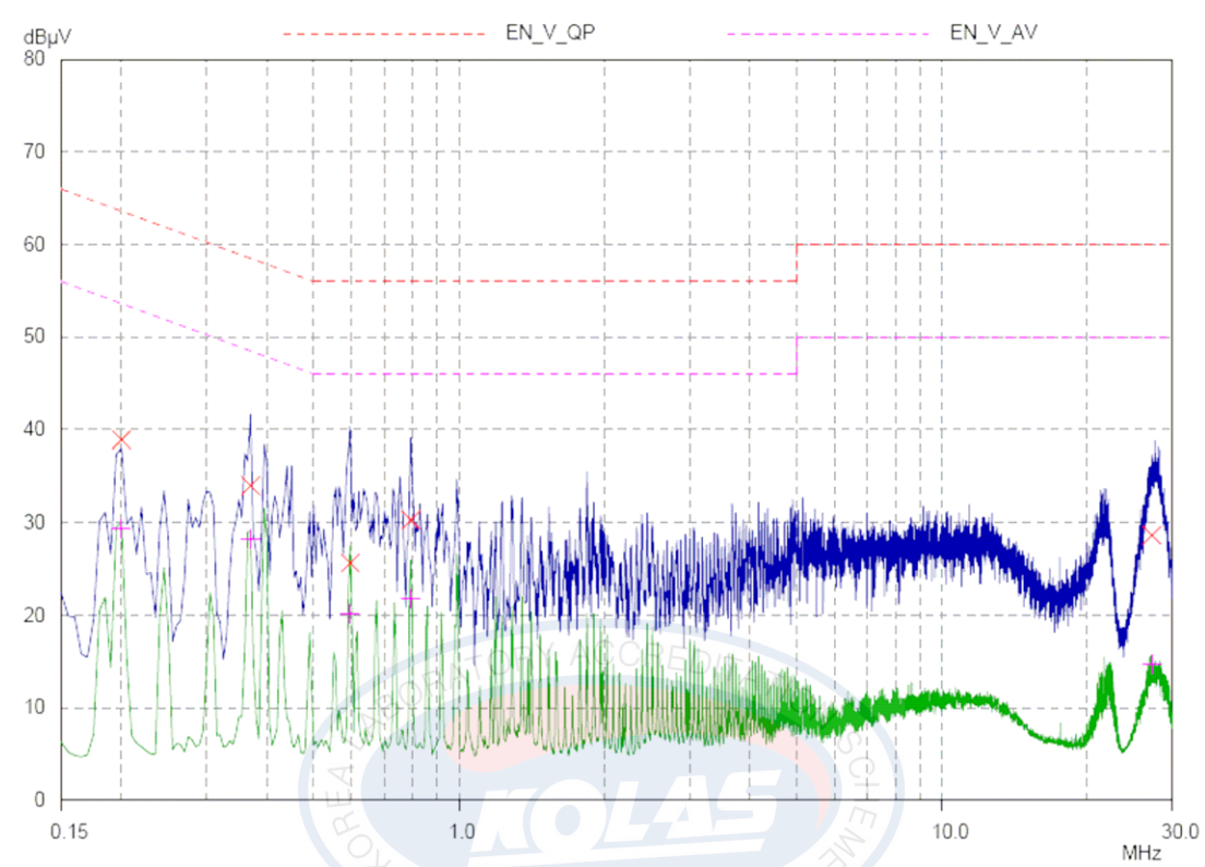
Neutral – PE(Quasi-Peak and Average detector used)
