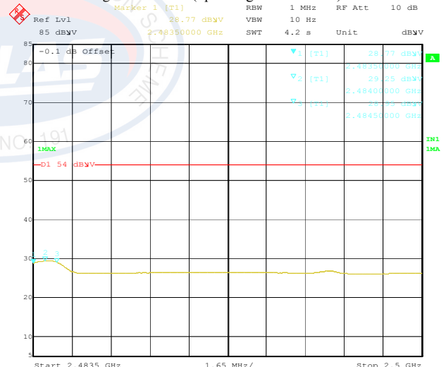
Main-RF Highest Channel (operating at 2480 MHz): AVERAGE
