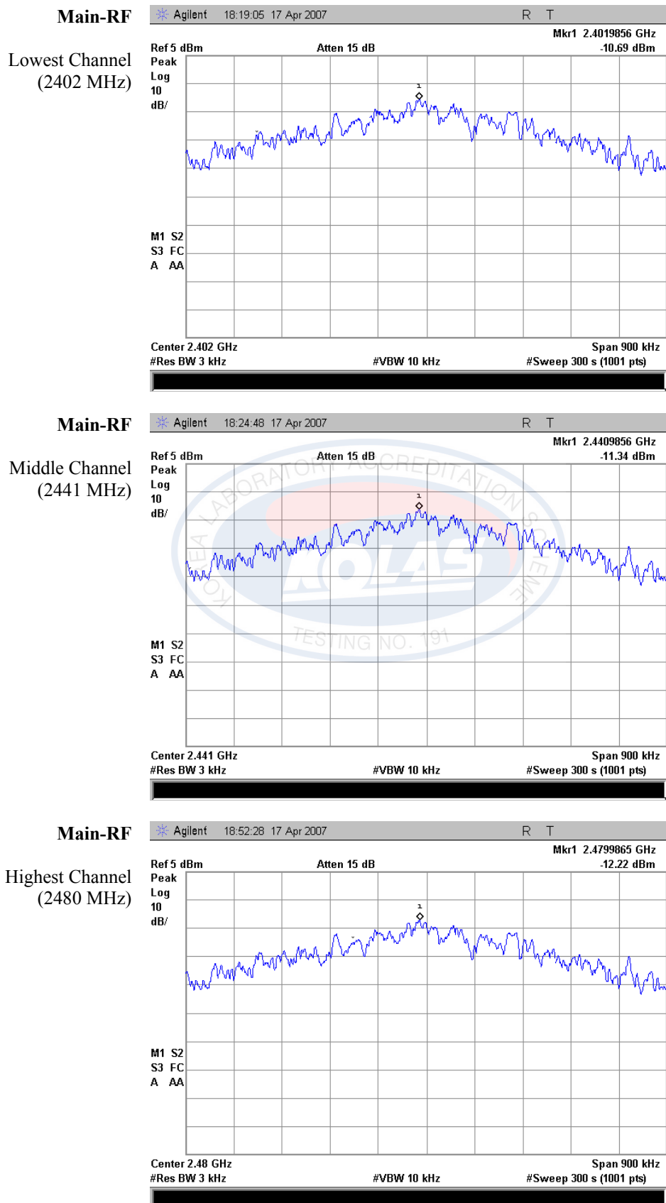
Figure 9: Power Spectral Density (Conducted)
