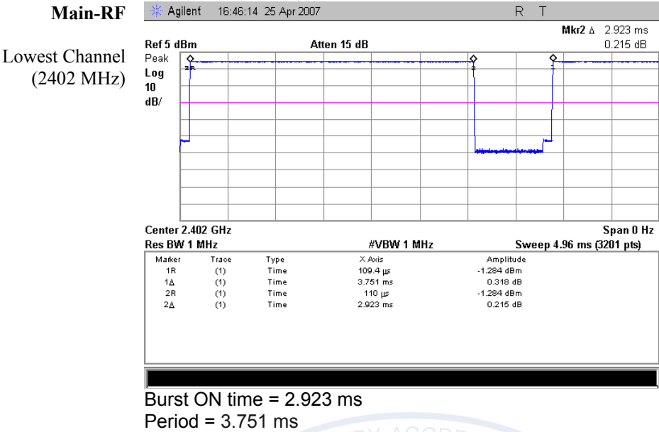
Figure 5: Time of Occupancy (Conducted)
