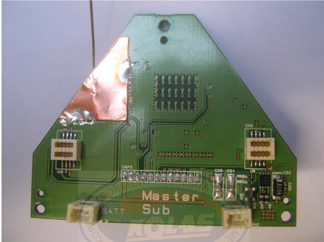
&lt;Photograph 3: Sub RF Board&gt;
