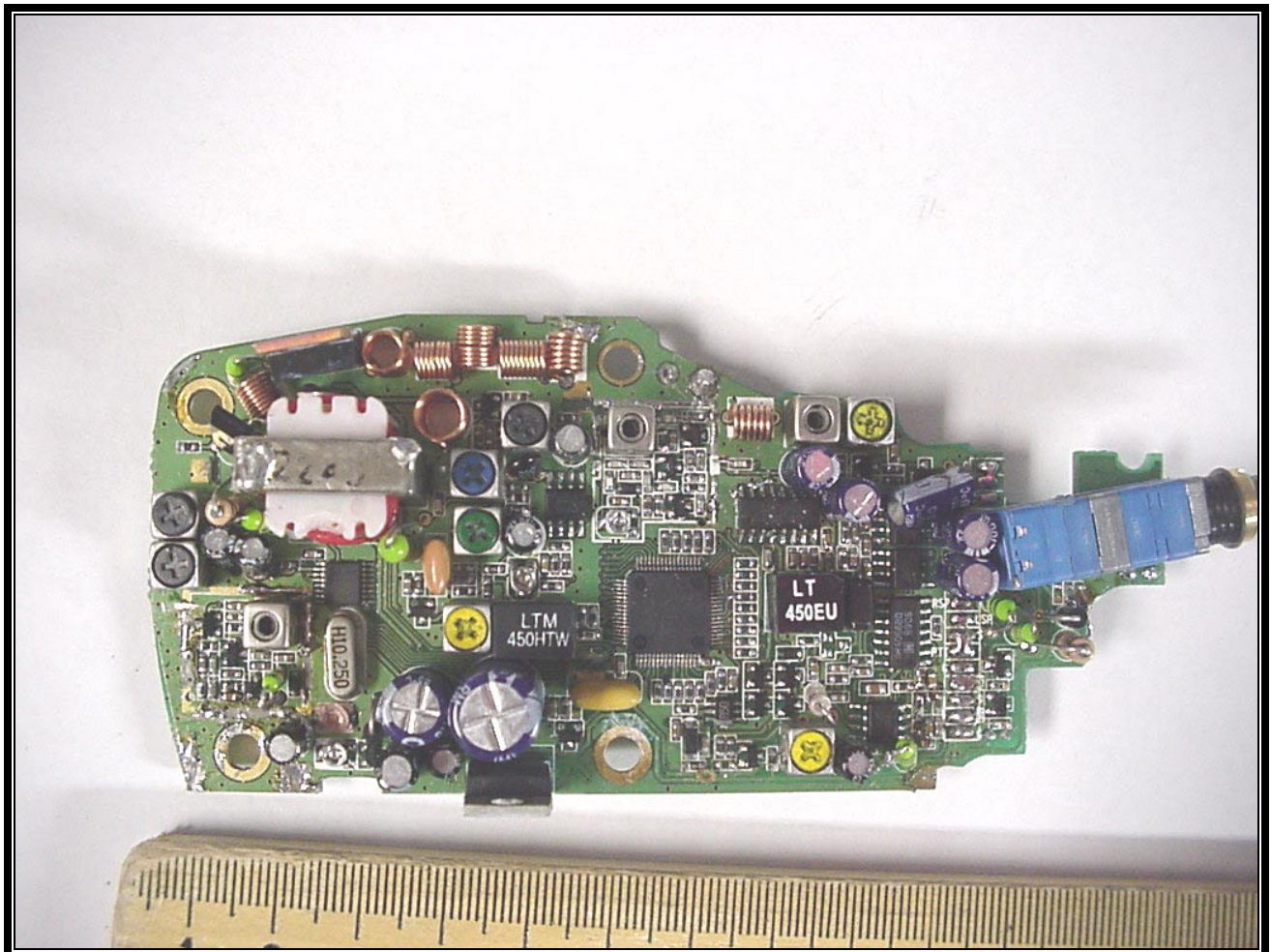
PHOTOGRAPH 18: BACK WITH SHIELD REMOVED
