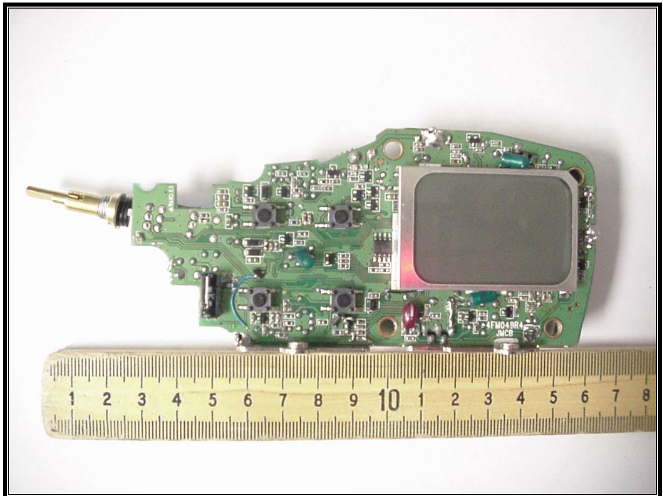
PHOTOGRAPH 19: FRONT OF PCB WITH LCD
