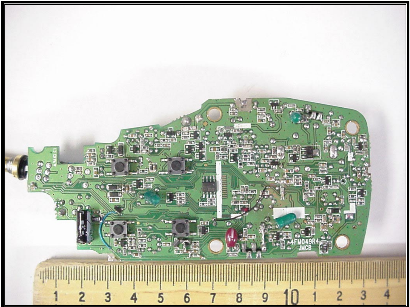
PHOTOGRAPH 20: FRONT OF PCB WITH LCD REMOVED
