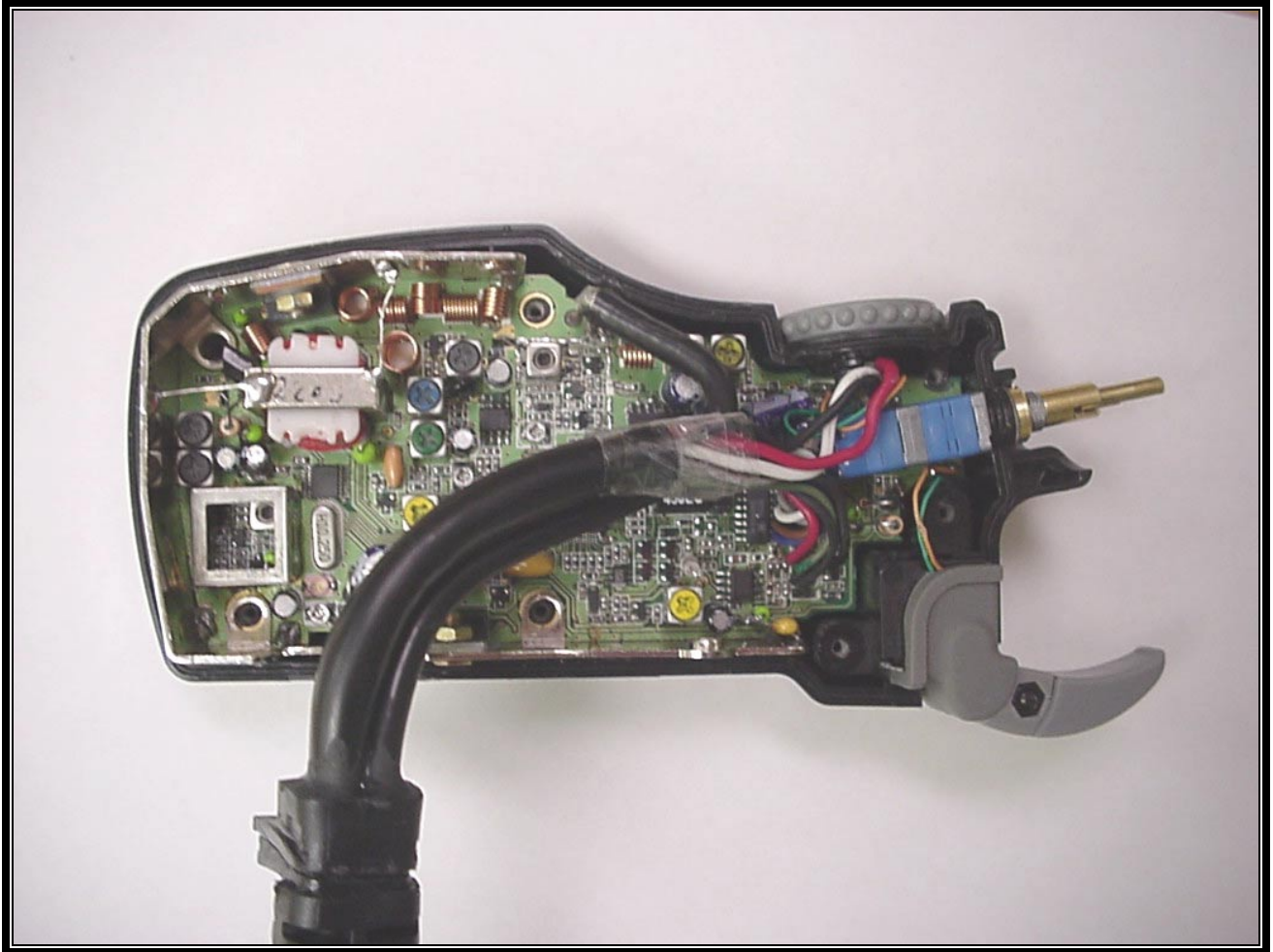
PHOTOGRAPH 13: BACK SIDE WITH CABLES CONNECTED
