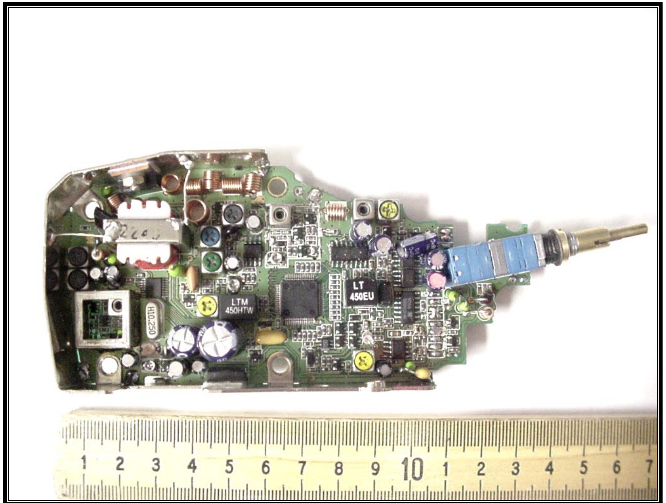
PHOTOGRAPH 17: BACK WITH SHIELDS
