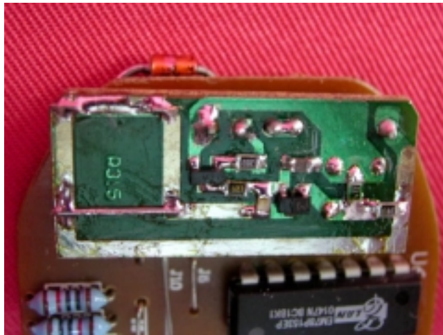
Internal Photo – 4
