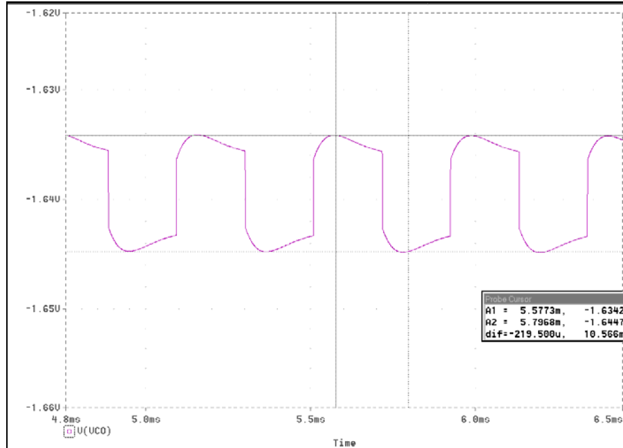
Figure 9.2.2. Plot of VCO V_{\text{tune}} output using single pole compensated modulation .
