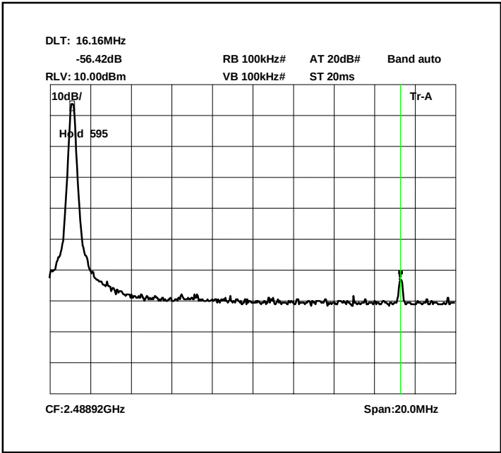
Spurious Emissions Top Channel CW Band-edge
