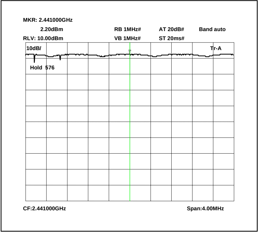
PEAK POWER MID CHANNEL
