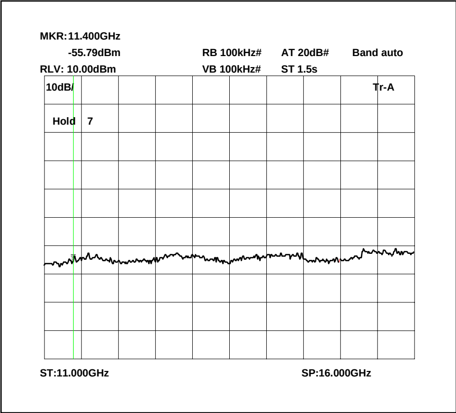
Spurious Emissions Hopping All Channels 11 GHz – 16GHz
