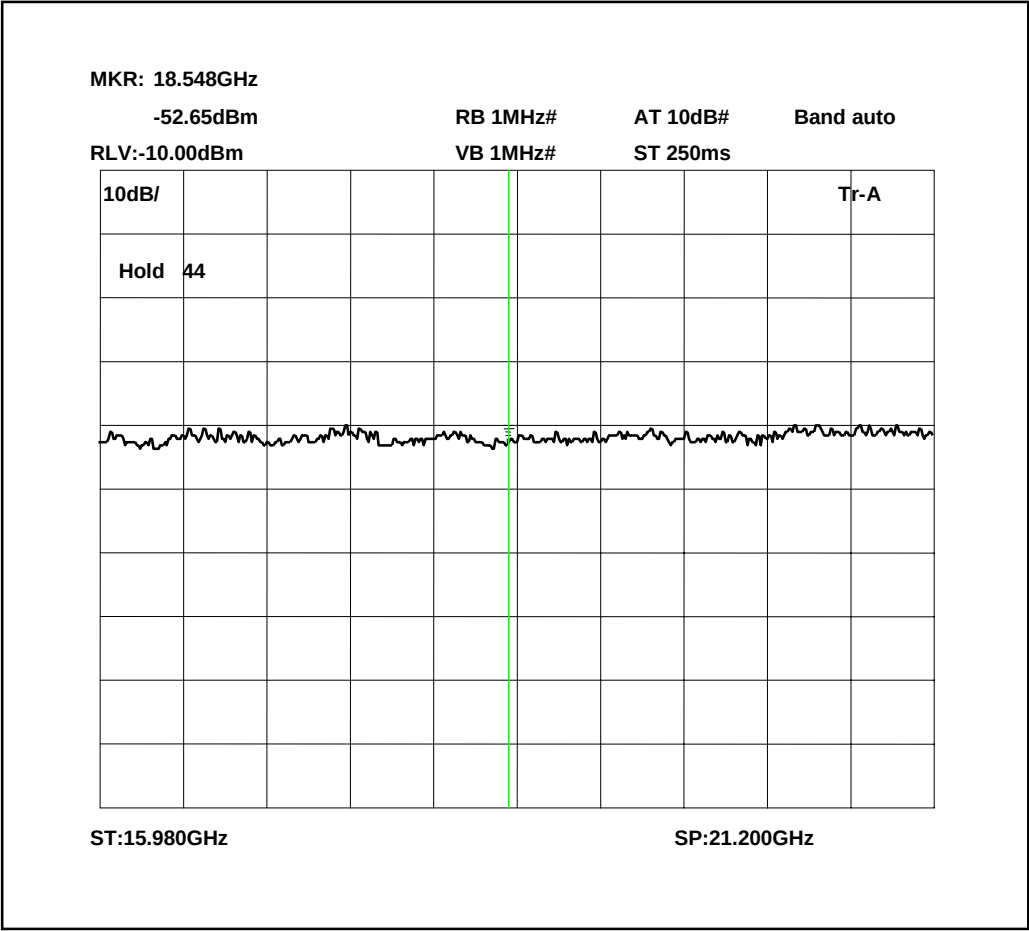
Spurious Emissions Receiver Operating 16GHz – 21.2GHz
