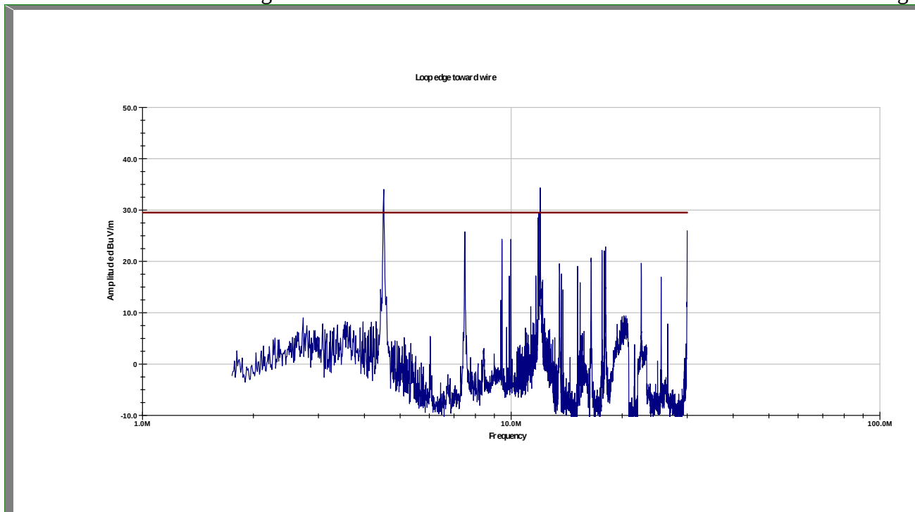
Field Strengths (location 14) 1.705 MHz– 30 MHz
