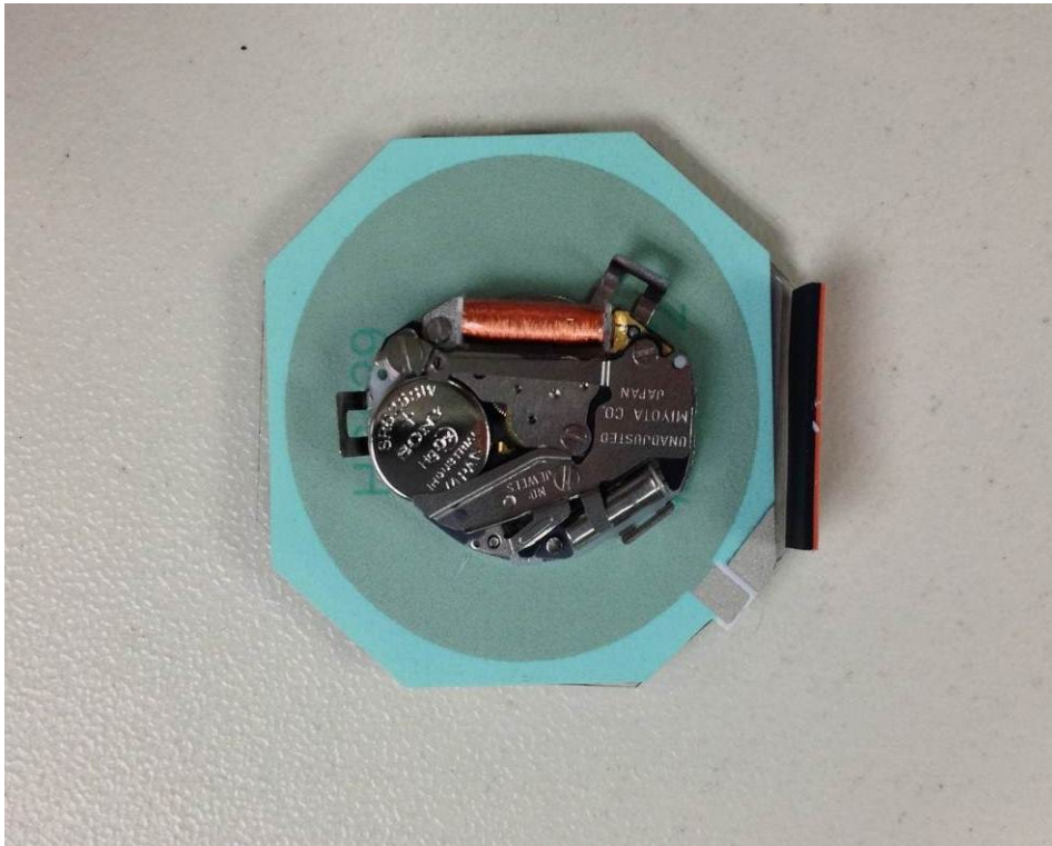
Internal View
