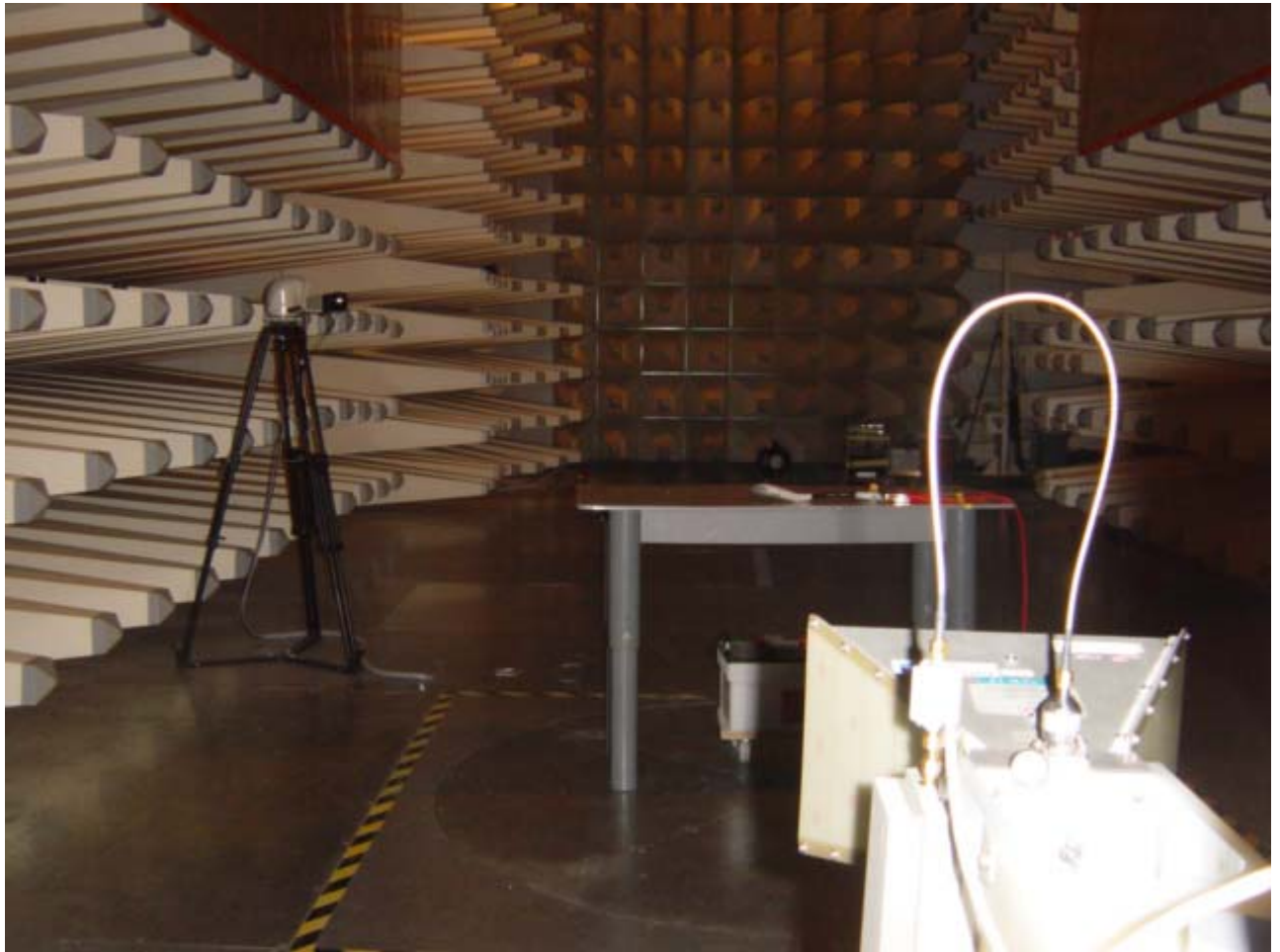
Set-up for Radiation Emission (Transceiver)
