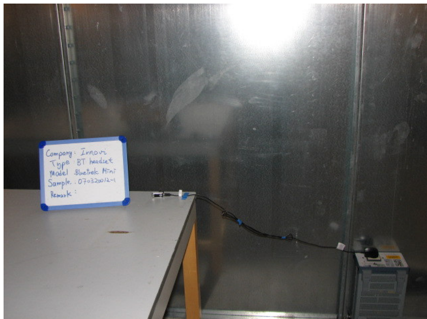
Set-up for Conduct Emission
