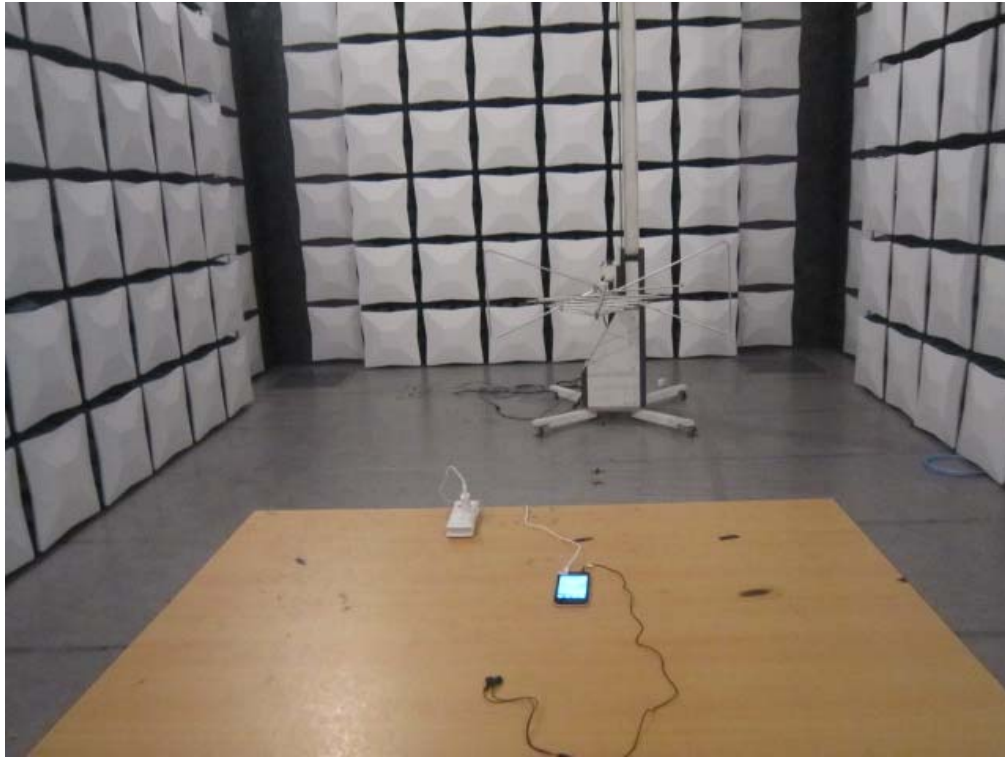
Photo 4 Radiated Disturbance Test (30MHz-1GHz)
