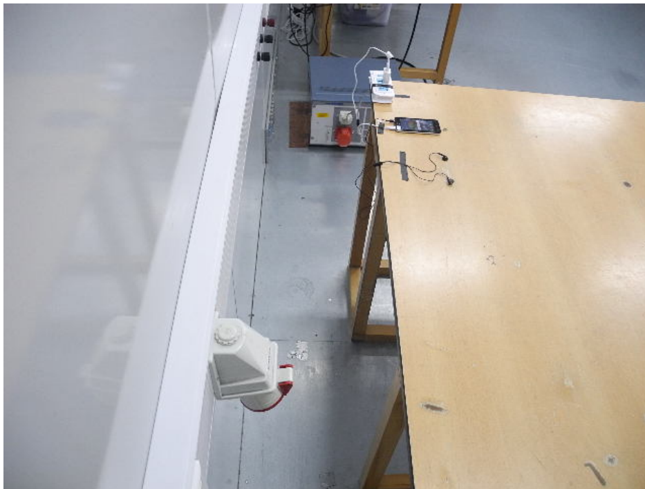
Photo 2 Conducted Disturbance Test
