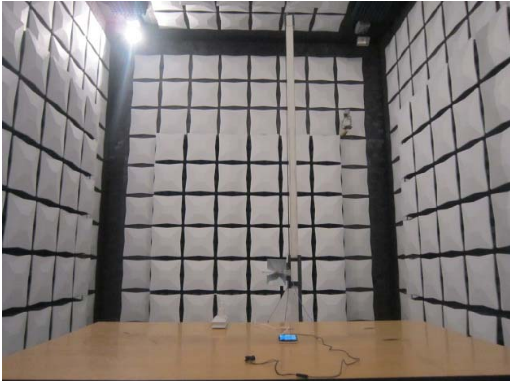
Photo 5 Radiated Disturbance Test (1GHz-6GHz)
