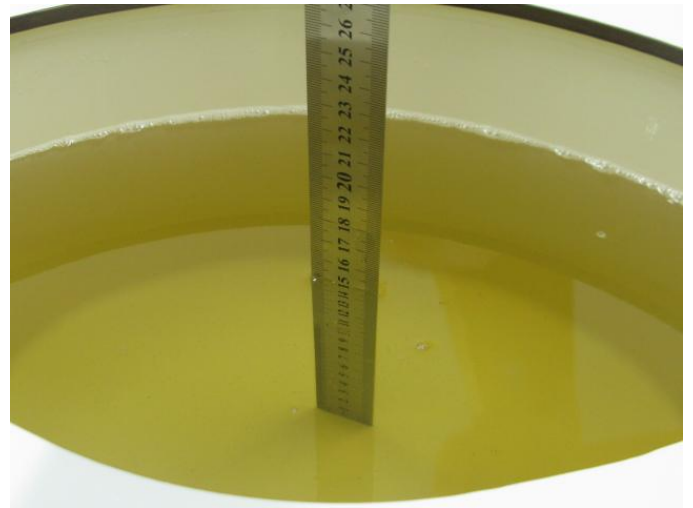
Photo 19:MSL 835MHz depth (15.1cm)
