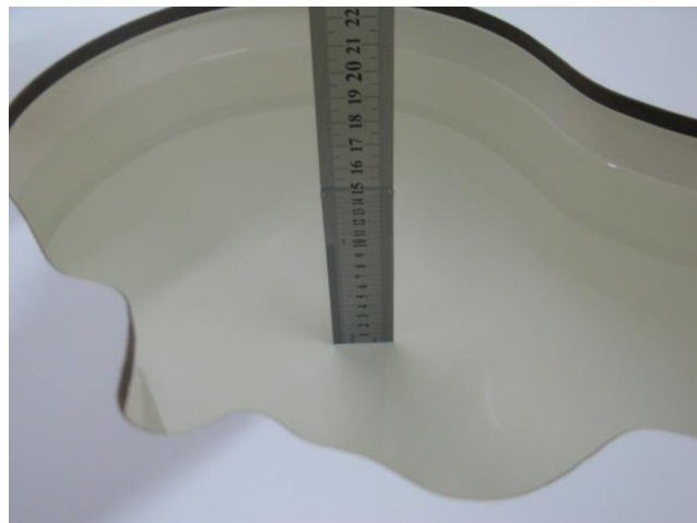
Photo 20:HSL 1800MHz depth (15.3cm)
