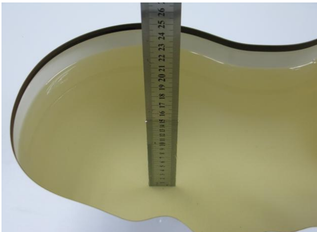
Photo 20:HSL 1800MHz depth (15.3cm)
