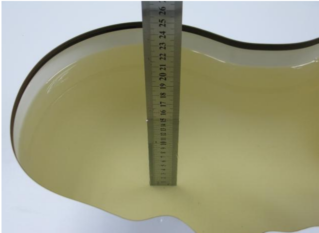
Photo 18:HSL 835MHz depth (15.2cm)
