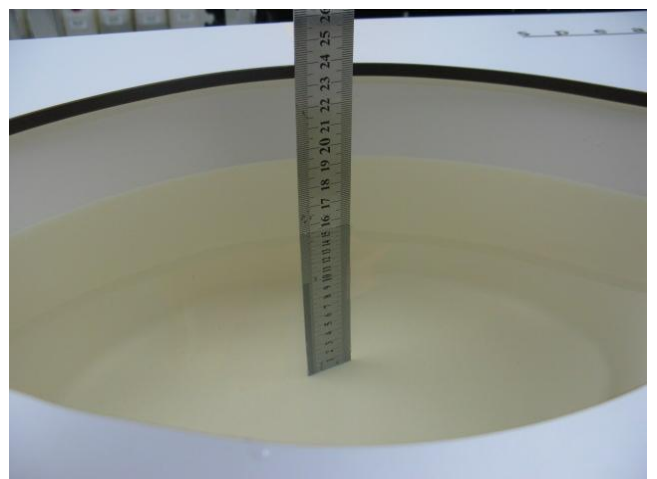
Photo 21:MSL 1800MHz depth (15.1cm)
