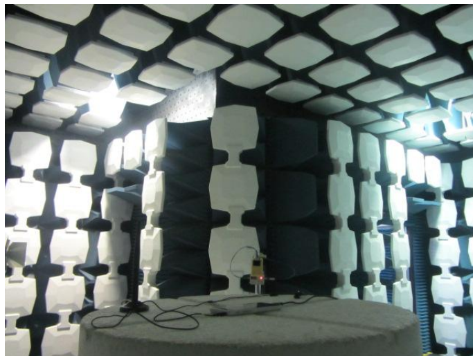
Radiated Spurious Emission (above 18GHz)
