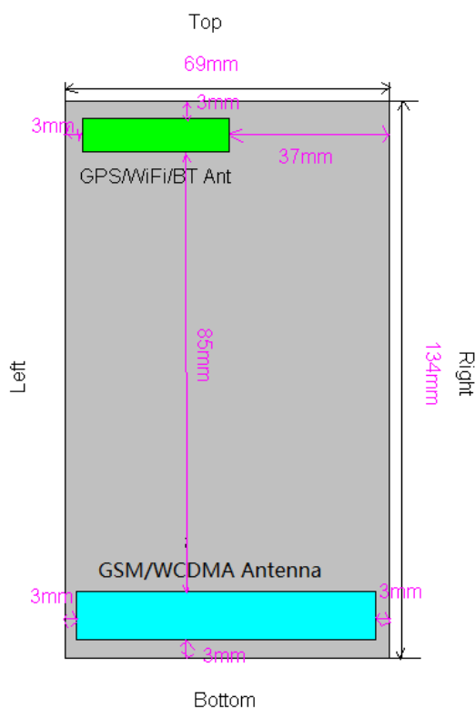
Mobile Hotspot Sides for SAR Testing
