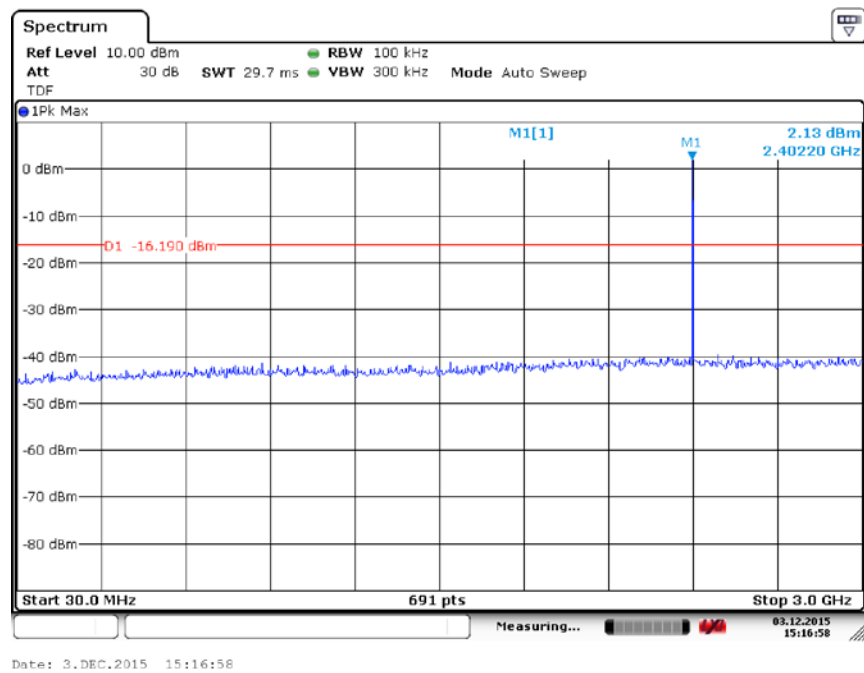
Fig. 40 Conducted Spurious Emission (8DPSK, Ch0, 2.402GHz)
