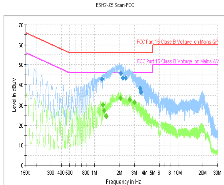
Fig. 98 AC Power line Conducted Emission (Idle, AE1)
