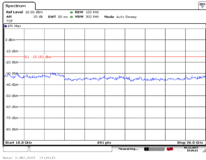
Fig. 49 Conducted Spurious Emission (All channel, 18 GHz-26 GHz)
