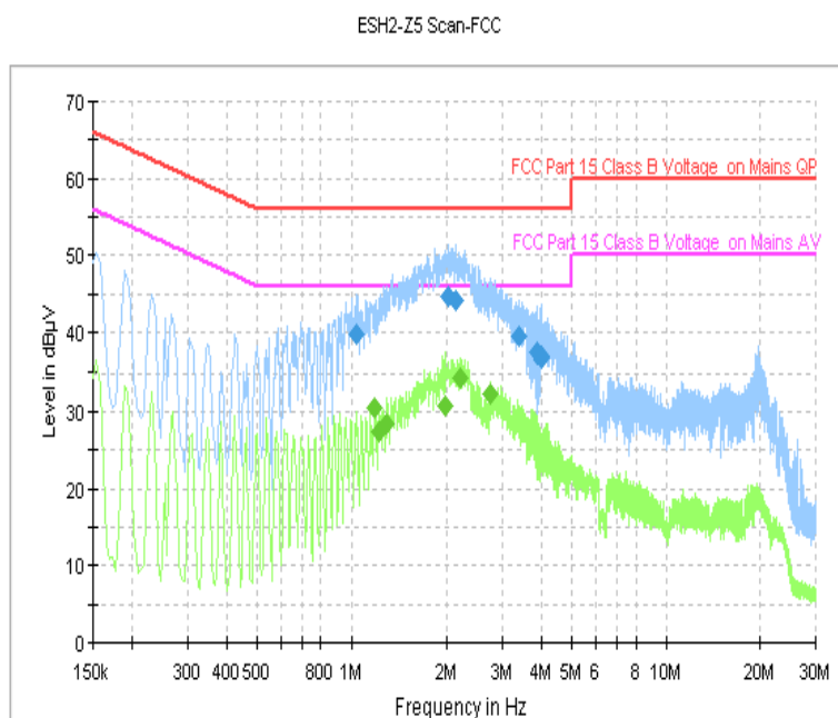
Fig. 32 AC Power line Conducted Emission (Idle, AE1)
