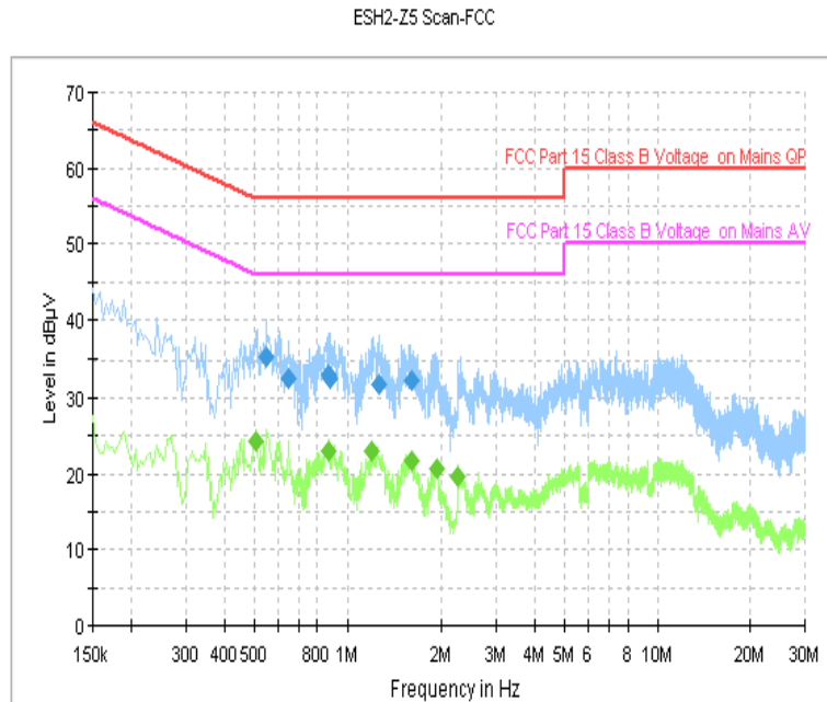
Fig. 33 AC Power line Conducted Emission (Idle, AE2)
