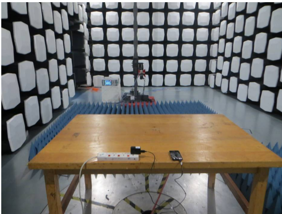
4. Radiated Emissions (Part 15B Charging mode) (Above 1GHz)
