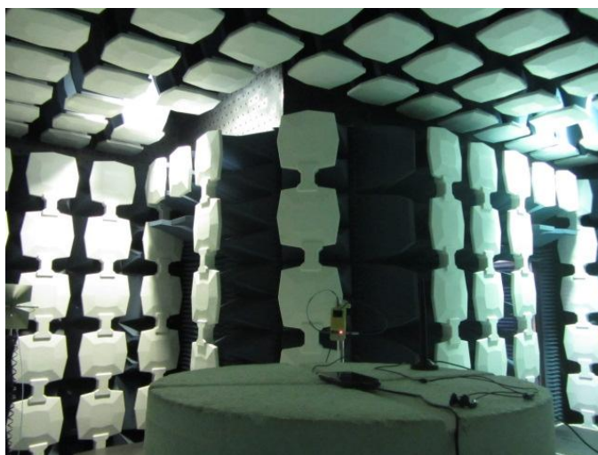
Radiated Spurious Emission (18GHz to 26.5GHz)
